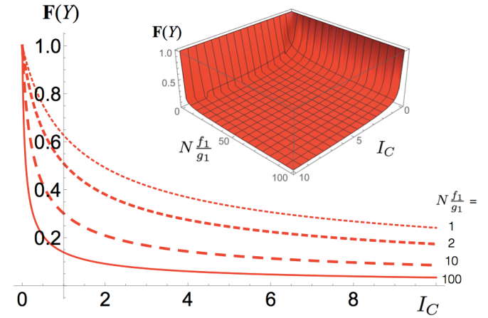
Fig. 4. Fano factor of the trimer F(Y) as a function of the cooperativity index I_C for different values of N \frac{f_1}{g_1} (2D graph), and as a function of I_C and N \frac{f_1}{g_1} (3D graph); N is taken equal to 500.
