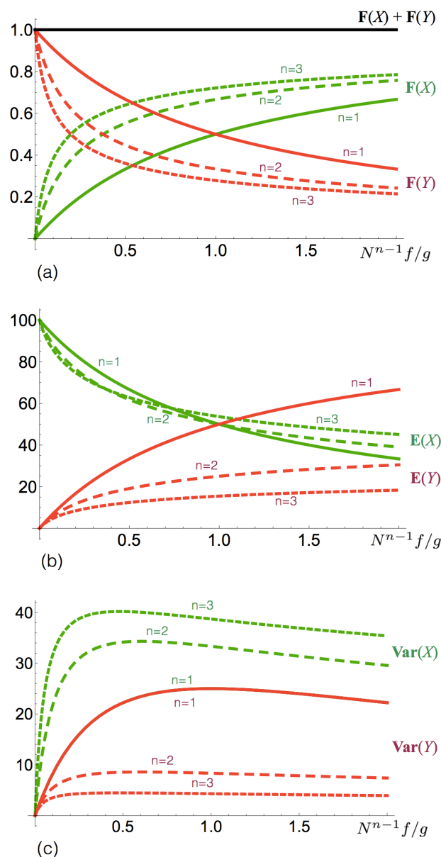
Fig. 2. Stochastic behavior of homo-oligomerization processes, as a function of the interconversion parameter \frac{f}{g} N^{n-1} , for oligomers of degree n = 1 to 3. N is taken equal to 100. (a) Fano factors; (b) Mean values; (c) Variances.
