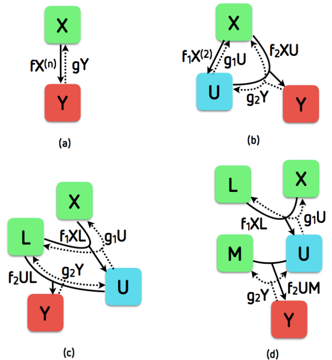
Fig. 1. Schematic representation of the oligomerization systems studied in this paper. The green boxes correspond to monomers ( X , L , M ), the red boxes to oligomeric products ( Y ), and the blue boxes to intermediate states ( U ).
