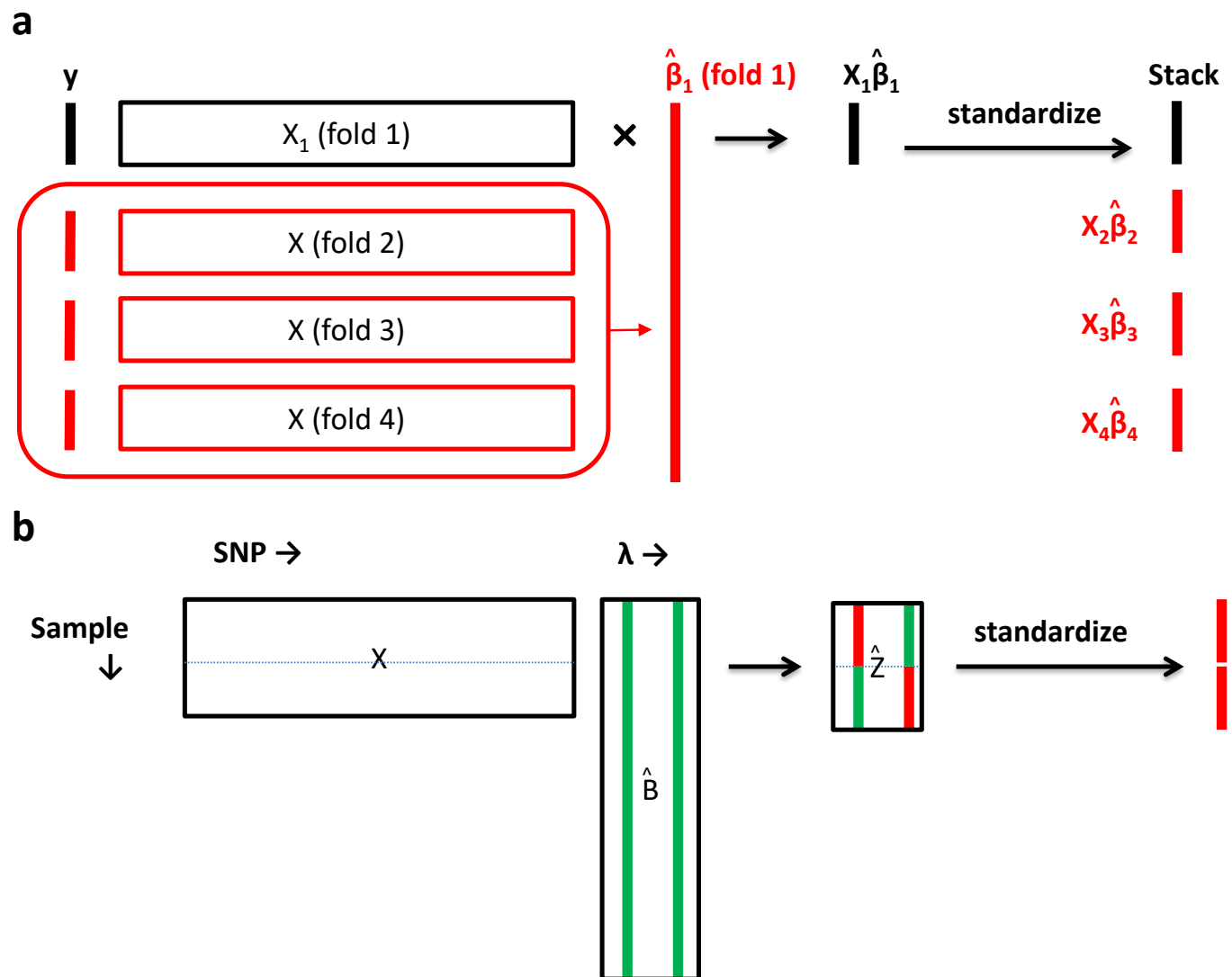
Figure 3: (a) Cross-prediction. The data (\mathbf{X}, \mathbf{y}) is split into 4 folds. For fold 1, the coefficients \hat{\beta}_1 is estimated from folds 2,3, and 4. The estimated PGS \mathbf{X}_1\hat{\beta}_1 is standardized and stacked together to form the final PGS. (b) Split-validation. Let \mathbf{X} denote the genotype matrix, \hat{\mathbf{B}} the matrix of coefficients, and \lambda indices the p -value threshold. Let \hat{\mathbf{Z}} = \mathbf{X}_k\hat{\mathbf{B}}_{-k} be the matrix of PGS calculated for the k^{\text{th}} fold. \hat{\mathbf{Z}} and \mathbf{X}_k are split into two halves. The green columns are the columns of \hat{\mathbf{B}} corresponding to the p -value threshold selected by validation. The red columns are the corresponding \hat{\mathbf{Z}} taken to form the PGS.
