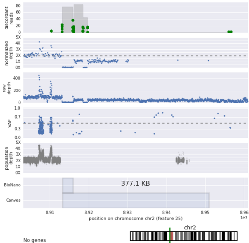
Supplemental Note Figure 2: This CNV is a homozygous deletion followed by a mosaic loss leading up to the centromere of chromosome 2. The homozygous deletion is called by BioNano, but the mosaic loss is missed or filtered.
