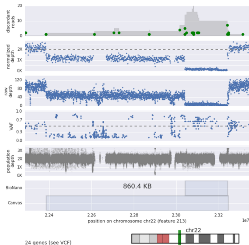
Supplemental Note Figure 1. This is a homozygous deletion flanking a mosaic 22q11 deletion, a likely cell line artifact. Our WGS pipeline called this event as a single CNV, whereas the BioNano/PacBio caller only called the homozygous deletion.
