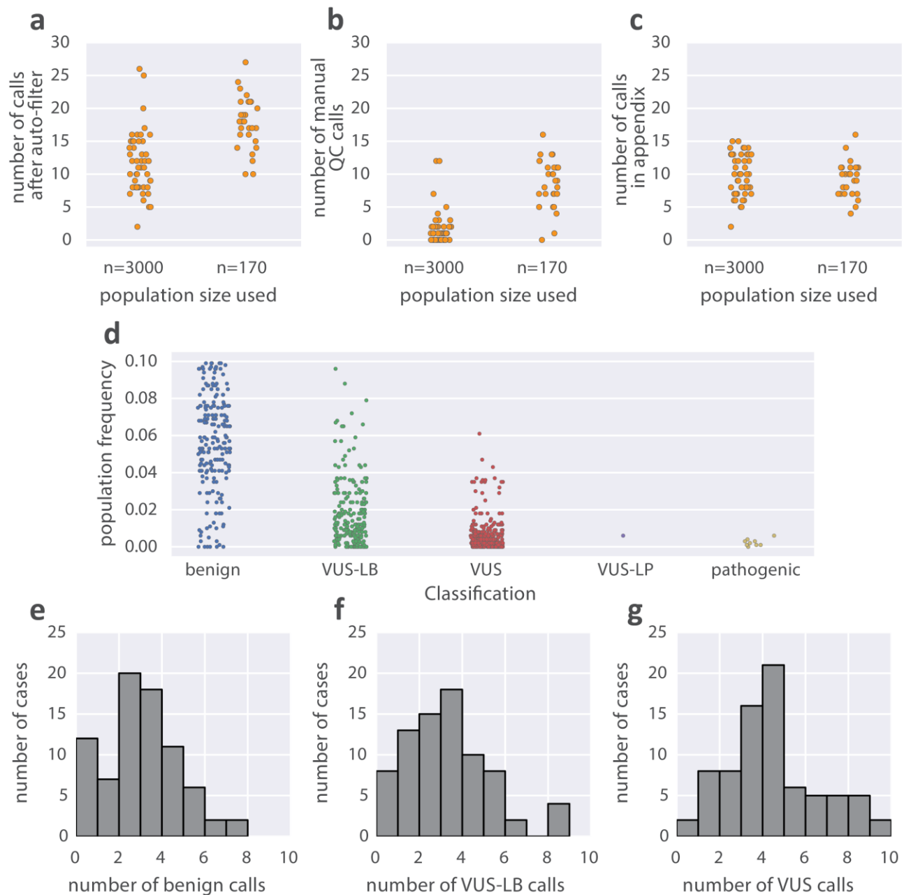
Figure S2. Summary of manual curation and variant annotation across the CNV clinical case cohort. (a-c) Number of calls passing automated filters (a) , manually filtered (b) and included in a CNV appendix to clinical reports (c) broken down by the two populations used for CNV frequency annotation (n=170 was used for the first 28, and n=3000 was used for the remainder). (d) Copy number variant population frequency broken down by variant classification post curation. (e-g) Breakdown of variant classifications for CNVs included in clinical report appendix across the cohort. In addition there were calls reported as pathogenic in 7 cases, and one likely-pathogenic call reported. VUS - variant of unknown significance; VUS-LB- variant of unknown significance, likely benign.
