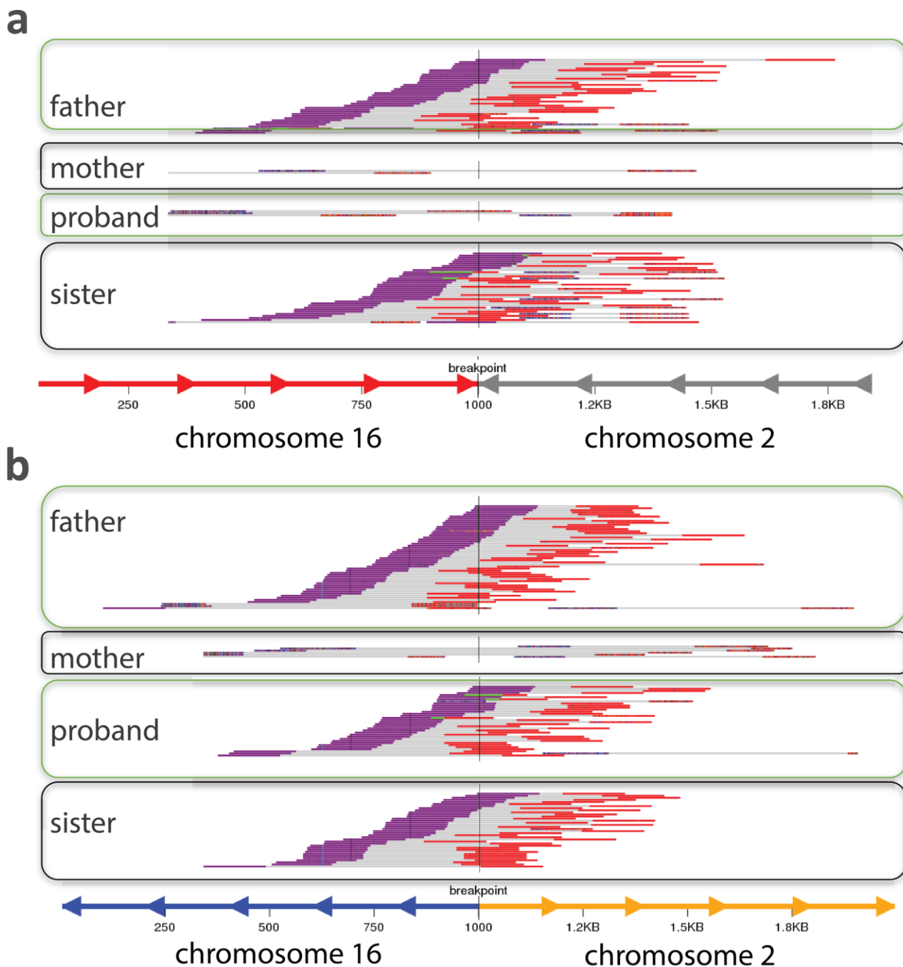
Figure S5. Read support for unbalanced translocation in subject P7. Shown here are modified plots from the svviz graph realignment program. In brief reads are realigned to normal (not shown) and recombinant (shown here) chromosomes across the pedigree. Purple and red colors represent the first and second reads in the read-pair, respectively, for details on the visualization and realignment methods see (Spies et al., 2015). See also Figure 2 .
