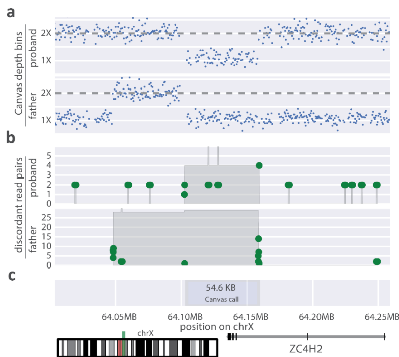
Figure 1. ZC4H2 de-novo deletion in case P1 . a) Normalized sequencing depth for proband and her father. b) Location of discordant read pairs (>1000bp insert size), where green dots represent the location of paired ends in a discordant read-pair, the grey shaded area represents the total number of discordant read-pairs spanning a given genomic segments. c) Annotation of the original Canvas call boundaries as well as the location of the CNV on chromosome X.
