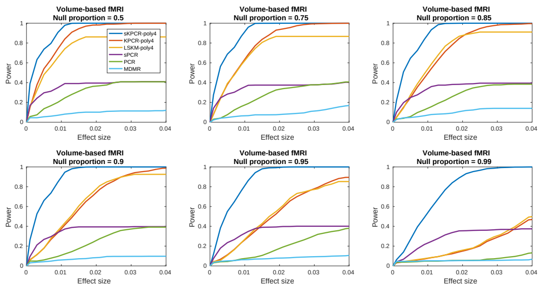
Figure 5: Comparisons of the power of detecting nonlinear signals with different methods using simulations relating to volume-based fMRI data . The simulated nonlinear signal is a four-degree polynomial \gamma y^4 + 0.5y^2 + 1 . Each figure plots the power curves for 6 different methods under different signal effect sizes ( \gamma = 0.001 \sim 0.04 ) with certain null signal proportions (0.5~0.99).
