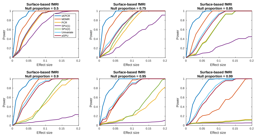
Figure 4: Comparisons of the power of detecting linear signals with different methods using simulations relating to surface-based fMRI data. Each figure plots the power curves of 7 different methods under different signal effect sizes (between group mean difference = 0.01~0.2) with certain null signal proportions (0.5~0.99).
