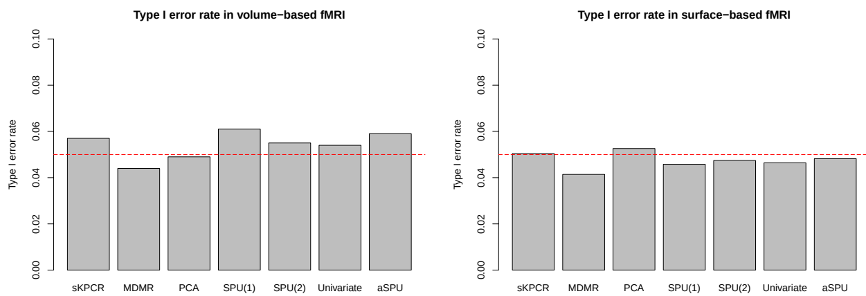
Figure 2: Type I error rate of different methods estimated in volume-based and surface-based fMRI data.
