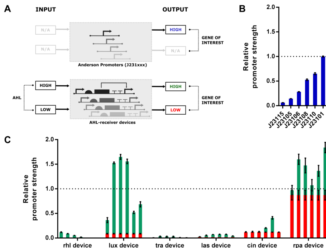
Figure 3: Relative promoter strengths of AHL-receiver devices. (A) Schematic of possible states of characterised genetic devices. Constitutive promoters of the Anderson promoter library exhibit just one output state of high signal in the absence of any input signal. Conversely, the AHL-receiver devices can operate in two states: at low input they exhibit a low output; while at high input they exhibit high output. (B) Bar chart of relative promoter strength of constitutive Anderson promoters and (C) inducible AHL-receiver devices. The dotted line indicates promoter strength of the reference standard promoter Bba_J23101. The chart is color-coded according to the states of the devices as indicated in the schematic in (A). Error bars indicate the standard error of the mean of three biological repeats.
