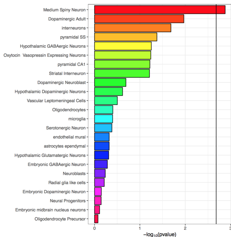
Figure 4. Association between mouse brain cell-type specific expression and gene-level genetic association to AN/OCD using MAGMA. The black vertical bar represents the Bonferroni significant threshold.
