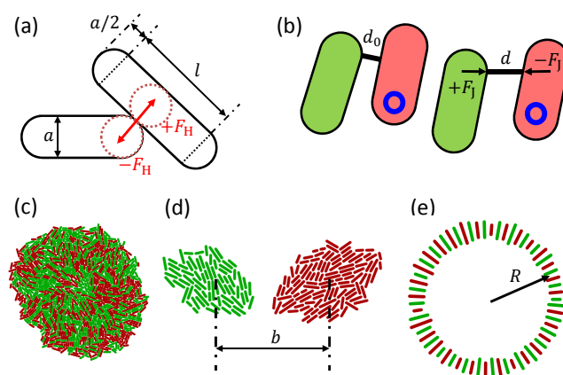
FIG. 1: The computer model. (a) Cells are modelled as spherocylinders of length l and diameter a , interacting through Hertzian repulsive forces F_H . (b) Conjugative junction in Models 2 and 3 is an elastic spring of rest length d_0 and spring constant k . The spring creates a restoring force F_J when the distance d between the conjugating cells (donor = red cell with a blue circle representing the plasmid, recipient = green cell) is different to d_0 . (c) A snapshot of an exponentially growing colony with a 1:1 mixture donors:acceptors. (d) Colliding colonies. b is the distance between the two cells that initiated the colonies. (e) Initial configuration of cells in the linearly-expanding colony simulation.
