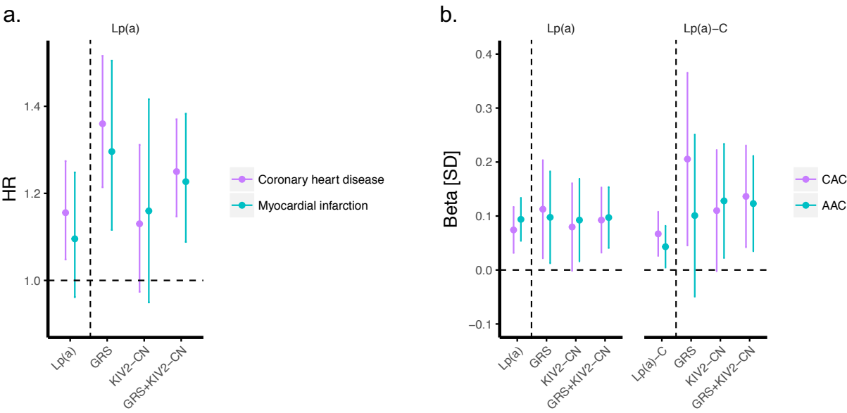
Fig 7. Association of LPA variant classes with incident cardiovascular events and subclinical measures.
