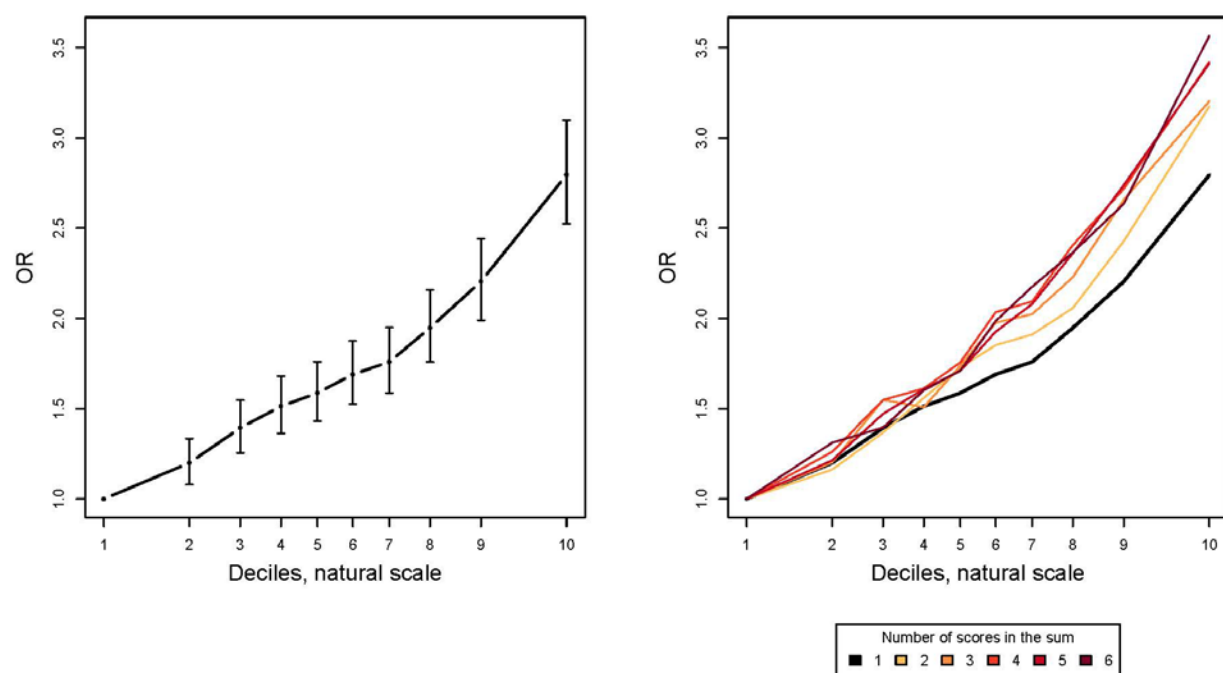
Figure 4. Decile plots
