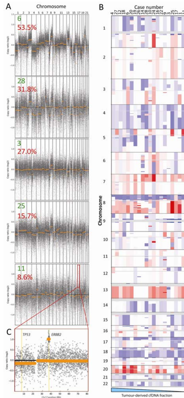
Figure 4 (A) Genome wide copy number aberrations can be detected from targeted cfDNA sequencing, even where tumour content is low. Representative log copy ratio plots for five cases (green number) in our cohort with tumour content ranging from 53.5% to 8.6% (red number indicates max VAF) are shown. (B) Genome wide heatmap of segmented copy number raw log ratio data after amplitude normalization. Gains are red and losses are blue. Profiles are ordered (left to right) from highest to lowest tumour content (based on maximum VAF) for all 20 cases that had a visible CNA profile. (C) Focused log copy ratio plot of chromosome 17 for case 11 which had a high level amplification of ERBB2 .
