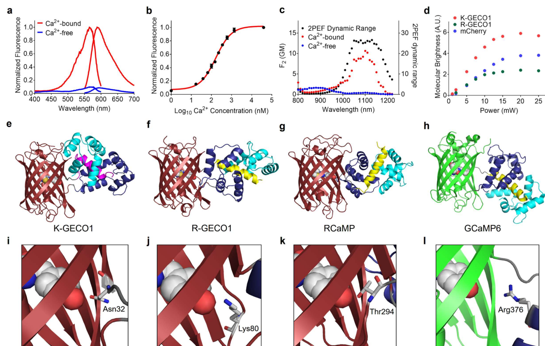
Figure 2. Characterization and structure of K-GECO1. (a) Fluorescence excitation and emission profile of K-GECO1 in the presence and absence of \text{Ca}^{2+} . (b) \text{Ca}^{2+} titration curve of K-GECO1. (c) K-GECO1 effective two-photon fluorescence excitation spectra in \text{Ca}^{2+} -saturated (red symbols) and \text{Ca}^{2+} -free (blue symbols) states. Ratio of the K-GECO1 two-photon excitation fluorescence \text{Ca}^{2+} -saturated/ \text{Ca}^{2+} -free signals as a function of wavelength (black symbols, plotted on right y-axis). (d) Two-photon molecular brightness of K-GECO1, R-GECO1 and mCherry with excitation at 1060 nm using various laser power. Overall protein structures of GECIs (e-g), K-GECO1 (PDB: 5UKG) (e), R-GECO1 (PDB: 4I2Y 19 ) (f), RCaMP (PDB: 3U0K 19 ) (g), and GCaMP6 (PDB: 3WLD 60 ) (h), with ckkap colored in magenta, RS20 in yellow, CaM N-lobe in dark blue, and CaM C-lobe in cyan. Zoom-in view of the interactions between key residues and the chromophore (i-l), K-GECO1 (i), R-GECO1 (j), RCaMP (k), and GCaMP6 (l).
