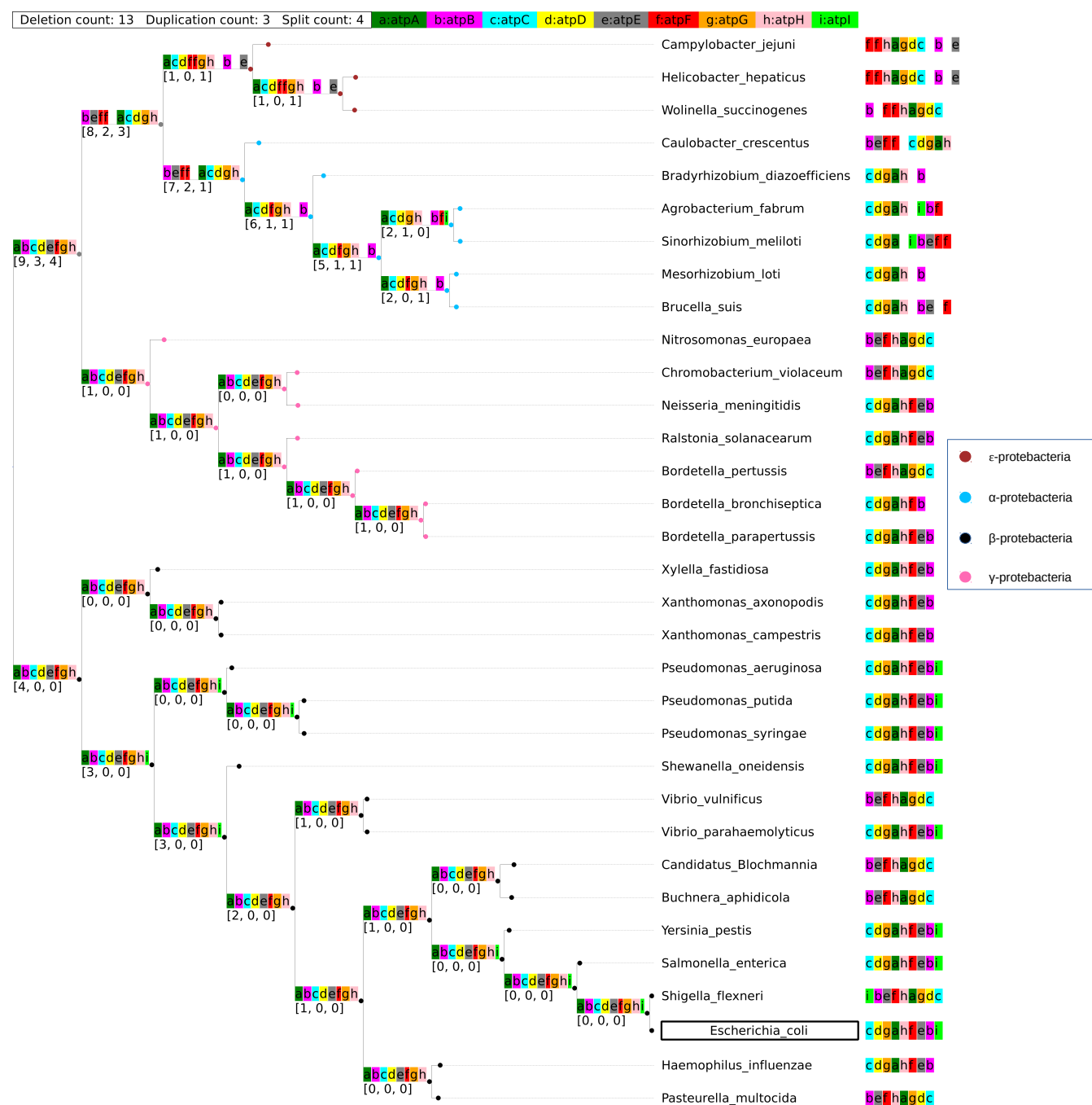
Fig 5. Ancestral reconstruction of operon atpIBEFHAGDC using the global optimization approach.
