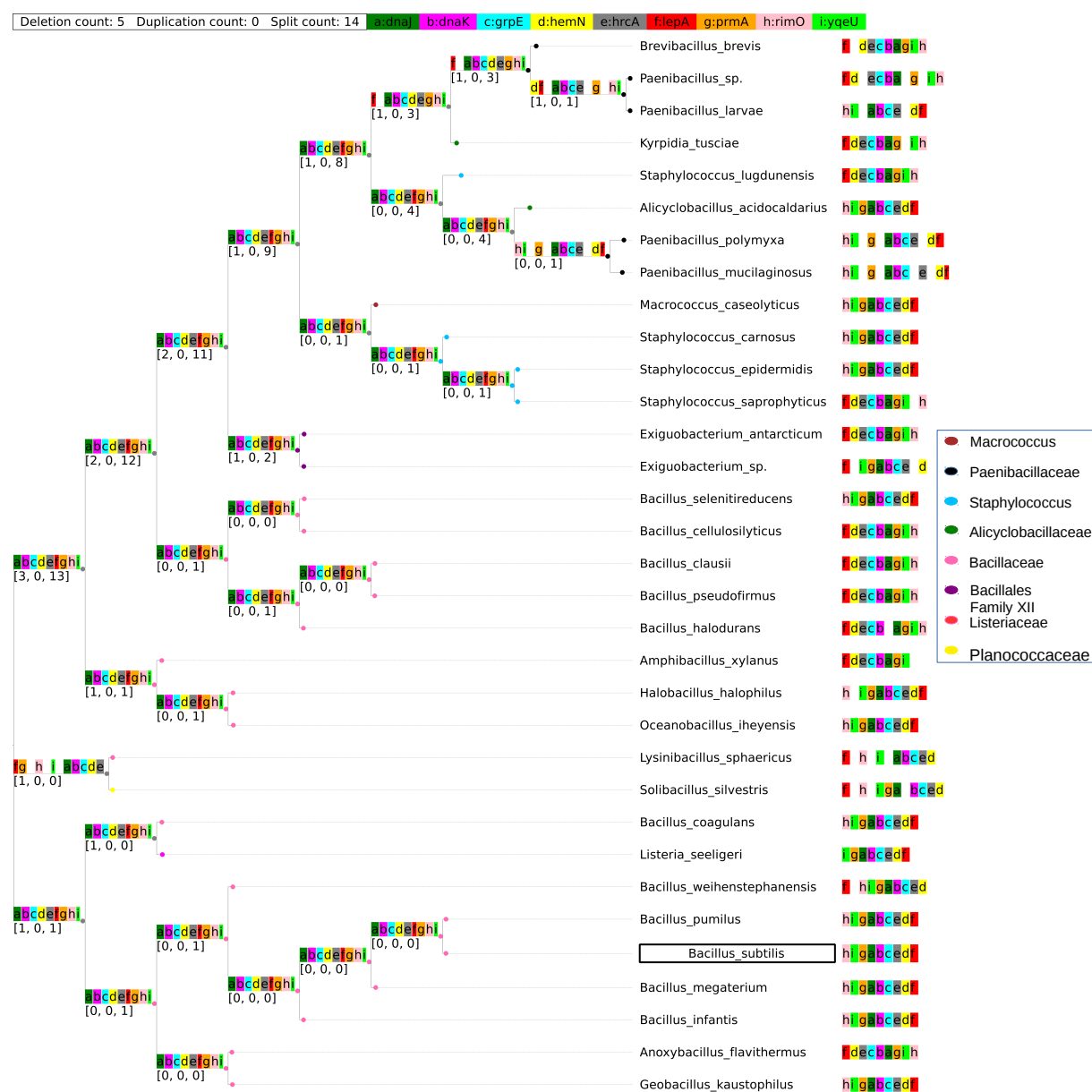
Fig 7. Ancestral reconstruction of lepA-hemN-hrcA-grpE-dnaK-dnaJ-prmA-ygqU-rimO .
