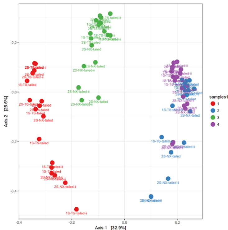
Fig. 3: Principal coordinate analysis (PCoA) plot
