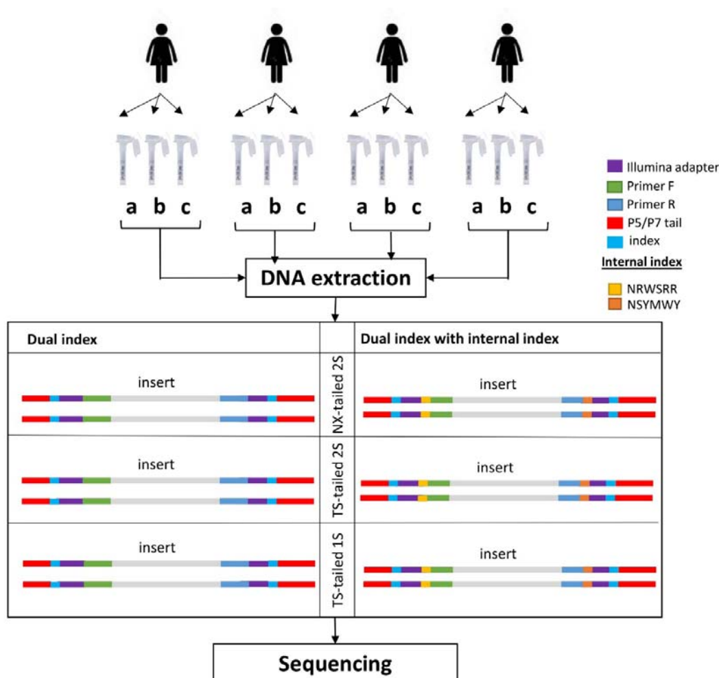
Fig. 1. Study Design
