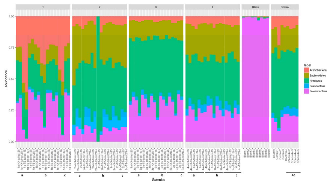
Fig. 5: Phylum abundance
