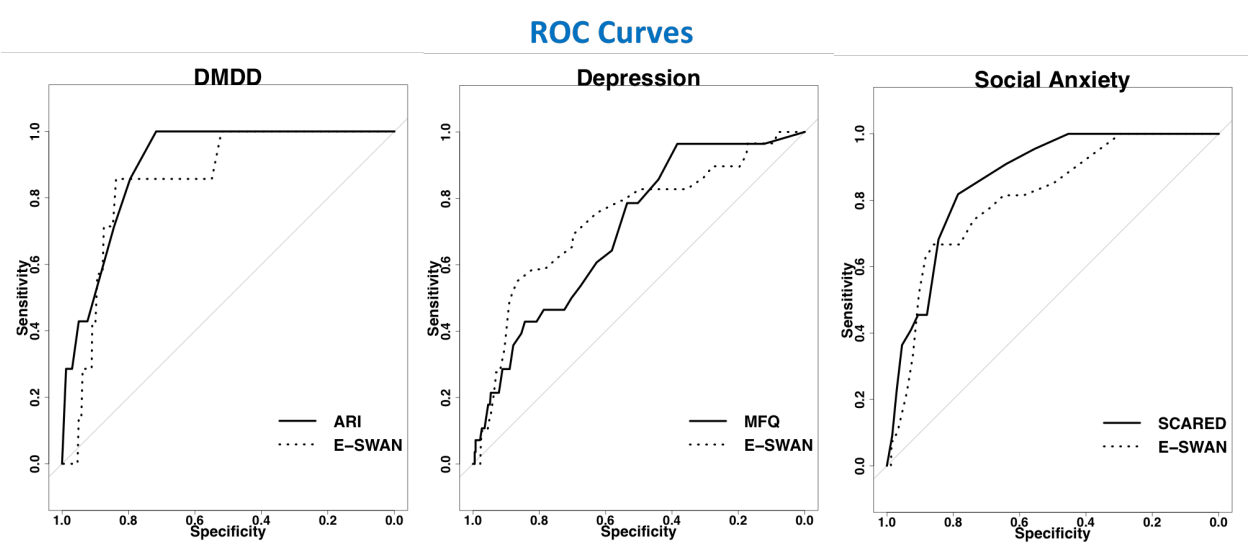
Figure 4. ROC Curves.
