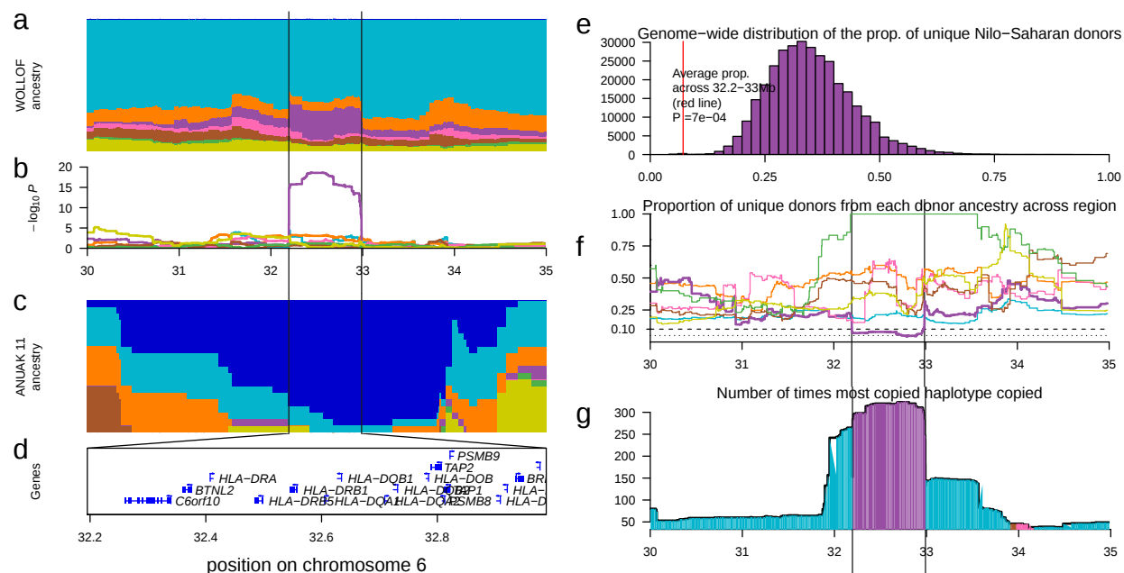
Figure 4: Investigating local ancestry at the HLA in the Wolof. a local ancestry across 2160 Wolof haplotypes at the 30-35Mb region of chromosome 6. b results of the binomial ancestry deviation test shows a significant increase in Nilo-Saharan (purple) ancestry between 32.2 and 33Mb. c ancestry proportions from a local painting analysis in a single Anuak individual showing Western African (dark blue) ancestry. d UCSC genes across this region. e genome-wide distribution of unique Nilo-Saharan donors in the Wolof. f the proportion of unique donors when each of 7 non-self ancestries are copied across the 30-35Mb region of chromosome 6. g the number of times the most common haplotype is copied; the colour under the line represents the ancestry of the most copied individual.
