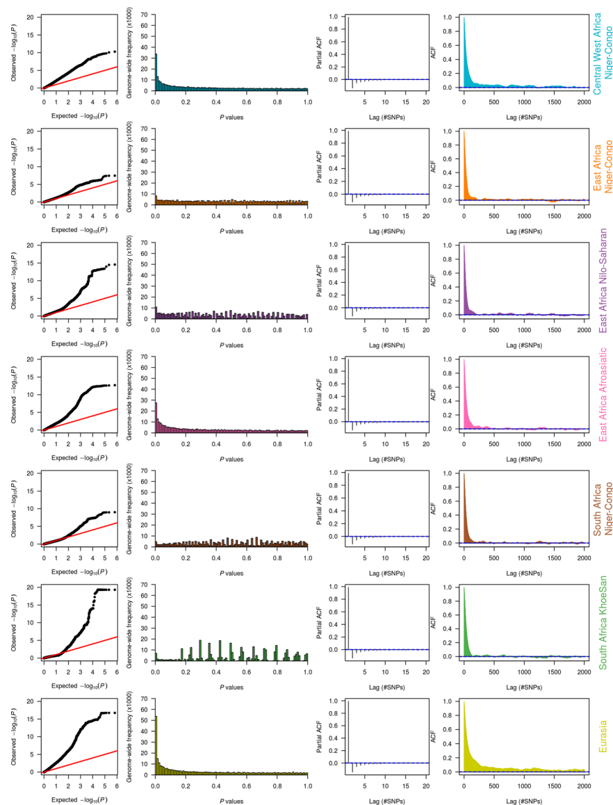
Figure S2: Quantile-Quantile plots of the model statistics in the Fula show inflation. We show QQ plots for P values generated by the binomial likelihood model for each ancestry separately.
