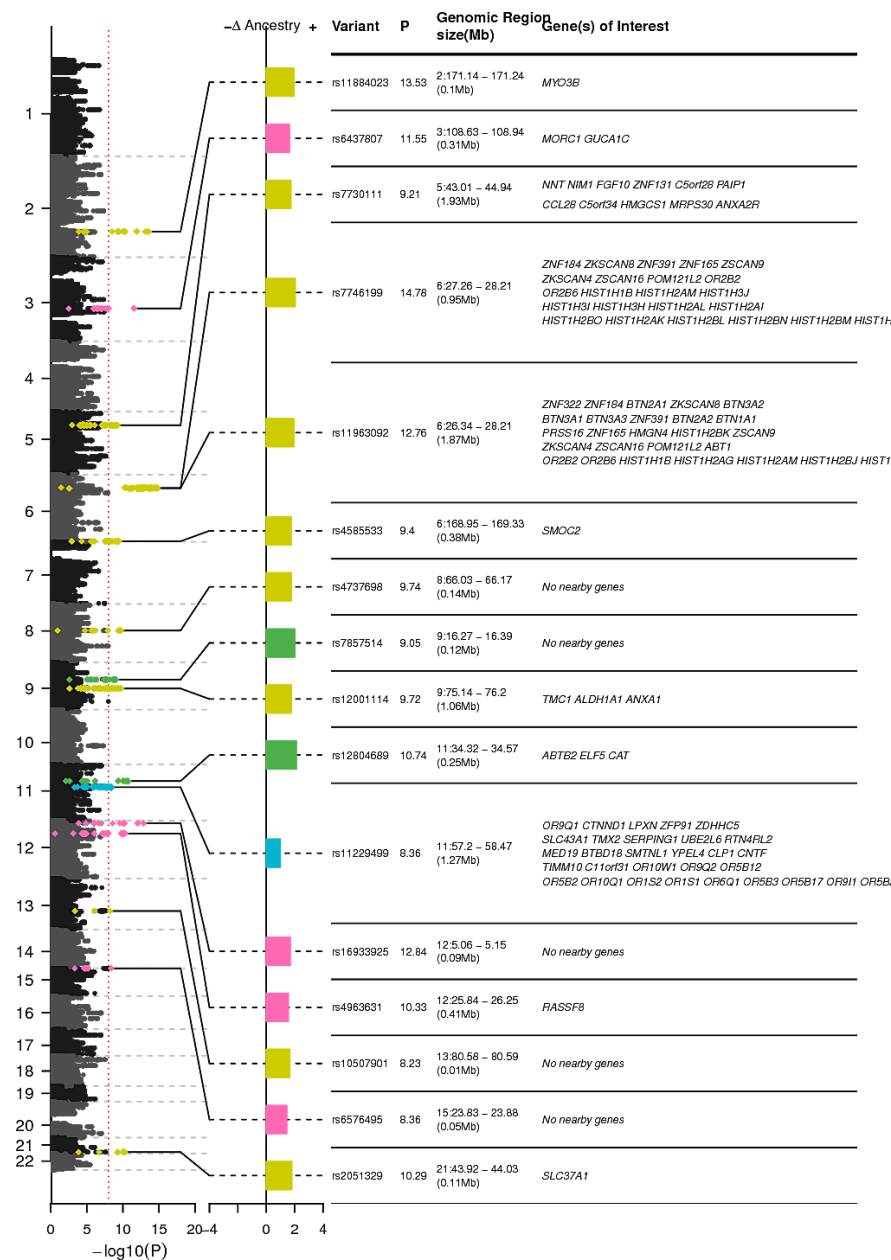
Figure S6: Manhattan plot showing ancestry deviations in the Jola. The left panel shows -\log_{10}(P) values based on the binomial likelihood test for each of the 7 non-self ancestries tested in the Fula. SNPs with P values greater than 8 are highlighted with the colour of the ancestry that the deviation is seen. The central panel shows the change ( \Delta ) in ancestry observed at significant SNPs. The right panel gives information about the top 'hit' SNP and the genes within the genomic region around the hit.
