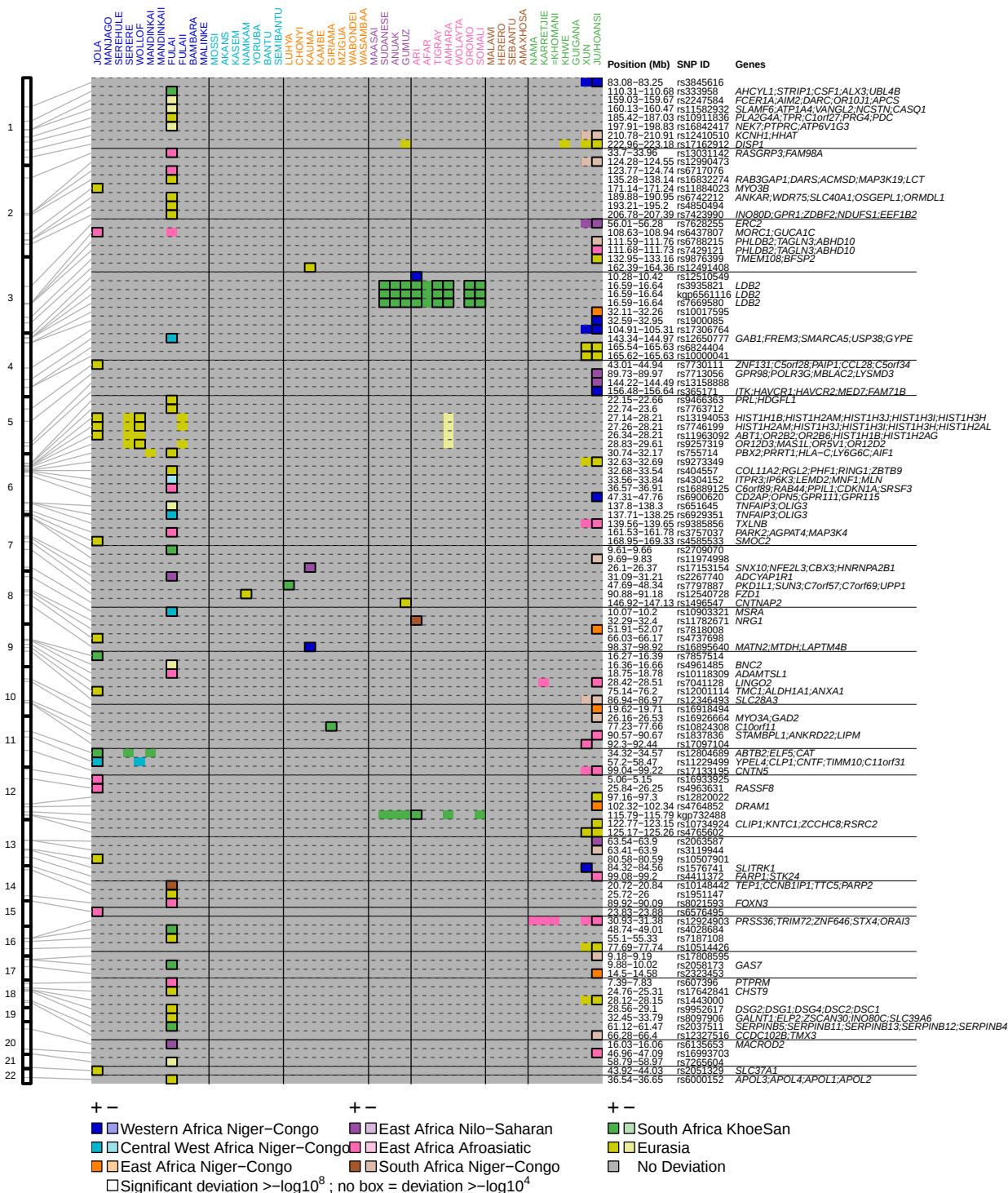
Figure 5: Genome-wide ancestry deviations across sub-Saharan Africa. For each of the 114 loci (rows) where we observe ancestry deviations with a -\log_{10}P \geq 8 , for each population (columns) we show the ancestry that has changed (colour) and the direction of change (lighter colours show decrease, darker increase) and the strength of significance (black box -\log_{10}P \geq 8 ; no box 4 < -\log_{10}P \leq 8 ; grey = -\log_{10}P < 4 ). The positions of the significant loci are shown on the right and genes of interest, together with the detailed genomic region, are shown on the left.
