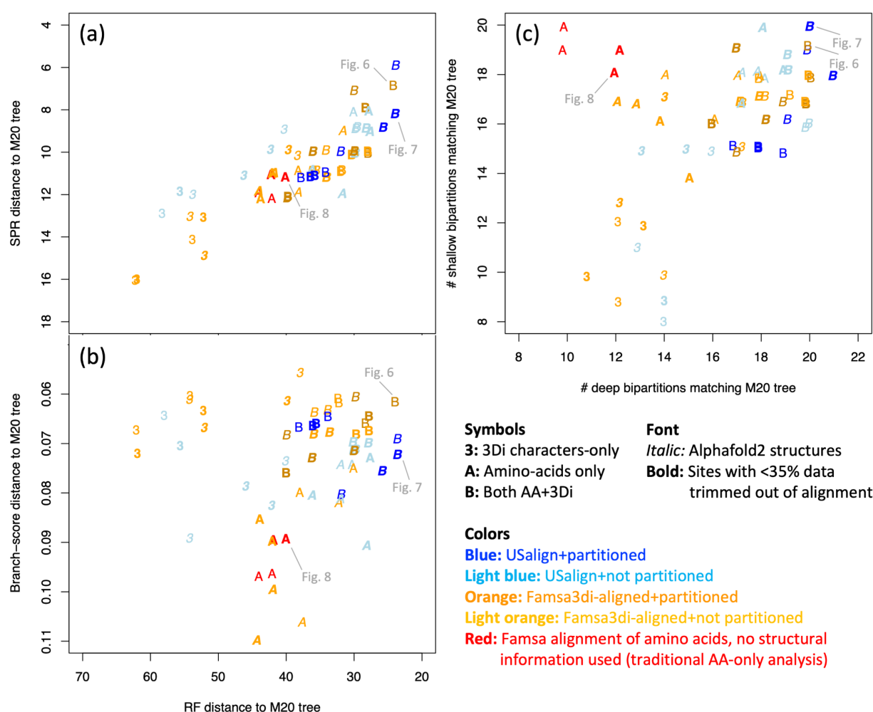
Figure 4. Similarity of all 60 IQtree runs to the Malik et al. (2020) structural-distances NJ tree (M20) for the ferritin-like superfamily. (a) Robinson-Foulds (RF) distance vs. Subtree Pruning-Regrafting (SPR) distance. SPR approximates the number of edits required to match the M20 topology. The closest matches to M20 on both metrics tend to be AA+3Di analyses with partitioning. AA-only and 3Di-only analyses tend to fare worse. (b) RF distance vs. branch-score distance, which takes branch lengths into account, unlike RF and SPR. 3Di-only match M20 well on the branch-score measure, but poorly on RF; however, AA+3Di performs well on both. (c) Number of M20 deep bipartitions matched vs. shallow bipartitions matched. "Deep" bipartitions are those annotated by Malik et al. to indicate major well-recognised categories, and groupings of those. Shallow bipartitions are all others, e.g. groups of 2-5 structures near the tips of the unrooted tree. AA-only runs retrieved shallow bipartitions but not deep ones; 3Di-only was weak on both, but AA+3Di retrieved both shallow and deep. Note: Points have been jittered for visibility.
