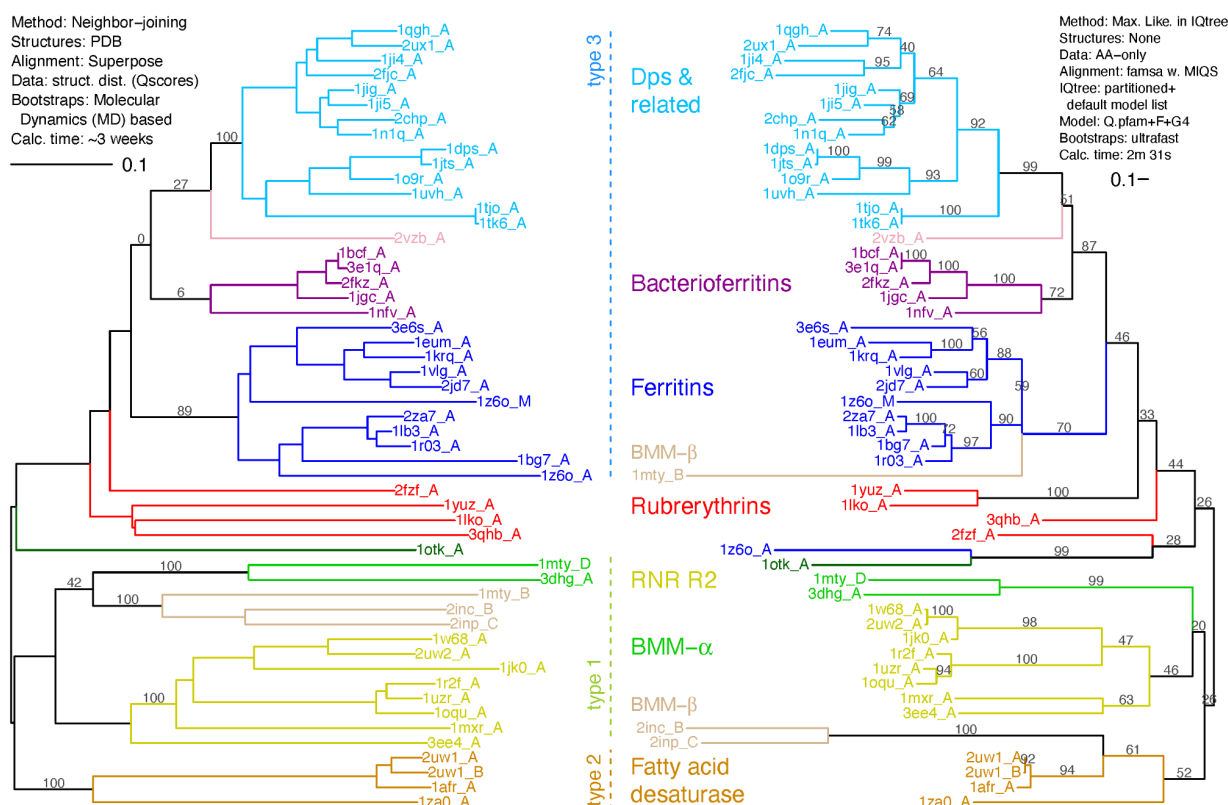
Figure 8. Structure, AA-only ML tree (right) compared to the M20 structural distances tree (left). ML tree is from the closest match "standard" AA-only analysis. The tree shares 12 deep and 19 shallow bipartitions with M20. The types refer to dimer geometries, likely slowly evolving structural characters (Lundin et al. 2012).
