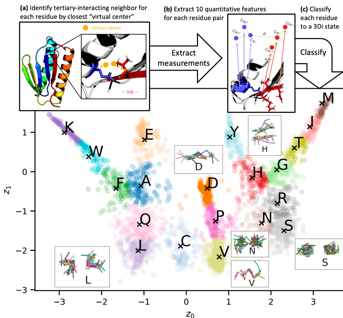
Figure 1. Summary of Foldseek's system for classifying tertiary interactions into the 20-state 3Di alphabet. For each residue in a protein structure (a) a virtual center is defined, and each residue is assigned a tertiary neighbor based on the closest virtual center. (b) 10 quantitative traits are collected for each residue+neighbor interaction, and then (c) assigned to the best-matching 3Di state using the classifier pre-trained by Van Kempen et al. 2023. The main panel shows a two-dimensional representation of the 20 states. Examples of 3Di states are inset; each of these represents 10 pairs of backbone fragments showing the typical arrangement for a 3Di state. Graphics modified from Van Kempen et al. 2023.
