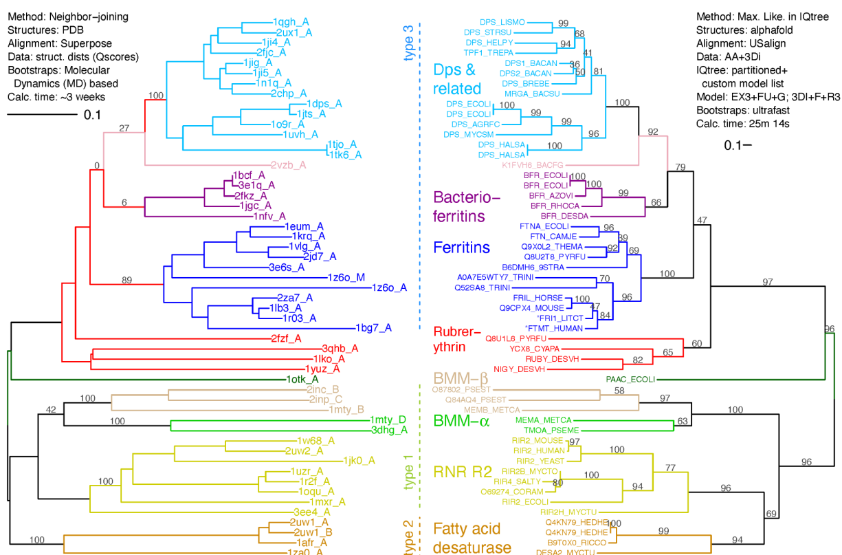
Figure 7. AlphaFold-based ML AA+3Di tree (right) compared to the M20 structural distances tree (left). This ML run was the closest overall topology match to the M20 tree, and shares 20 deep and 20 shallow bipartitions with M20. Tip labels are Uniprot IDs for which AlphaFold predictions were downloaded. Each Uniprot label on the right represents the closest AA match to the corresponding PDB structure on the left, with the exception of two tips marked with asterisks; here, FRI1_LITCT corresponds to 1bh7_A, and FTMT_HUMAN corresponds to 1r03_A. The types refer to dimer geometries, likely slowly evolving structural characters (Lundin et al. 2012).
