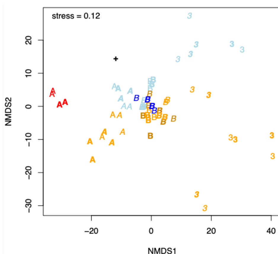
Fig. 5. Nonmetric Multidimensional Scaling (NMDS) representation of the 61x61 matrix of RF distances between all ML trees (60 IQtree runs + the M20 tree). Values <0.1 are typically taken to indicate "excellent," and <0.2 "good," 2-dimensional approximations of the original distances (Clarke 1993). Legend as in Figure 4. M20 tree = +. The trees using both AA+3Di data ("B") show a merger of both signals and cluster tightly, compared to the variability between the AA-only or (particularly) 3Di-only trees.
