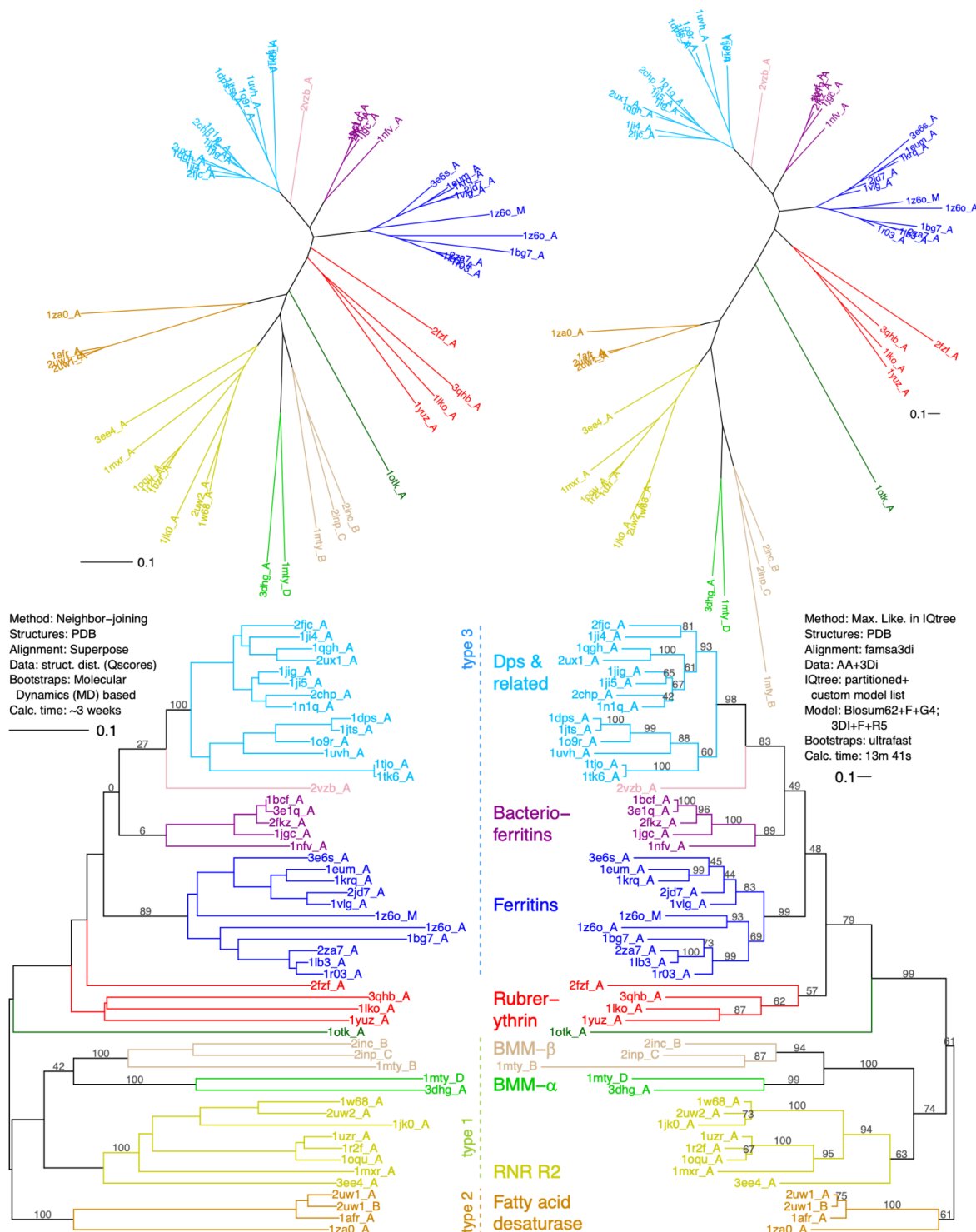
Figure 6. Comparison of trees using PDB structures. Left: M20 structural distances tree, with MD-based bootstraps where available in Malik et al. 2020. Right: the closest-match PDB-based IQtree analysis using AAs+3Di from PDB structural data. This tree shares 20 deep and 19 shallow bipartitions with M20. Top row: unrooted trees. Bottom: arbitrary rooting for visual comparison. Branch length units for the M20 tree are Q_{score} -based distances; for the ML tree they are expected substitutions per site. The types refer to dimer geometries, likely slowly evolving structural characters (Lundin et al. 2012).
