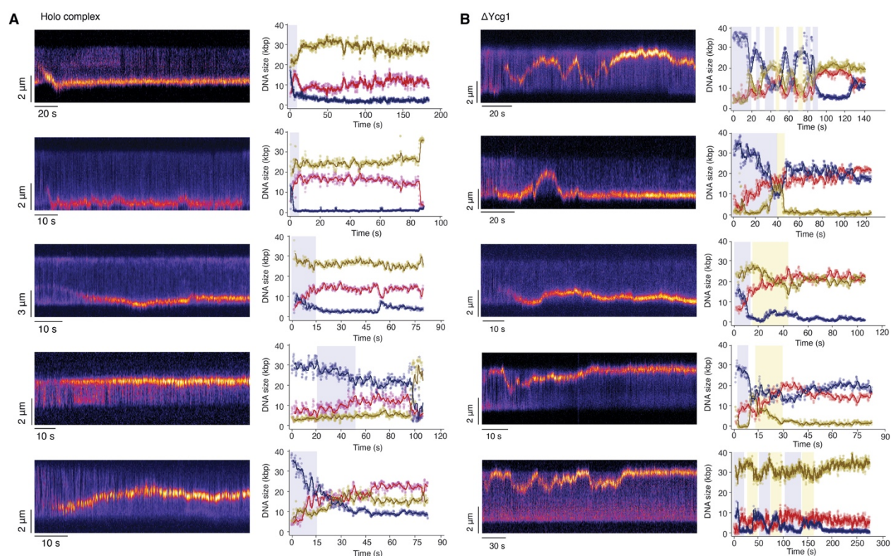
Fig. S20. Additional examples of DNA loop extrusion events by Ct holo and \Delta Ycg1 condensin. Kymographs of DNA loop extrusion by Ct holo (A) and \Delta Ycg1 (B) condensin and fluorescence intensity plots of the DNA regions above (yellow) and below (blue) the extruded DNA loop (red). Shaded regions indicate an increase in the DNA loop and concurrent decrease of the DNA region above (yellow) or below (blue) the loop.
