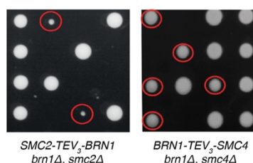
Fig. S4. In vivo functional analysis of SMC-kleisin fusion proteins. Tetrad dissection of diploid yeast strains after 3 days at 25 °C. Colonies of cells expressing Smc2–Brn1 or Brn1–Smc4 fusion proteins as their sole source of Brn1 and Smc2 or Smc4, respectively, are indicated by circles
