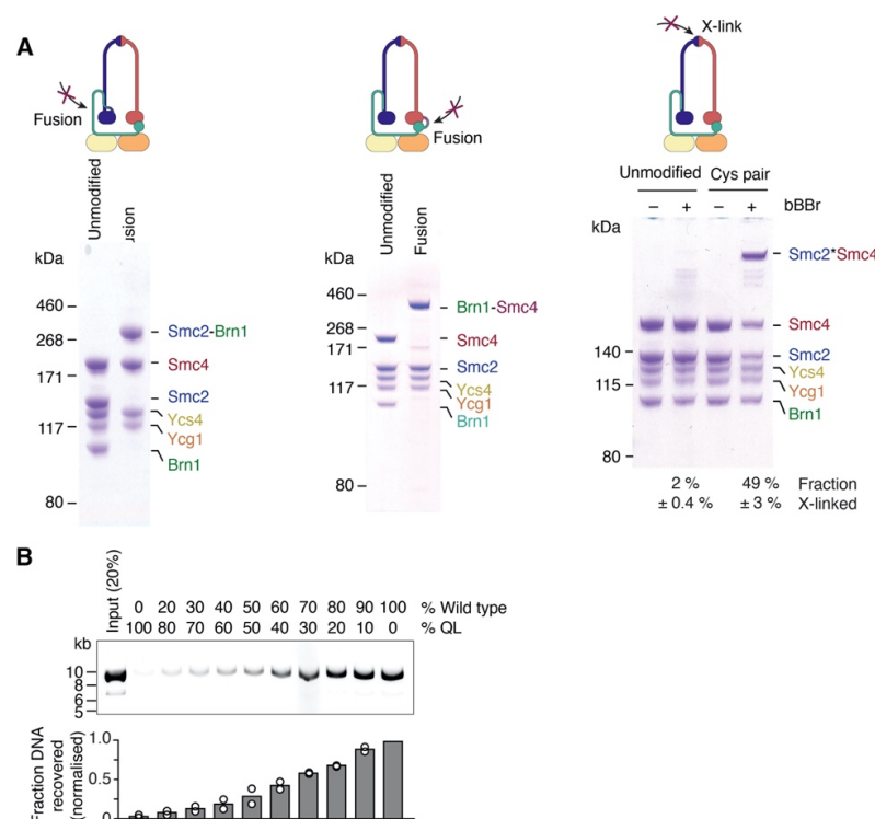
Fig. S2. Closure of SMC-kleisin ring interfaces. (A) SDS-PAGE of purified unmodified, Smc2-Brn1 fusion, Brn1-Smc4 fusion, or cross-linkable hinge (Smc2 K639C ; Smc4 V721C ) condensin complexes after staining with Coomassie Brilliant Blue. The fraction of cross-linked species was estimated by densitometry (mean \pm s.d., n = 3 ). (B) Formation of salt-resistant condensin-DNA complexes using a mixture of wild-type and QL catalytic mutant (Smc2 Q147L ; Smc4 Q302L ) condensin as in Fig. 1B. The graph shows the quantitation of salt-resistant DNA fractions for each ratio after ethidium bromide staining (mean, n = 2 ).
