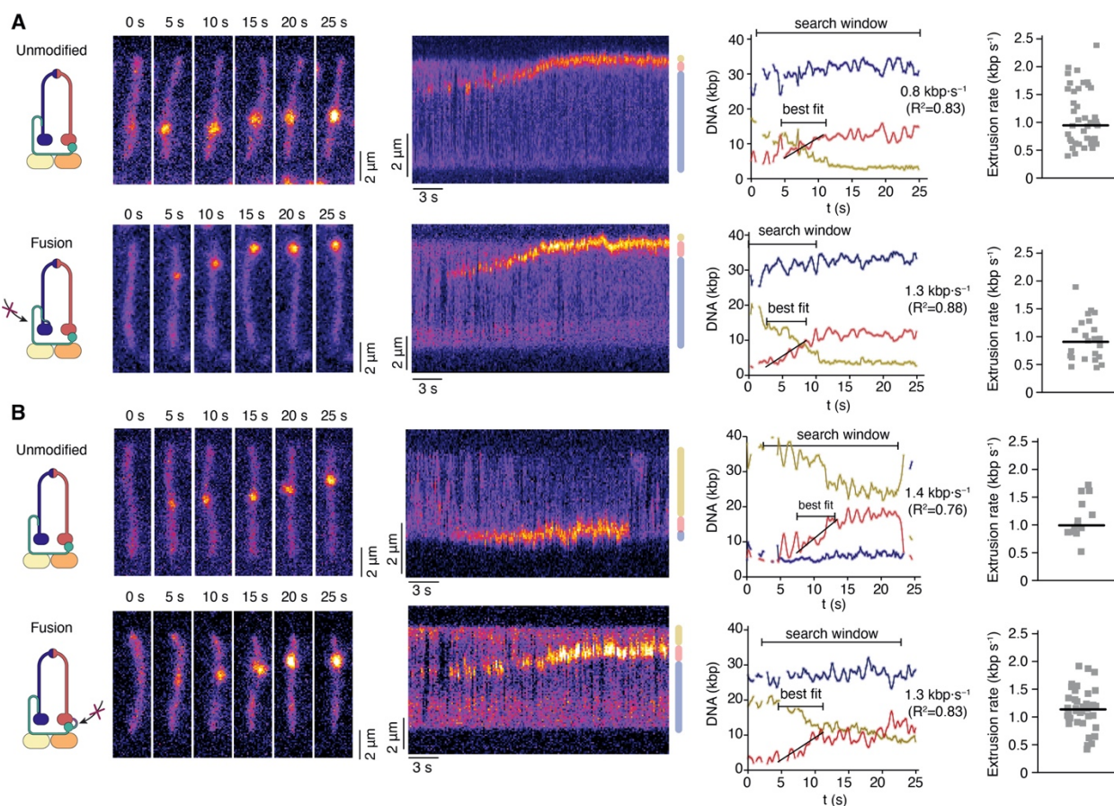
Fig. S3. DNA loop extrusion by condensin with fused SMC-kleisin interfaces. (A) Stills and kymographs of surface-tethered \lambda -phage DNA (48.5 kbp) stained with SxO and incubated with unmodified or Smc2–Brn1 fused condensin. Graphs show quantitation of DNA in (red), above (yellow) and below (blue) the loop. A user-defined search window was selected in which the slope of the best linear fit of 50 consecutive data points was taken as loop extrusion rate. Individual loop extrusion measurements and the median (line) are plotted. (B) As in (A) for Brn1–Smc4 fusion condensin. See also movie S1 .
