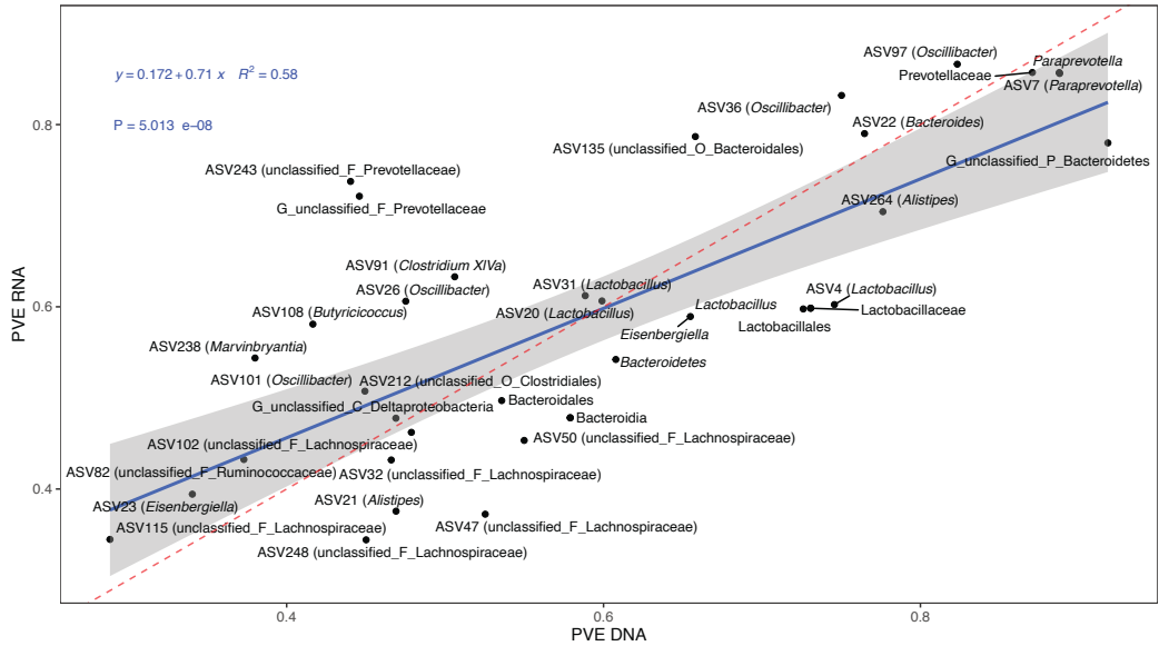
758 Supplementary figure 4: Correlation of SNP-based heritability estimates based on DNA (x- 759 axis) or RNA (y-axis). The blue line represents a linear regression fit to the data. Red dashed 760 line represents the identity line with a slope of 1.
