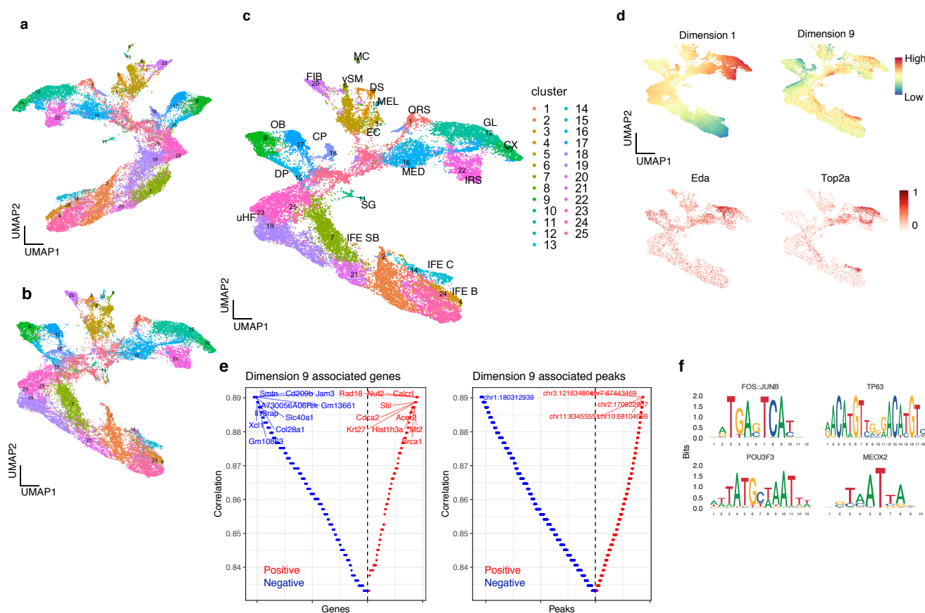
Figure 4: scMM analysis on the mouse skin SHARE-seq dataset. a , b , c , UMAP visualization of unimodal latent variables for transcriptome, chromatin accessibility, and multimodal latent variables, respectively. Each dot represents a single cell and is color-coded according to the clustering performed on multimodal latent variables. d , Upper panels: multimodal UMAP visualization color-coded based on latent dimension values. Middle and lower panels: UMAP visualization colored according to transcriptome counts for cell type markers. e , Genes (left panel) and peaks (right panel) associated with latent dimension 9. Each feature was aligned based on Spearman correlation coefficient. The y-axis represents the absolute correlation coefficient, where red and blue colors represent positive and negative correlations, respectively. f , Motif plot for representative motifs significantly enriched in peaks positively associated with latent dimension 9.
