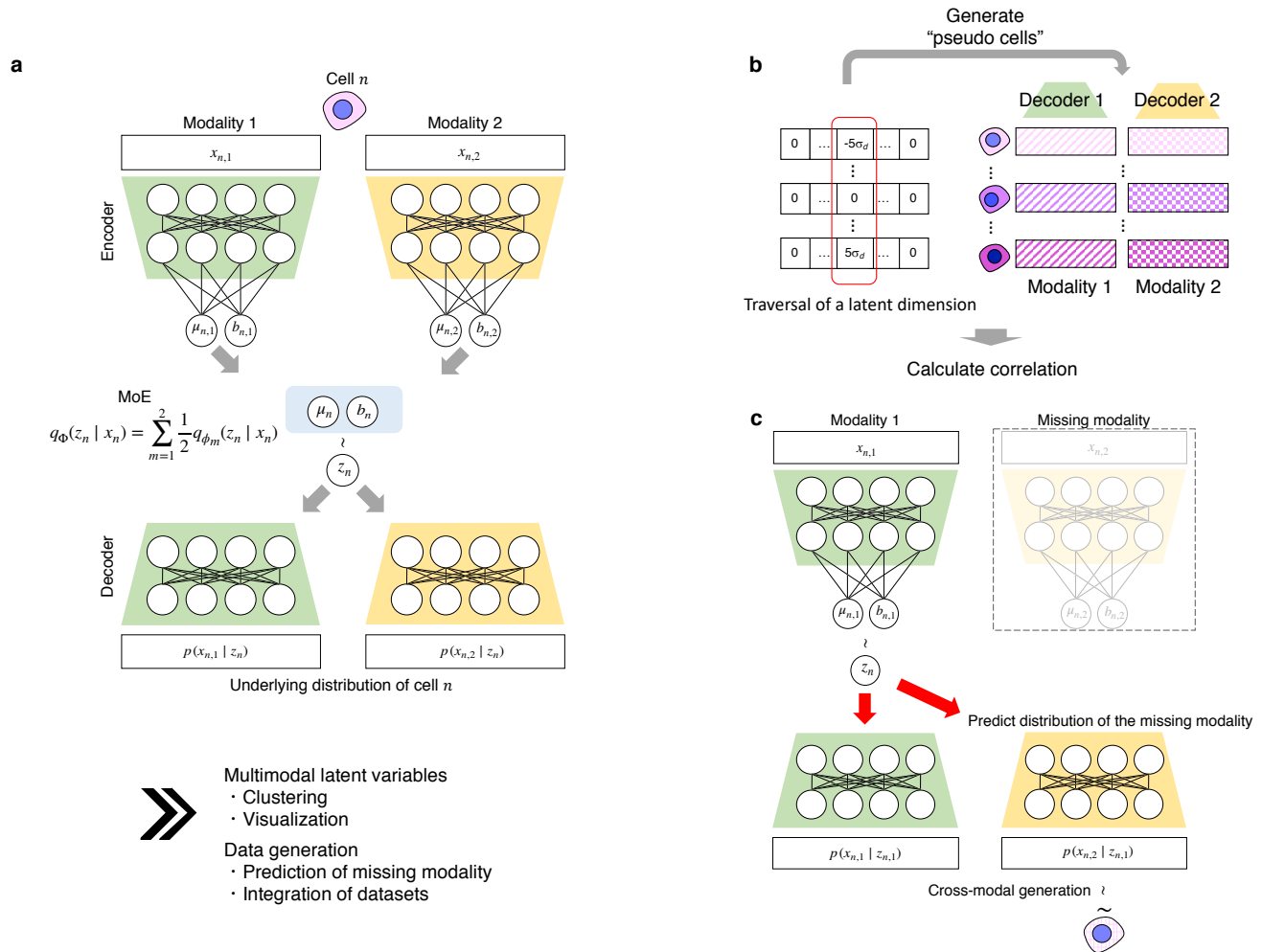
Figure 1: Conceptual view of single-cell multimodal data analysis by scMM. a , The underlying model of scMM. scMM takes feature vectors of each modality as input to separate encoders. The model is trained to learn low-dimensional joint variational posterior factorized by a mixture-of-experts (MoE). Decoders reconstruct the underlying probability distributions for data in each modality from latent variables. During the training processes, latent variables from one modality are used to reconstruct data in both modalities. b , Schematic view of procedure for finding latent dimension-associated multimodal features by independently traversing each dimension. c , Schematic view of cross-modal generation by trained scMM model when one modality is missing. For further details, see the Methods section.
