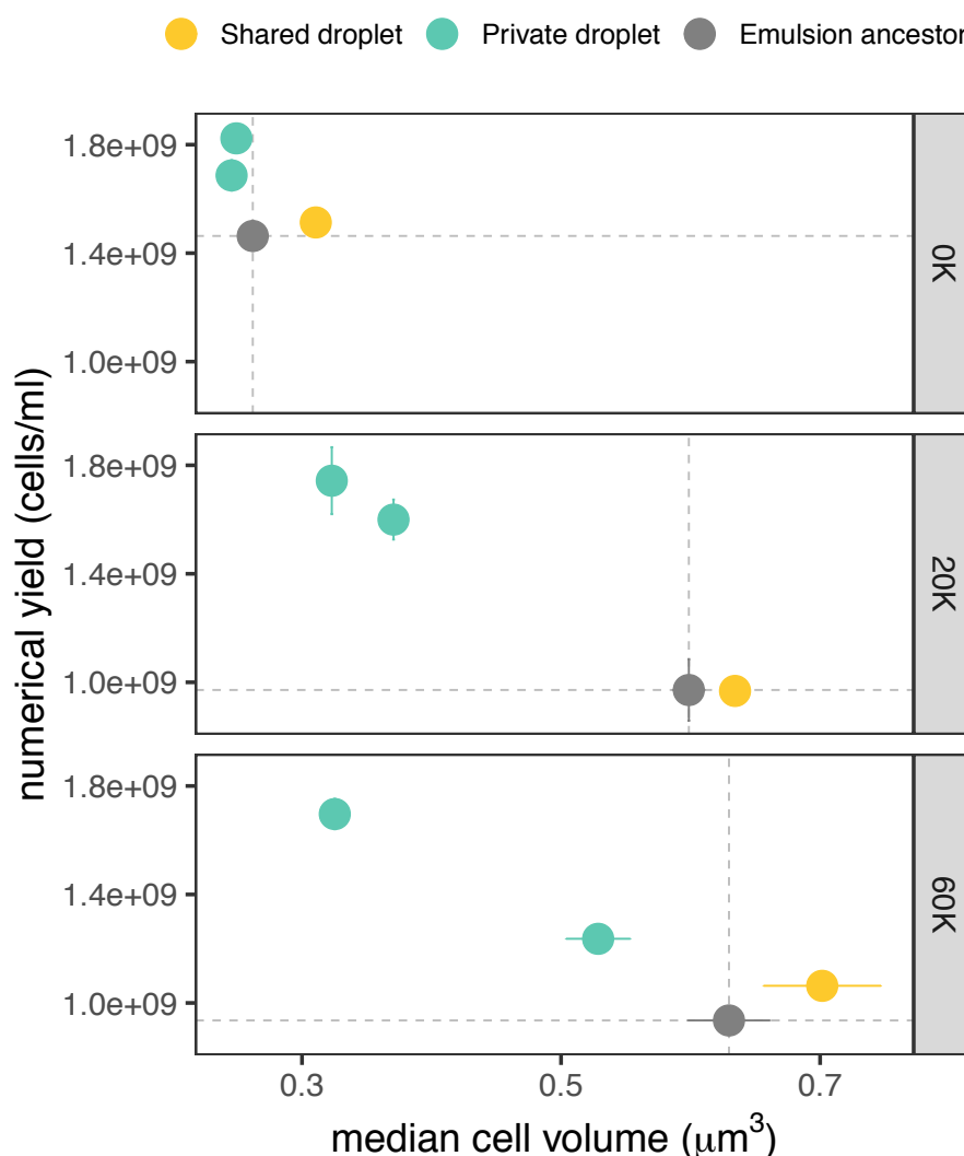
Figure 5: Median cell volume compared to numerical yield. Each panel shows strains originating from a single emulsion ancestor (in grey, at right) from the Ara-5 lineage of the LTEE (0, 20,000, and 60,000 generations). Colors indicate emulsion evolution treatments (labels at top). The coordinate positions of each point show the average of three replicate assays for each phenotypic trait. Error bars show SEM; when they are not visible along either axis, the corresponding SEM is smaller than the symbol itself. Dashed lines show the mean numerical yield and cell volume of the relevant ancestor.
