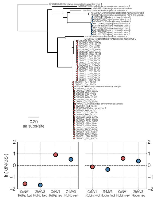
Fig. 1. a A maximum-likelihood tree illustrating the relationship between CxNV1 ( Culex narnavirus 1 ) (red) and ZJMV3 ( Zhejiang mosquito virus 3 ) (blue) and related narnavirus RdRp amino acid sequences. b ORF-wide dN/dS values for forward and reverse directions of RdRp and Robin segments for both viruses.
