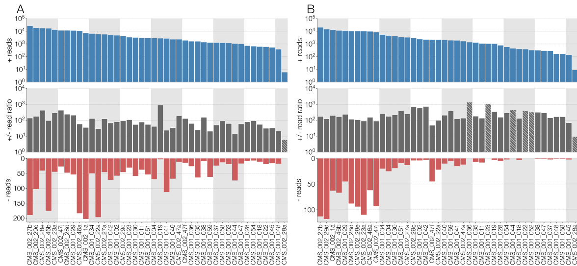
Fig. 2. A) Number of reads (from top to bottom): in the positive sense (i.e., same as genomic) with respect to RdRp segment of Culex narnavirus 1 , the ratio of positive- to negative-sense reads, and negative-sense reads. Numbers of positive-sense reads and ratio of positive- to negative-sense reads are log-scaled while number of negative reads is displayed in normal space. Ratios where no negative sense reads could be identified are highlighted with hatches and the ratio reflects positive-sense reads (i.e., by assuming there is one negative-sense read). B) Same information as A , but showing read numbers for Robin segment of Culex narnavirus 1 . The results are displayed for the 42 different strains, with the samples ordered in descending order of the total number of reads for each segment.
