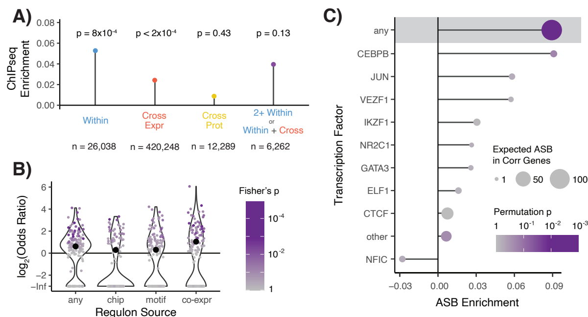
Figure 3. TF binding of TF-eQTL interactions. A) Overlap enrichment of TFBS, based on TF ChIP-seq peaks, of TF-eQTL interactions by dataset. Permutation-based p -values are plotted above each measurement. Datasets include within-tissue (blue) interactions, cross-tissue expression-based (red), cross-tissue protein-based (yellow), and TF-eQTL interactions with at least two lines of evidence from cross-tissue expression-based and within-tissue interactions (purple). B) The enrichment of target genes with two lines of evidence for TF-eQTL interactions falling into that TF's regulon. Large black dots depict overall enrichment across TFs. C) Enrichment for allele-specific TF binding (ASB) for TF-eQTL interactions with two lines of evidence. Shaded area contains statistics for unmatched TF ASB analysis. Below that, statistics for matched TF ASB analysis is shown, with TFs with more than one expected ASB event plotted individually, and all other TFs combined (other).
