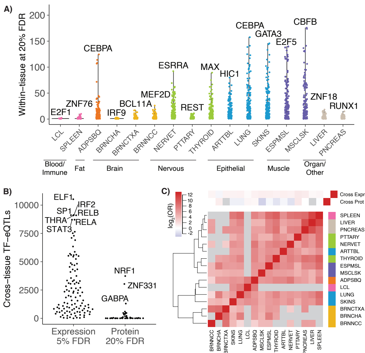
Figure 2. Discovered TF-eQTL interactions. A) Number of within-tissue TF-eQTL interactions at 20% FDR is plotted per TF for each tissue analyzed. The TF with the most interactions per tissue is highlighted. B) Number of discovered cross-tissue TF-eQTL interactions per TF for expression-based interactions (at 5% FDR) and for protein-based interactions (at 20% FDR). TFs with the most correlations per analysis are highlighted. C) Sharing of TF-eQTL interactions between tissues and within/cross-tissues. Red indicates positive enrichment and blue, negative enrichment. Grey squares indicate no shared TF-eQTL gene pairs between the two datasets.
