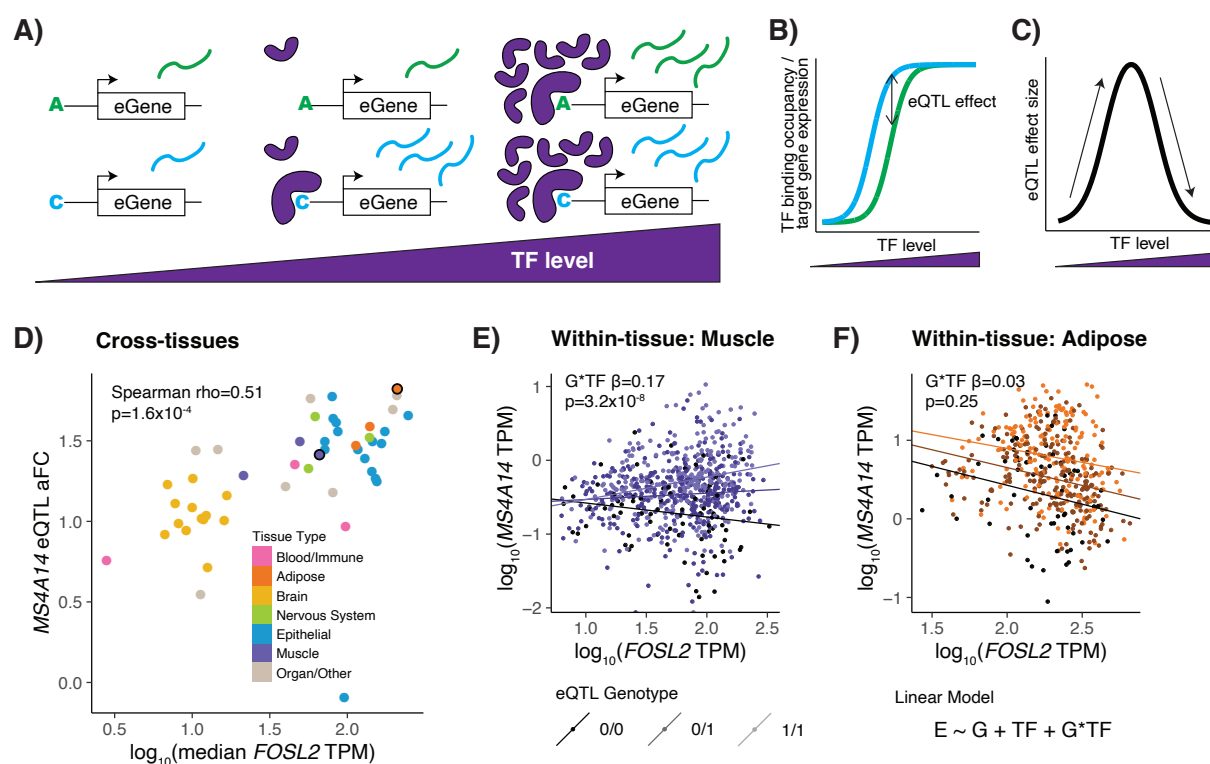
Figure 1. TF model of eQTL effects. A) TF binding to an eQTL variant with different allelic TF affinities is depicted at low, medium, and high TF levels. B) TF binding occupancy, resulting in target gene expression, for the two eQTL alleles across TF levels. C) Difference in expression of alleles or eQTL effect size, quantified as \log_2 allelic fold change, across TF levels. Our applied models only examine monotonic effects, which can be imagined as different sides of the hill. D) Tissues are plotted by eQTL effect size vs.
