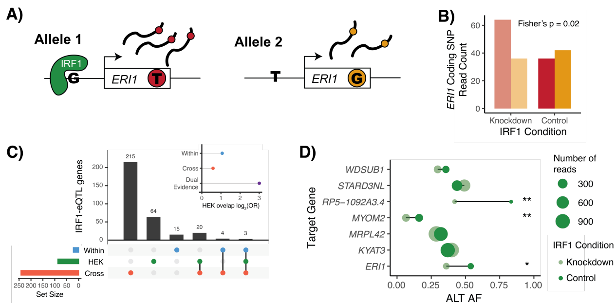
Figure 4. IRF1-eQTL interactions in HEK293-TLR4 IRF knockdown. A) Depiction of allele-specific expression, with IRF1 preferentially binding to the G-allele in the regulatory region of the ERI1 target gene. This leads to higher expression of allele 1, which we can measure based on the presence of a heterozygous coding SNP in the ERI1 transcript. Reads from allele 1 will have a T genotype (red) at the coding SNP and reads from allele 2 will have a G (orange). B) Read counts for ERI1 coding SNP alleles in both knockdown and control conditions. In this example, it appears that we observe allelic effects at lower (knockdown) IRF1 levels, while higher (control) levels of IRF1 may saturate binding to both alleles. Conditions are compared using Fisher's exact test of allelic counts. C) Sharing of IRF1-interacting eQTL genes in within-tissue (blue), cross-tissue expression-based (red), and HEK293 IRF1 knockdown (green) datasets. Only genes with an adequately expressed heterozygous coding SNP in HEK293 samples are included. Inset shows enrichment for overlap between HEK293T IRF1-eQTL genes and listed datasets. D) HEK293 coding SNP alternative allele frequency in dual-evidence IRF1-eQTL genes that were heterozygous for a top TF-eQTL variant and had adequate coverage of a heterozygous coding SNP. * indicates a Fisher's p value < 0.05, ** < 0.01 of allelic counts vs. condition.
