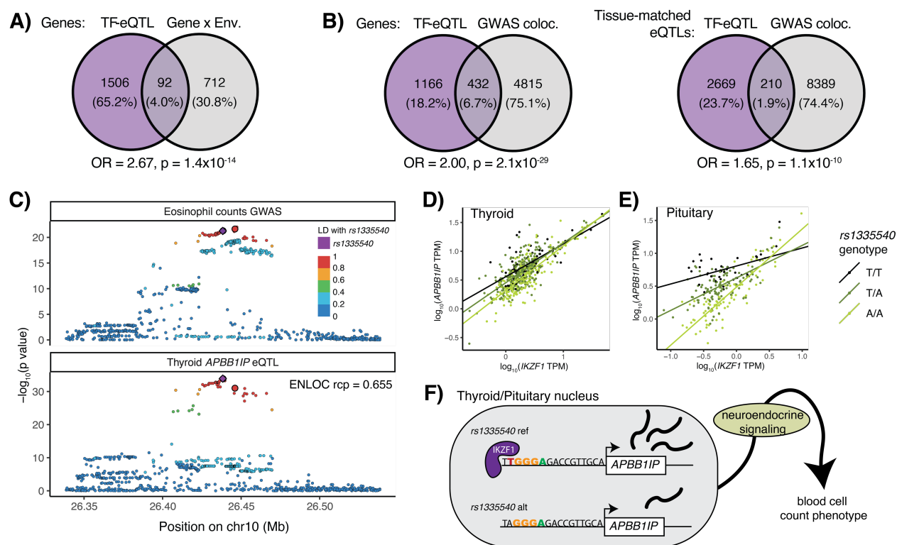
Figure 5. TF-eQTL implications for gene-by-environment and GWAS effects. A) Overlap of TF-eQTL genes with GxE genes from Findley et al. 2021. B) Overlap of TF-eQTL genes with GWAS colocalizing eQTL genes from GTEx. The first diagram shows overlap for a gene with a TF-eQTL in any tissue and colocalizing eQTL in any tissue. The second shows overlap of tissue eQTLs with TF-eQTL and/or colocalizing GWAS locus in the given tissue. C) Representative eQTL and GWAS p-values are plotted for variants in the region of an APBB1IP eQTL and blood trait GWAS locus. Lead variants from IKZF1-eQTL interactions in thyroid, pituitary, and tibial artery are larger and outlined in black. (The lead variant from pituitary/artery cannot be seen as it falls behind rs1335540.) D) & E) Individual samples in thyroid and pituitary tissues are plotted by IKZF1 and APBB1IP expression, and linear regression lines are plotted by genotype. The difference in APBB1IP expression between the genotypes gets smaller as IKZF1 expression increases across the samples. F) Schematic of IKZF1 regulation of APBB1IP and blood cell counts. An IKZF1 binding site predicted by the HOCOMOCO IKZF1 motif lies nine bases upstream of APBB1IP's transcription start site, which is disrupted by the alternative allele of rs1335540. Under our neuroendocrine signaling hypothesis, APBB1IP expression in neuroendocrine tissues goes on to alter system-wide neuroendocrine signaling, which would cause changes in blood cell counts. As IKZF1 appears to regulate the APBB1IP eQTLs in these tissues, it would follow that IKZF1 TF therefore may regulate the effect of this locus on blood cell counts.
