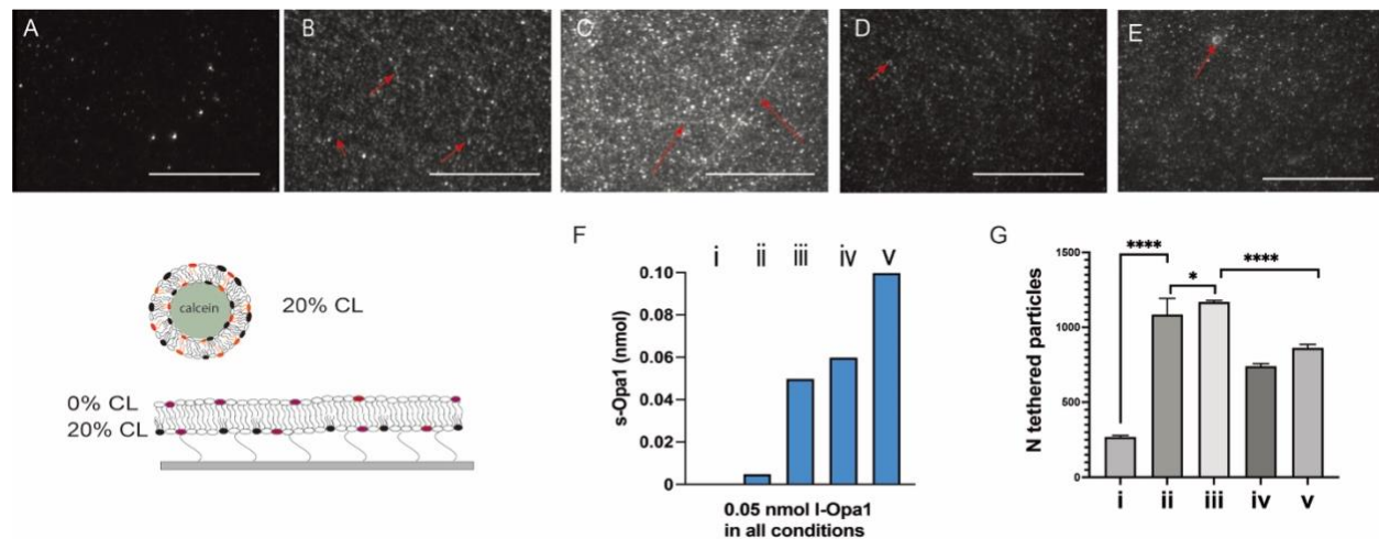
Fig 3. Effect of s-Opa1 on proteoliposome tethering to an asymmetric CL bilayer. A. In the presence of GTP, few l-Opa1 proteoliposomes are tethered to an asymmetric CL bilayer containing l-Opa1. Upon s-Opa1 addition, proteoliposome tethering increases significantly. Panels B-E show representative images varying l-Opa1 and s-Opa1 concentration shown in panel F as i-iv. l-Opa1 concentration was fixed at 0.05 nmol in all conditions. Scale bar, 20 \mu m. Red arrows indicate tubular structures tethered to the bilayer. G. Quantification of the number of proteoliposomes tethered to the bilayer, based on 10-20 random points in each experiment, for a total of 3-5 different experiments. Data were analyzed using t-test. The illustrations indicate lipid distribution in the membrane, with both bilayers containing reconstituted l-Opa1.
