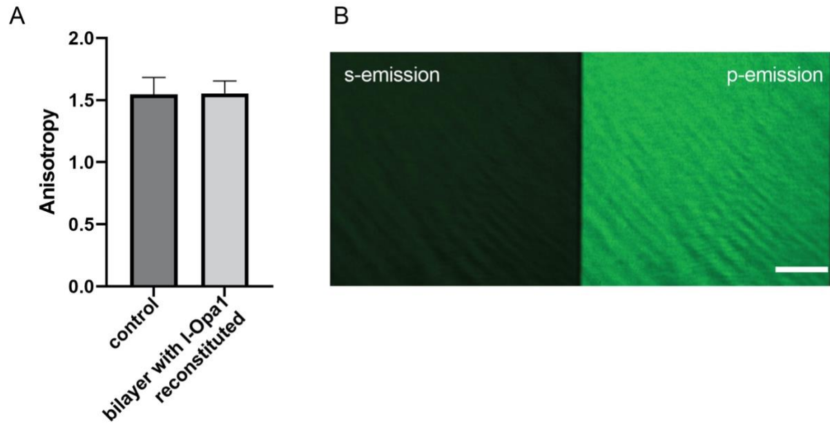
Supplemental Fig. 1 I-OPA1 reconstitution does not affect CL asymmetry. A. Calculated anisotropy before and after I-OPA1 reconstitution suggest a similar cardiolipin distribution in the bilayer. B. shows the fluorescence images obtained in s-emission and p-emission channels.
