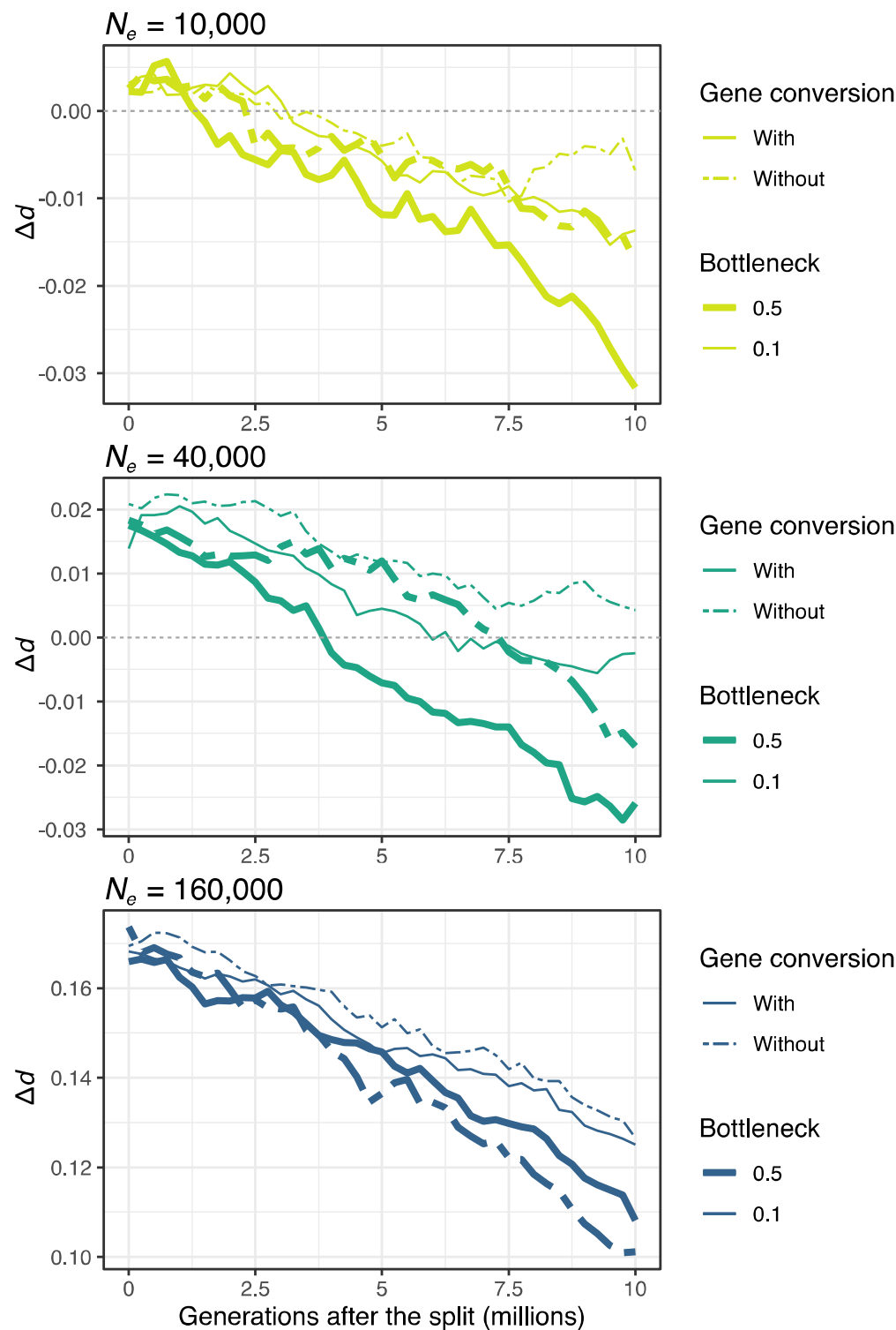
Fig. 4. Plots showing the decay of \Delta d over time in the evolutionary simulations based on the models with and without gene conversion, and with a mild (0.5) and a severe bottleneck (0.1) for each of the three simulated ancestral N_e .
