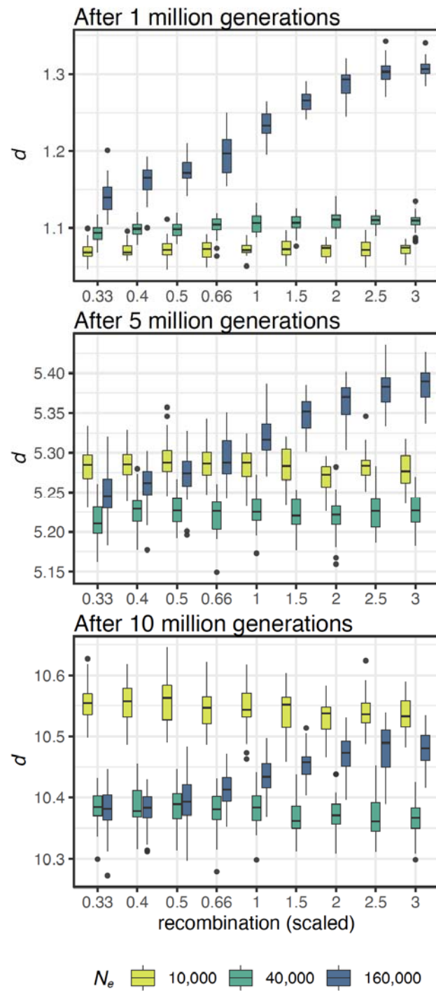
Fig. 3. Boxplots summarizing results from evolutionary simulations on the relationship between recombination rate and d in models with selection and without gene conversion in each of three simulated ancestral N_e and three time points after the split from the ancestral pop A and a mild bottleneck. Gene conversion was not included in these models as no significant differences were found between models with and without gene conversion. (See Fig. S5 for comparisons with neutral models and models with a more severe bottleneck).
