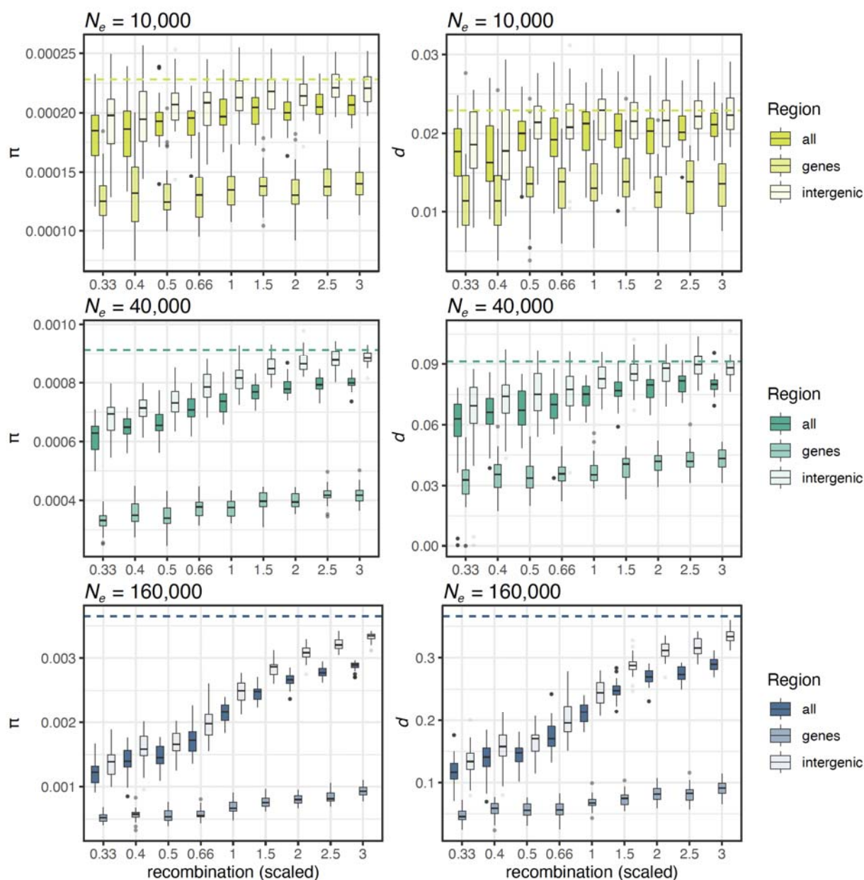
Fig. 2. Boxplots summarizing results from evolutionary simulations on the relationship between recombination rate and \pi after 20N_e generations in the ancestral population (panel A on the left) and d one generation after the split after a mild bottleneck ( 0.5 of ancestral N_e ) between the two daughter populations (panel B on the right) in each of three simulated ancestral N_e . Boxplots refer to the results from the models with selection and the dashed line shows the results from the neutral models. Here are the results with models without gene conversion as no significant differences were found between models with and without gene conversion.
