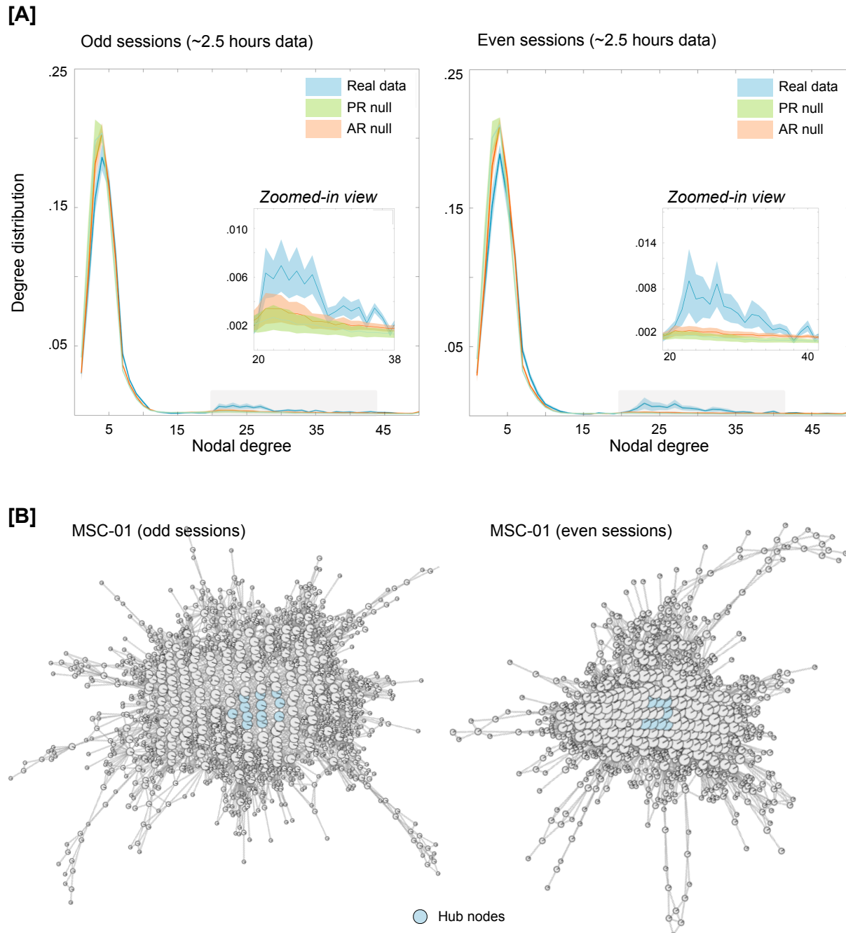
Fig. 2: Characterizing the Mapper-generated graph using degree distribution. [A] Degree distributions averaged across the ten participants, separately for odd and even sessions. For examining linear vs. nonlinear aspects, two null models were used, namely, the phase randomized null and the multivariate autoregressive null model. As evident from the degree distribution plots, real data were significantly fat tailed ( >20 ) compared to both nulls. This finding was independently replicated in both halves of the data. The shaded area represents standard error around the mean (S.E.M.). [B] Mapper-generated graphs for a representative participant (MSC-01), highlighting hub nodes (i.e., nodes with high degree ( >20 ) and high centrality (top 1%)). Similar plots were observed across all MSC dataset participants (see Fig. S2).
