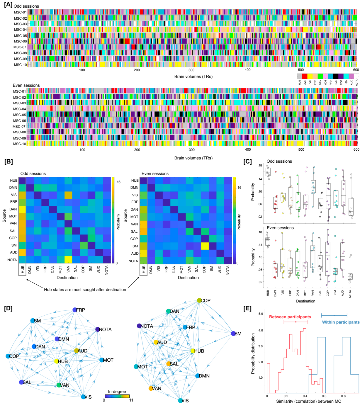
Fig. 6: Traversal in the temporal domain at the single frame level. [A] Depicts transitions in brain activation over time frames in terms of dominant individual-specific RSNs (or hub-like states). Each time frame (TR) was labeled from the Mapper-generated shape-graphs by propagating the RSN-based annotation from each graph node to the time frames represented by that node. In addition to RSNs, a new label representing hub-nodes was also generated. As evident, hub state was often visited by participants across both data splits. Only showing a subset of timeframes (first 600 frames) for each participant for ease of viewing. [B] A discrete-time Markov chain was estimated using RSN-based labels for each participant and data split. While estimating transition probabilities, transitions due to motion censoring and session boundaries were discarded. Here, we present transition probability matrix averaged over all 10 MSC participants. Diagonals were suppressed to better illustrate transition probabilities across states. The hub state was observed to be the most sought-after destination from any other state. [C] Boxplots
