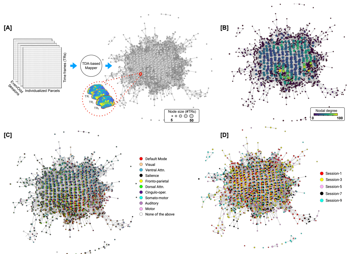
Fig. 1: Estimation and characterization of the dynamical structure underlying transitions in intrinsic brain activity using our TDA-based Mapper approach. Here, we present data from a representative participant (MSC-01; odd sessions). [A] Individualized parcellated data from the highly sampled Midnight Scan Club (MSC) individuals 53 was split into two halves: odd sessions (2.5 hours) and even session (2.5 hours) sets. The Mapper approach was independently run on each set to generate the underlying structure as a graph. Each graph consists of nodes and edges, where the nodes could in turn contain multiple whole-brain volumes (or TRs; size of a node represents the number of TRs). The nodes are connected if they share TRs. [B] The Mapper-generated graph can be characterized in several ways. Here, we examine topological properties by annotating the graph nodes using nodal degree. [C] The graph can also be annotated with meta-information to characterize the mesoscale structure. Here, we show annotation using the activation of individual-specific resting state networks (RSNs). A pie-chart based annotation is used to reveal the proportion of time frames with each node belonging to different RSNs. [D] Similarly the graph can also be annotated using other available meta-information, e.g., session information.
