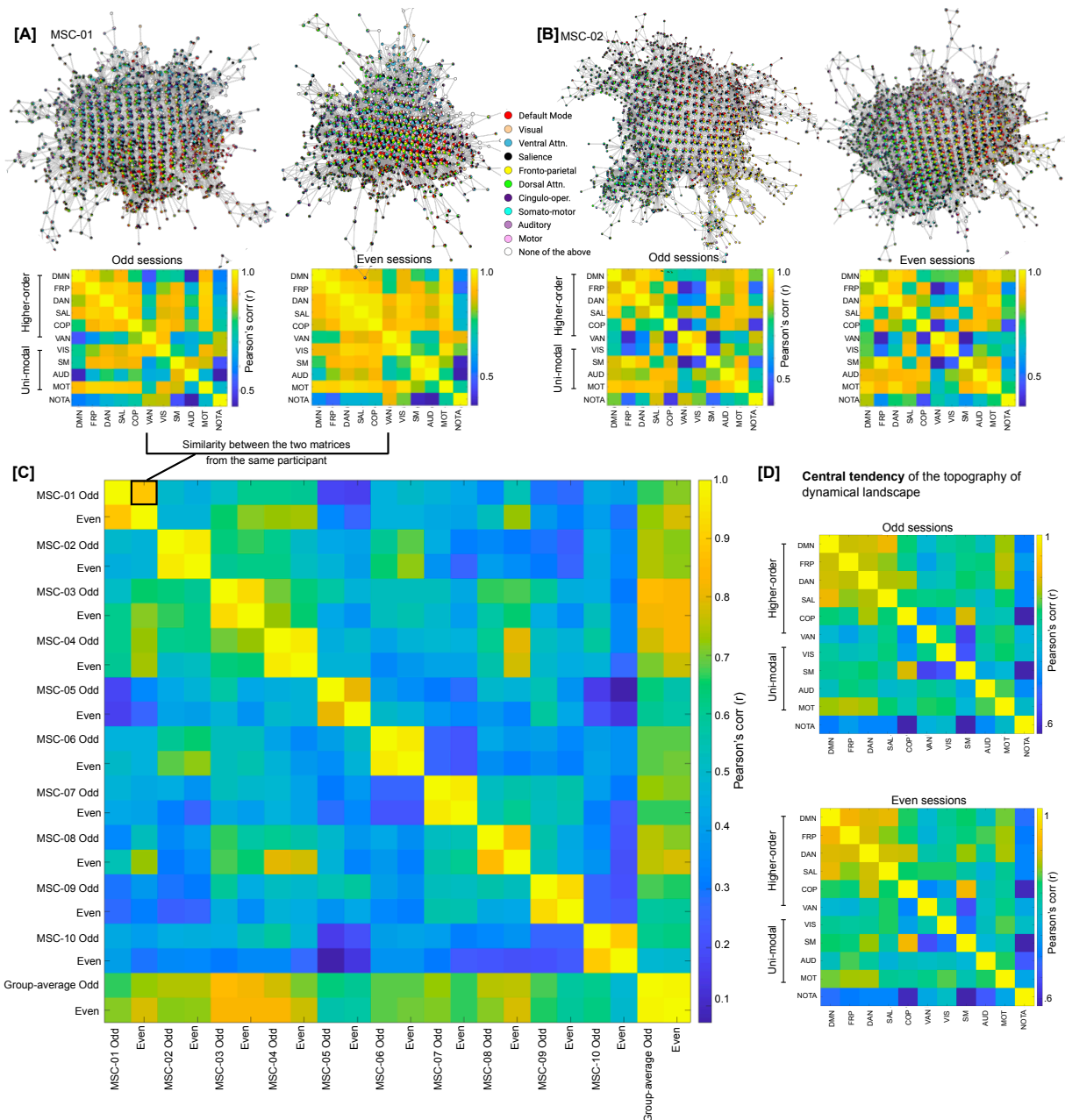
Fig. 4: Dynamical landscapes and their organization are subject specific. [A-B] Mapper-generated graphs annotated by RSN activation for two representative participants (MSC01-02) are shown. Both split halves (odd and even sessions) are shown for each participant. For each half, the figure also shows a similarity (correlation) matrix between RSNs, where high correlation between two RSNs suggest co-location on the Mapper-generated graph. As evident through Mapper-graph annotations and between network correlations there was high degree of similarity between two halves of the same participant. [C] To quantify between- vs within-participant correspondence across network similarity matrices, network similarity matrices were compared across split halves from all participants. As shown in the between subject matrix, high correspondence was observed for within-participant matrices, suggesting dynamical landscapes demonstrated idiosyncratic, yet highly replicable, topological signature at the level of canonical resting state networks. [D] Central tendency of the dynamical landscape, averaged over ten highly sampled individuals, for odd and even sessions.
