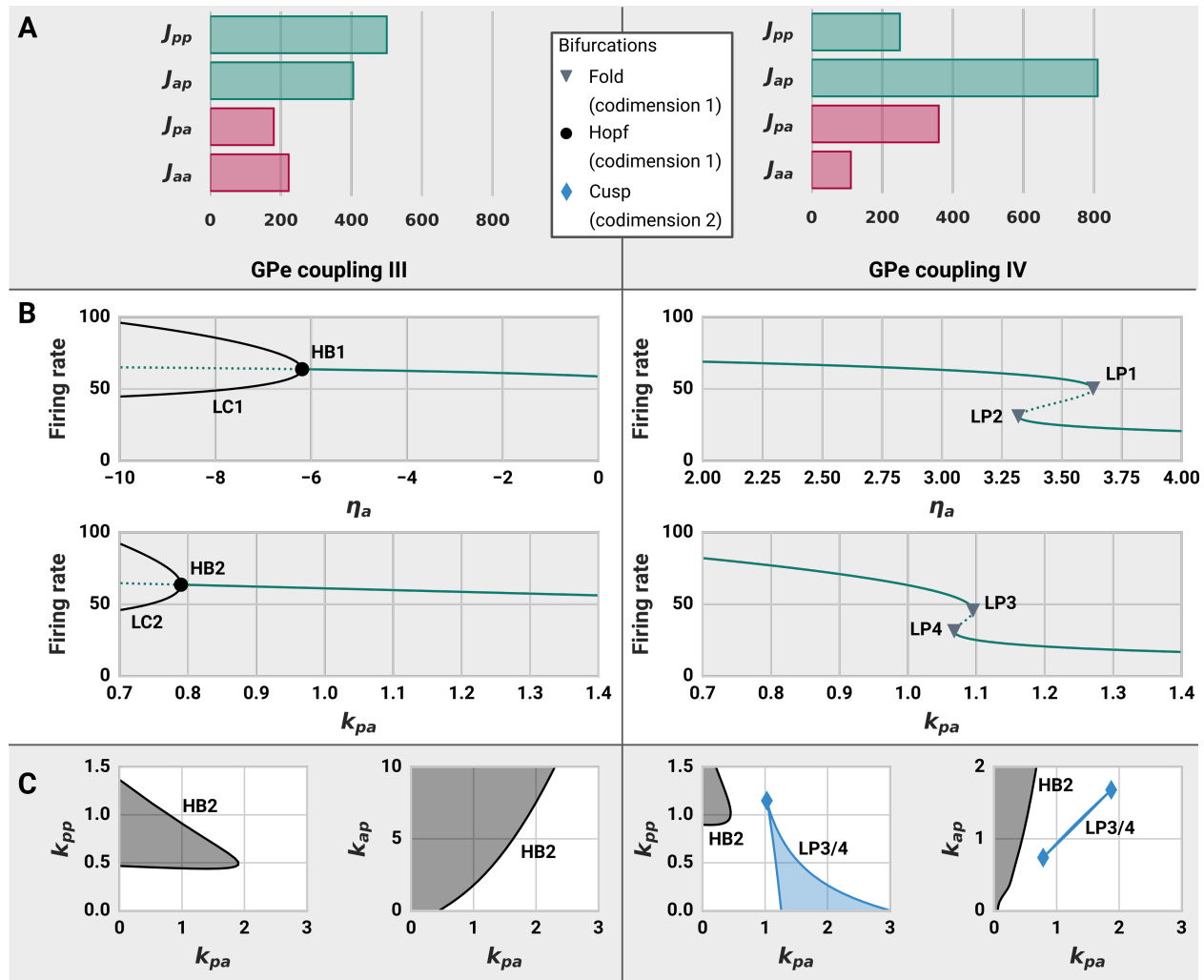
Figure 2: GPe phase transitions induced by changes in the synaptic coupling. A : GPe coupling patterns III ( k_i = 0.9 , k_p = 1.5 ) and IV ( k_i = 1.8 , k_p = 1.5 ) and a legend of all bifurcations reported in this figure. B : Bifurcation diagrams for 1D parameter continuations in \eta_a and k_{pa} . Solid lines represent stable solution branches whereas dotted lines represent unstable solution branches. For GPe coupling III and \eta_p = 4.8 , reducing \eta_a or k_{pa} moves the system over a supercritical Andronov-Hopf bifurcation (HB1) from which a stable limit cycle emerges. The black, solid curves show the minimum and maximum limit cycle amplitudes of the GPe firing rate. For GPe coupling IV and \eta_p = 3.2 , two fold bifurcations are found in both \eta_a and k_{pa} , allowing for the co-existence of two stable focus branches in a small parameter regime. C : 2D parameter continuations of the Hopf and fold bifurcations in the k_{pp} - k_{pa} and k_{pp} - k_{ap} planes for both GPe coupling patterns. Areas shaded in dark grey represent parameter regimes in which stable oscillations exist, whereas areas shaded in blue represent areas in which two stable focus branches can co-exist (bi-stability).
