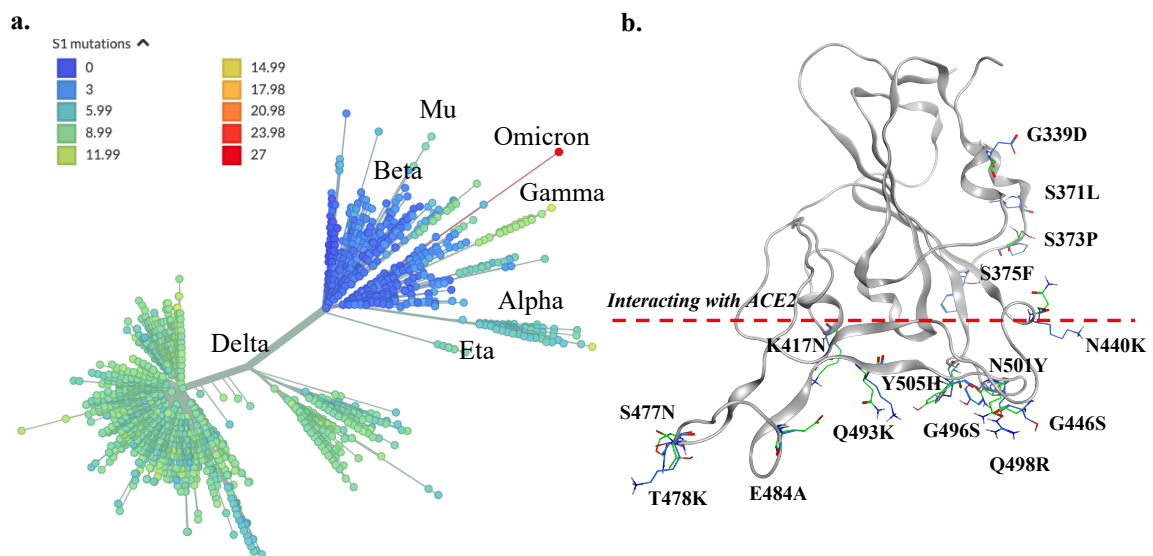
Figure 1. Mutations and the diversity of SARS-CoV-2. (a) The phylogenetic tree of SARS-CoV-2. Major variants are labelled on the graph, and the color of clans is according to the number of spike protein mutations. The tree is generated at https://nextstrain.org . (b) Mutation sites of the receptor binding domain. The residues below the red line are at or near the ACE2 binding interface.
