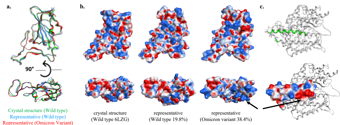
Figure 4. Representative structures and the electrostatic potential surfaces. (a) The representative structures of wild type RBD (blue) and RBD O (red) are superposed to the crystal structure (green). The bottom panel shows the structure alignment for the ACE2 binding interface of RBD. (b) The electrostatic potentials on the RBD/RBD O surface (-5 k B T/e to +5 k B T/e, for colors from red to blue). (c) The RBD binding interface of ACE2
