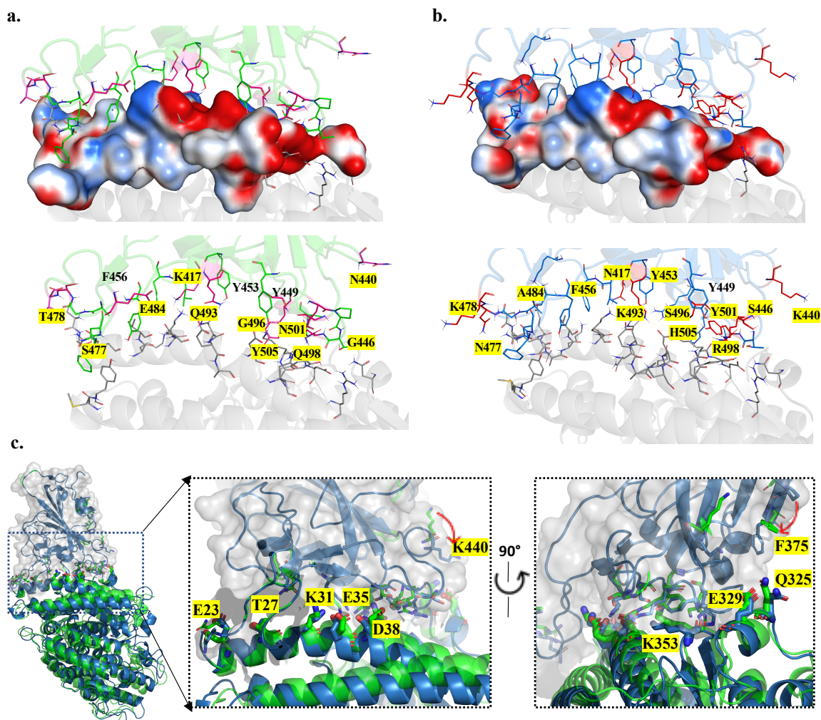
Figure 5. Detailed structures at the ACE2-RBD binding interface. (a) The interface of the wild type ACE2-RBD complex, the amino acids at mutation sites are shown with stick representations. The upper panels show the side chain positions of RBD on the surface of ACE2, where the surface is colored according to electrostatic potentials ( -5 k_B T/e to +5 k_B T/e , for colors from red to blue); lower panel shows the side chains of both ACE2 and RBD. (b) The interactions between ACE2-RBD of the Omicron variant. The figure labeling and coloring scheme are the same as in (a). The amino acids at mutation sites are highlighted with yellow color. (c) The conformation and the positions of ACE2 residues that are in close contact with RBD. The predicted complex model is shown in green color, and the representative model is in blue color. The RBD domain is enclosed by the solvent accessible surface colored in gray. The right panels show enlarged views of the interface in two orientations. The key residue side chains are shown in thicker sticks. Red arrows indicate the major movements of RBD residue side chains.
