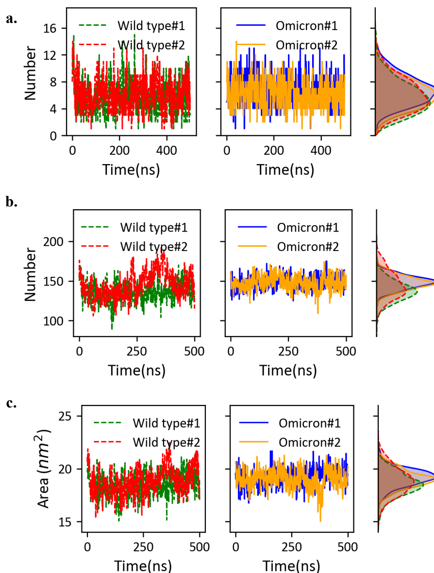
Figure 3. Quantitative analysis of the ACE2-RBD interactions. (a) Hydrogen bonds between ACE2 and RBD/RBD O . The time traces of hydrogen bond numbers observed during the simulations are shown on the left and middle columns. The histograms are shown on the right column to compare the statistics between the wild type system and the Omicron variant system. (b) The number of residue contacts between ACE2 and RBD. (c) The buried surface area due to ACE2-RBD binding. Similar to (a), the histograms are shown to facilitate the comparison in (b, c).
