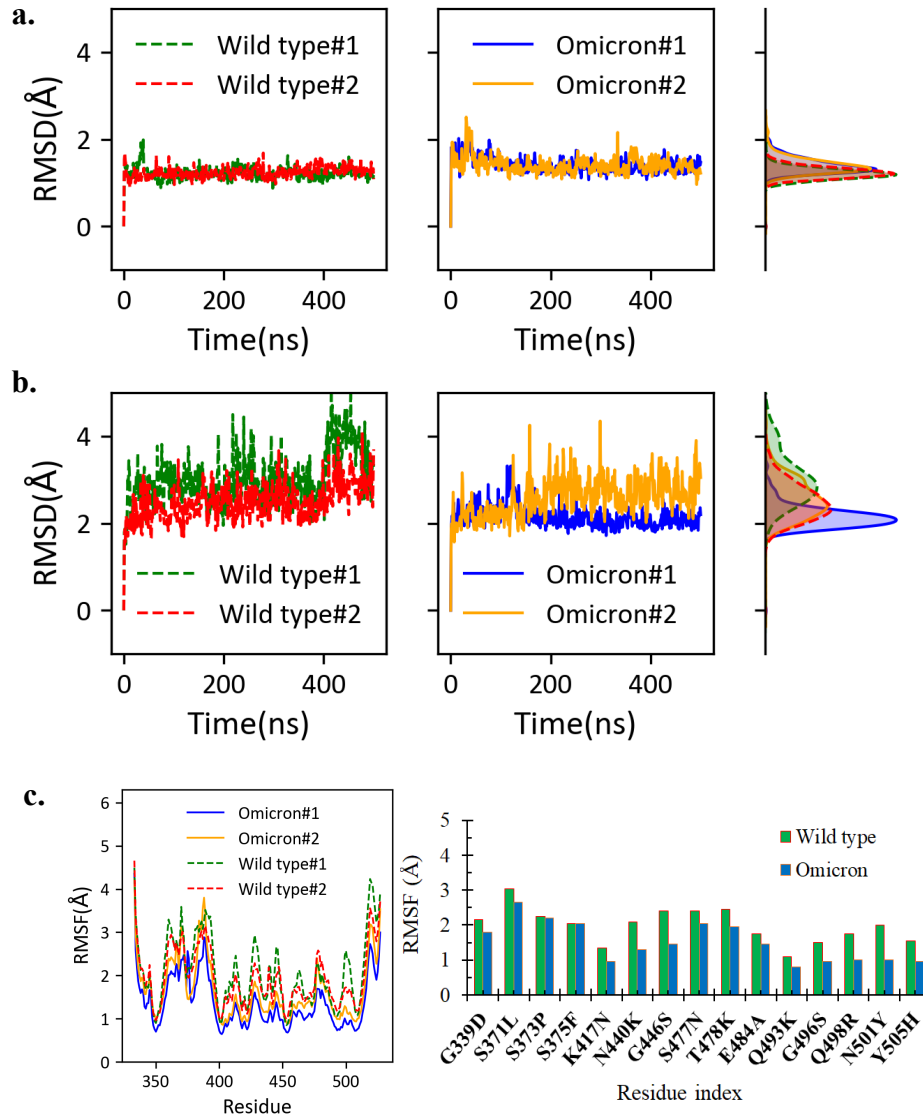
Figure 2. Stability of the RBD and ACE2-RBD complex structures. (a) The RMSD of RBD with respect to the starting structure. The histogram of each RMSD time trace is drawn on the right. (b) The RMSD of the whole complex with respect to the starting complex structure, with the histograms shown on the right. (c) The RBD residue fluctuations. The residue fluctuations for the mutation sites are shown on the right panel. The interactions between ACE2 and RBD are enhanced in Omicron variant. We extracted the hydrogen bonds formed directly between ACE2 and RBD O , and further compared the data to the wild type system (Figure 3). On average, there are 6.5 \pm 2.2
