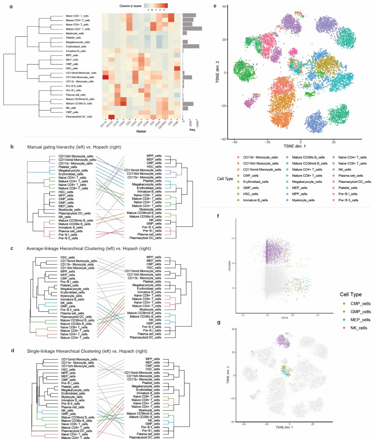
Supplementary Fig 1: treekoR facilities varying cell type hierarchies to enable the measurement of cell types %parent a. A heatmap of the median marker frequencies, clustered using HOPACH, for each cell type as subsetted with manual gating from a healthy human bone marrow sample 38 (top left). b. Tanglegrams comparing two trees to highlight differences in cell type hierarchies: manual gating hierarchy vs. HOPACH clustering; c. average-linkage hierarchical clustering vs. HOPACH clustering; and d. single-linkage hierarchical clustering vs. HOPACH clustering (bottom right). e. A t-SNE plot of the sample, highlighted by the manually gated cell types f. Scatterplot of CD34 vs. CD45RA with only
