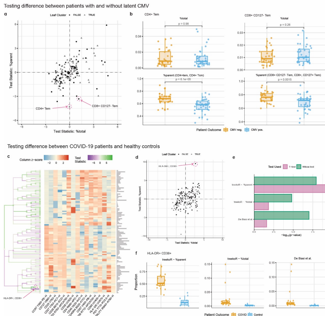
Fig 2: Measuring %parent can provide additional insight over %total. a. Scatterplot of test statistics with the cell clusters in differentiating between latent CMV infection patients. Highlighted clusters are significant using %parent, whilst not significant using %total. b. Comparative boxplot of the proportions of highlighted cell clusters, between patients with CMV and without CMV, with the %total (upper panel) and %parent (lower panel). c. A heatmap generated using treekoR on a CD8+ T cell compartment to predict healthy vs COVID-19, containing a hierarchical tree of cell clusters coloured by the test statistic using the corresponding %total (nodes) and %parent (branches). The heatmap is coloured by the scaled cluster median expression values characterise leaf nodes in the tree. d. Scatterplot of test statistics of each cell cluster with test statistic from using %total (x-axis) vs. test statistic from %parent (y-axis). The HLA-DR+ CD38+ cluster highlighted has a larger test statistic when differentiating between COVID-19 patients and healthy control using %parent than %total. e. Comparison of -\log_{10} of p-values of a HLA-DR+ CD38+ subset for %total, %parent and manually gated proportions from De Biasi et al. from a t-test (pink) and Wilcoxon test (green). f. Comparative boxplot of a HLA-DR+ CD38+ subset, with the %total (upper left panel), %parent (lower panel), and manually gated proportions (upper right panel) between COVID-19 and healthy patients
