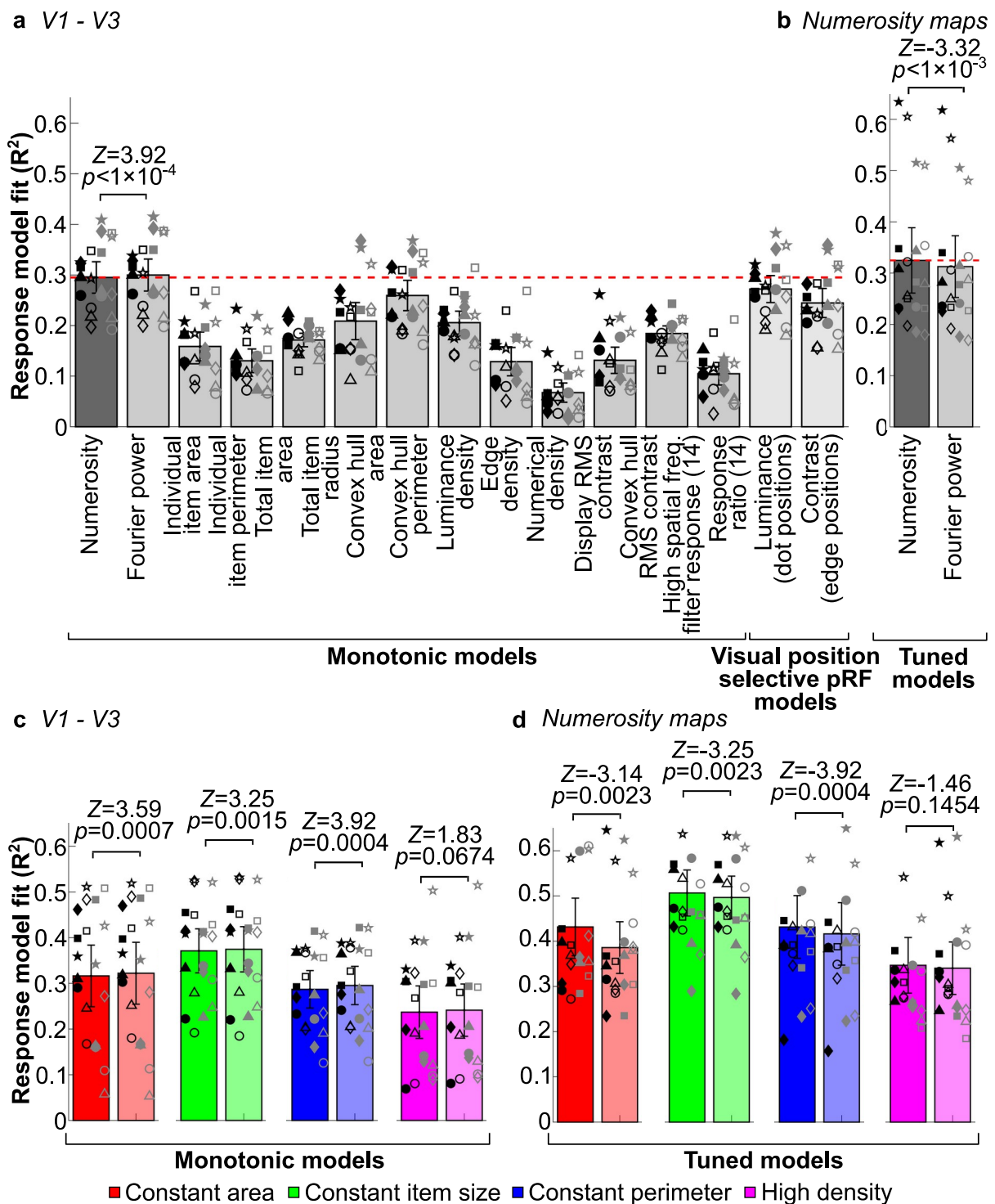
Fig. 4: Responses to aggregate Fourier power predict early visual monotonic responses better than numerosity, but numerosity predicts tuned responses better. a Variance explained by monotonic response models for numerosity and non-numerical visual features, and visual position selective pRF models in V1-V3. b Variance explained by tuned response models for numerosity and aggregate Fourier power in the association cortex numerosity maps. c Variance explained by monotonic response models for numerosity (saturated bars) and Fourier power (unsaturated bars) in V1-V3 in each stimulus configuration. d Variance explained by tuned response models for numerosity and Fourier power in the association cortex numerosity maps in each stimulus configuration. Bar height is the mean variance
