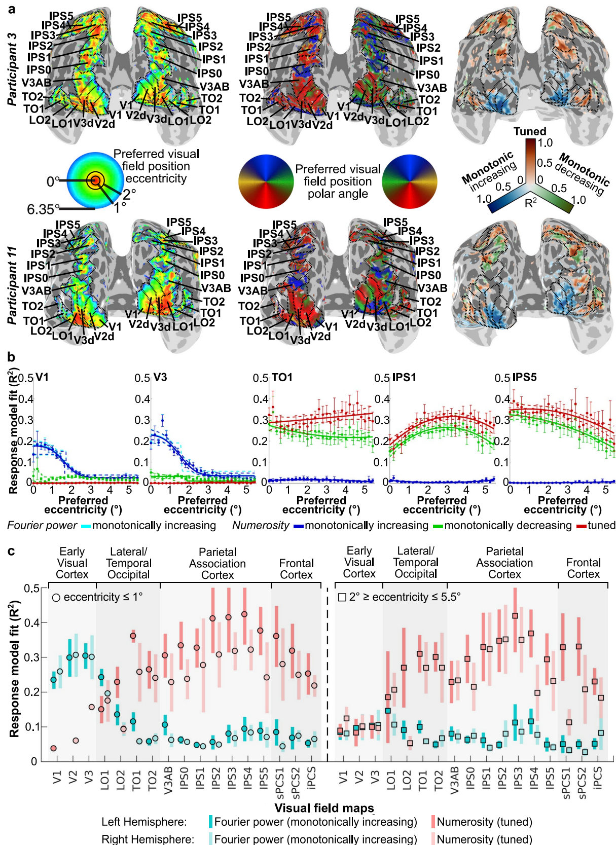
Fig. 2: Relationships between responses to numerosity and visual field position. a Visual position preferences (eccentricity and polar angle, left and middle) and best fitting numerosity model (right, colors) at each cortical location, for two illustrative participants. Dashed black lines and labels show visual field map borders and names respectively. b
