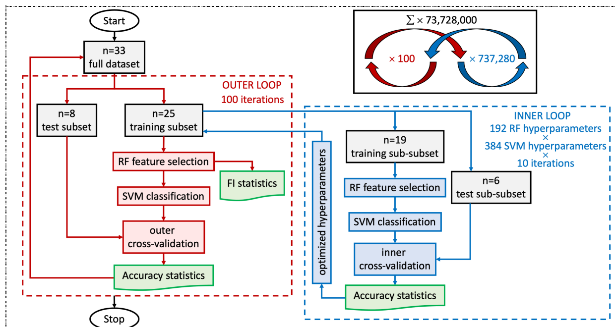
Figure 2. Double cross-validation loop design. Starting in the outer loop: stochastic cross-validation starts with 100 iterations using 25% of data (randomly selected per iteration) for testing. The training subset goes to the inner loop after the train-test split. In the inner loop: split data again just like in the outer loop to obtain training set and validation set for an inner 10 cross-validation iterations with each hyperparameter setting (in total 192 combinations for RF and 384 for SVM, leading to 73,728 combinations with every 10 iterations). Next, we scale training features by subtracting the median and dividing by the inter-quartile range (makes them robust to outliers we identified above). We apply these scaling statistics calculated from the training set also to the test set. Then, we iterate through hyperparameters ( Supplementary Tables 1 and 2 ). RF is used for feature selection. Afterward, the remaining features are used for training the SVM classifier with specific hyperparameter settings. We track the selected features for each run and compute the frequency with which they are selected across iterations for the outer loop. The SVM classifications are validated with the test sub-subset (inner cross-validation). This provides optimized hyperparameter settings from the inner cross-validation loop. Back to the outer loop, we recombine training and validation data (which were separated in the inner loop) - still keeping test data separate. We set hyperparameters to the best settings obtained in the inner loop. Then, we train the model and record results: RF is again used for feature selection, which leads to feature importance (FI) statistics used for the results. Afterward, SVM classifies the remaining features, which are then validated with the test set (outer cross-validation). After this, the next iteration of the outer loop begins.
