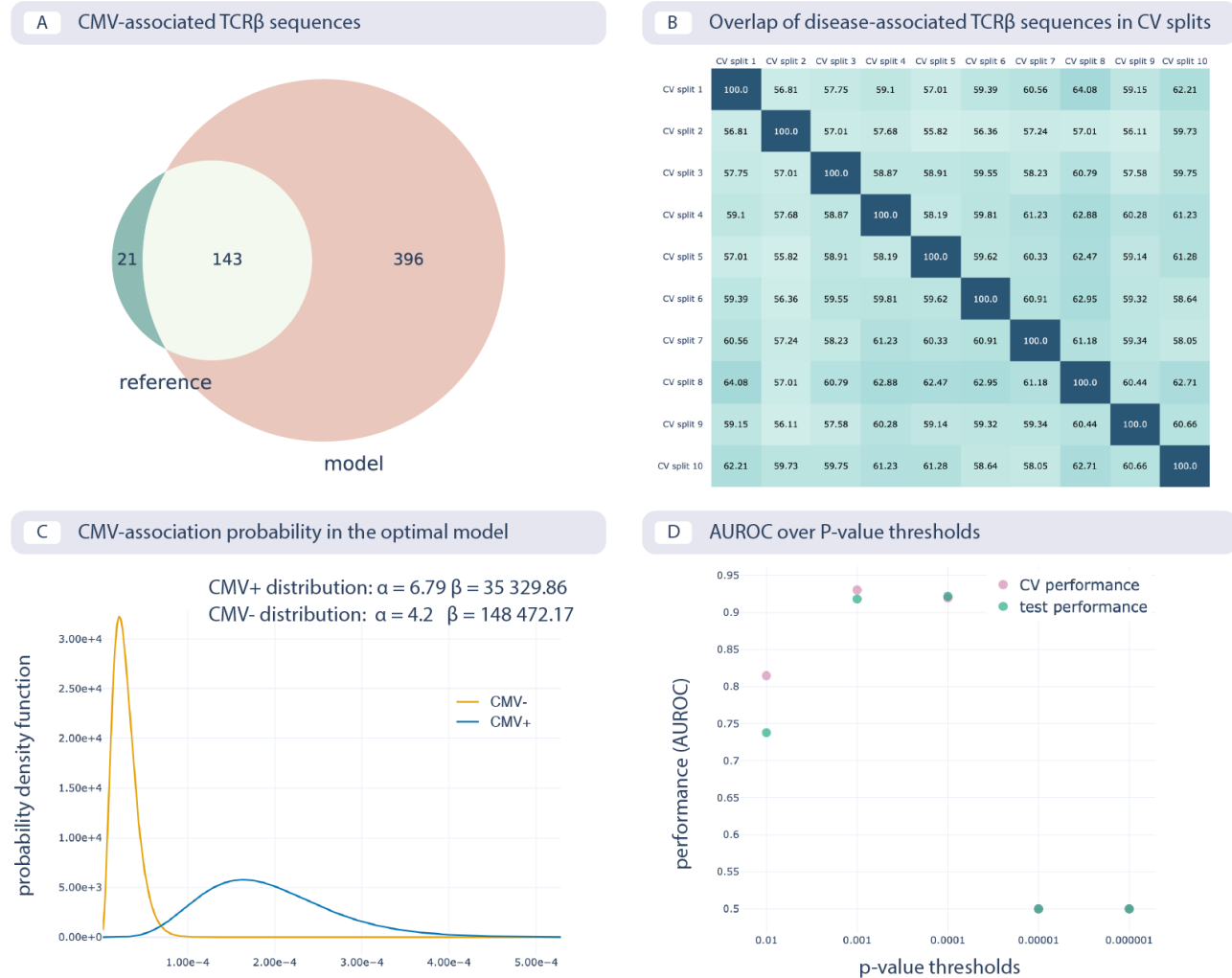
Supplementary Figure 4 | Reproducing the CMV status prediction study by Emerson et al. 6 A. The overlap of the 164 disease-associated TCR \beta sequences (V-TCR \beta aa-J) determined in the original study by Emerson et al., labeled “reference”, with those determined by the optimal model as reproduced here with a p-value threshold of 0.001 (labeled “model”). B. The overlap percentage of disease-associated TCR \beta sequences for the optimal model with the p-value threshold of 0.001 between different data splits in 10-fold cross-validation (between 50% and 65% overlap). C. The probability that a TCR \beta sequence is CMV-associated follows a beta distribution estimated separately for CMV positive and negative subjects, which is then used for CMV status prediction of new subjects. D. Area under the ROC curve (AUROC) over p-value thresholds in training data (average AUROC over 10 cross-validation splits) and test data (AUROC in cohort 2).
