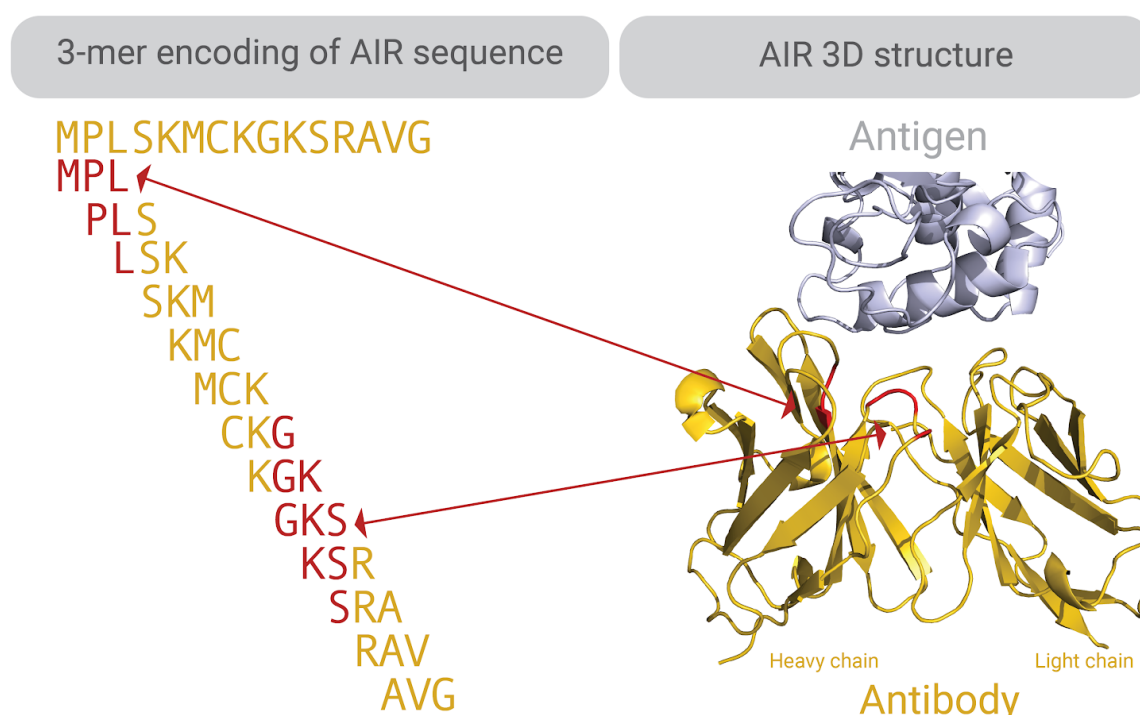
Supplementary Figure 3 | An example of how a k-mer encoded AIR (here antibody) sequence may map the antibody 3D-structure (Protein Data Bank (PDB) ID: 2DQC 78 ). K-mers are subsequences of length k . Through ML, we can learn, for example, which k-mers are important for determining antigen specificity (color-coded in red). These k-mers may map to regions of the (CDR3) sequence that are in contact with the antigen. 16 3D visualization of the antibody-antigen structure was carried out in Pymol 79 .
