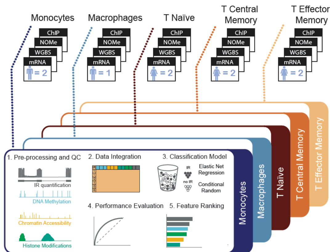
Figure 6 Experimental design and workflow to determine regulators of IR. Raw high-throughput data were processed for each biological replicate and amalgamated by cell type from the indicated number of samples (n). The output was used for feature extraction: IR events were treated as a binary outcome and we trained an Elastic Net (EN) regression model and a conditional Random Forest model with a total of 46 sequence-based and epigenetic features. Using feature ranking, we identified the factors that were most strongly associated with IR outcomes and compared the performances of both modelling strategies. These steps were repeated for each cell type.
