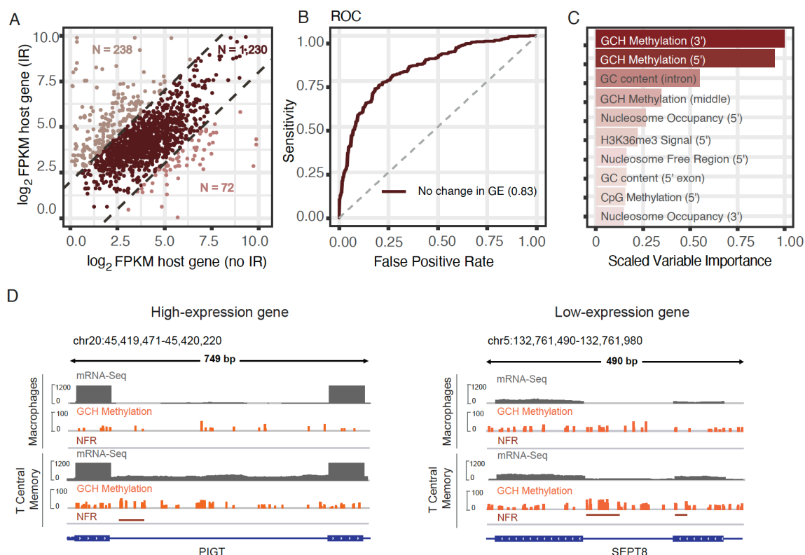
Figure 9 Analysis of introns from genes with non-differential expression levels. (A) Scatter plot of host gene expression for introns that change their IR status. (B) ROC curve indicating the performance of a conditional RF model fitted on the data from non-differentially expressed genes (GE, gene expression). (C) Ranking of the features based on the scaled variable importance scores. (D) Integrative Genomics Viewer (IGV) plots revealing higher density and hypermethylation levels of GCH sites in the splice site regions of differentially retained introns in both highly- and lowly- expressed gene examples (NFR – Nucleosome Free Region, GCH Methylation – methylation levels of GC dinucleotides followed by any nucleobase except guanine).
