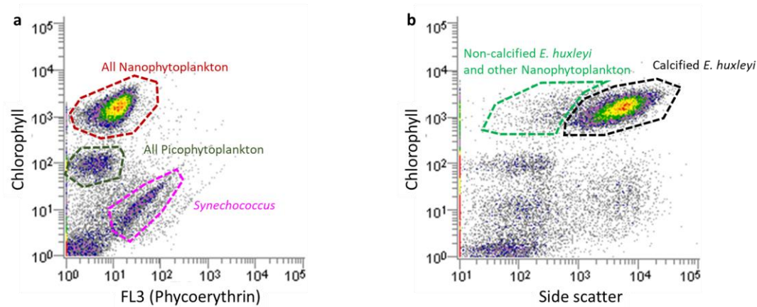
Figure S1. Gating strategy for flow cytometry analysis of natural phytoplankton communities. (a) Example cytogram that contains a mixture of Nanophytoplankton (red), Picoephytoplankton (green) and Synechococcus (pink). Populations were identified based on their different chlorophyll and phycoerythrin content. (b) Calcified E. huxleyi was identified based on the high side scatter caused by the coccoliths that adorn the cells.
