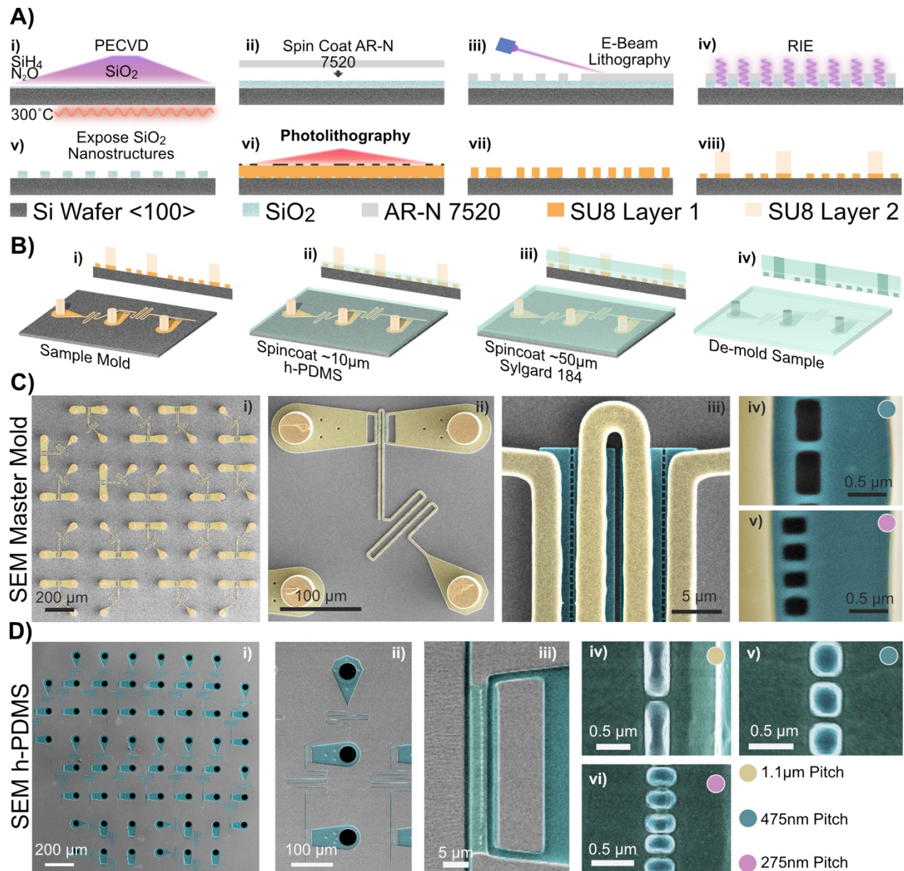
Figure 2: Master Mold and h-PDMS Devices (A) Mix and match lithography process for master mold fabrication: i) Plasma Enhanced Vapor Deposition (PECVD) of 360nm of \text{SiO}_2 on a \langle 100 \rangle silicon wafer; ii) Spin coat the same thickness of E-beam compatible photoresist; iii) Expose the photoresist and remove uncrosslinked material; iv) Reactive ion etch to remove exposed \text{SiO}_2 with the Si wafer acting as an etch stop; v) Strip the remaining photoresist and clean the sample for further processing; vi) The two subsequent layers are made using conventional photolithography where SU8 is exposed through a photomask; vii) The first SU8 layer is 2 \mu\text{m} thick
