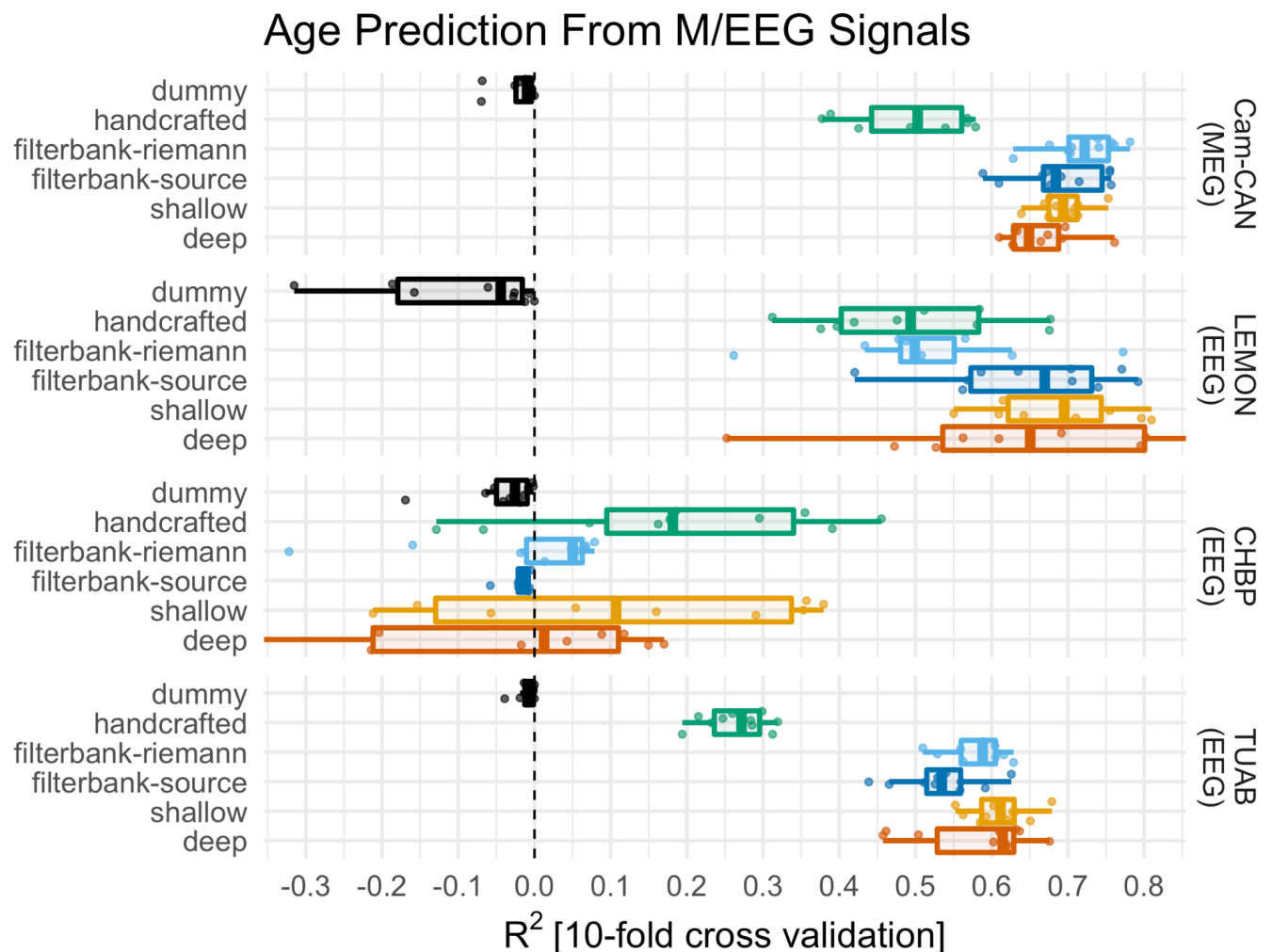
Fig. 3. Age prediction benchmarks across M/EEG datasets ( R^2 score). Generalization performance was assessed by 10-fold cross-validation and the R^2 score for five machine learning strategies compared against a dummy model (rows) and four datasets (panels). Across datasets, dummy models were mostly well-calibrated with R^2 scores close to zero. The LEMON dataset was one exception as dummy scores were systematically worse than chance, which can be explained by the bimodal age distribution (cf. Fig. 2), rendering the average age a bad guess for the age. The 'handcrafted' benchmark delivered moderate but systematic prediction success across all datasets. The two filterbank models performed well across datasets with similar performances, markedly higher than for the 'handcrafted' approach. The only exception was the CHBP benchmark for which neither the filterbank nor the deep models delivered useful predictions. Note that here, for the 'filterbank-source', a single fold with an abysmal R^2 score of -0.15 was obtained (x limits constrained to a range between -0.3 and 1.0). Overall, the deep learning benchmarks performed similarly to the filterbank models.
