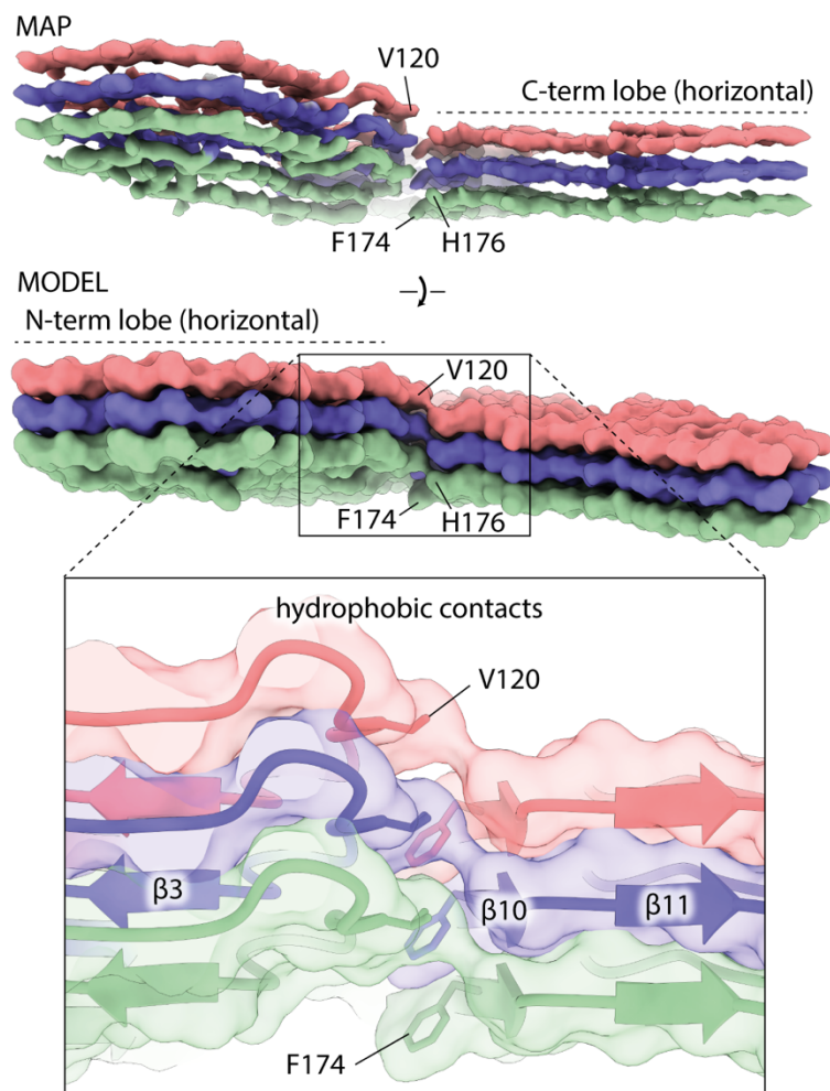
Fig. 3. Staggering of the N- and C-terminal lobes in the RML prion fibril. Top, cryo-EM density (MAP) and solvent-excluded surface (MODEL) of three rungs, with indicated side chains that connect to form the inter-lobe contacts. The F174 and H176 residues are better visible in the MAP and MODEL views, respectively. Bottom, magnified view of the staggered interactions (hydrophobic contacts) shown with transparent surface, main chain as ribbon and selected interacting residues as sticks.
