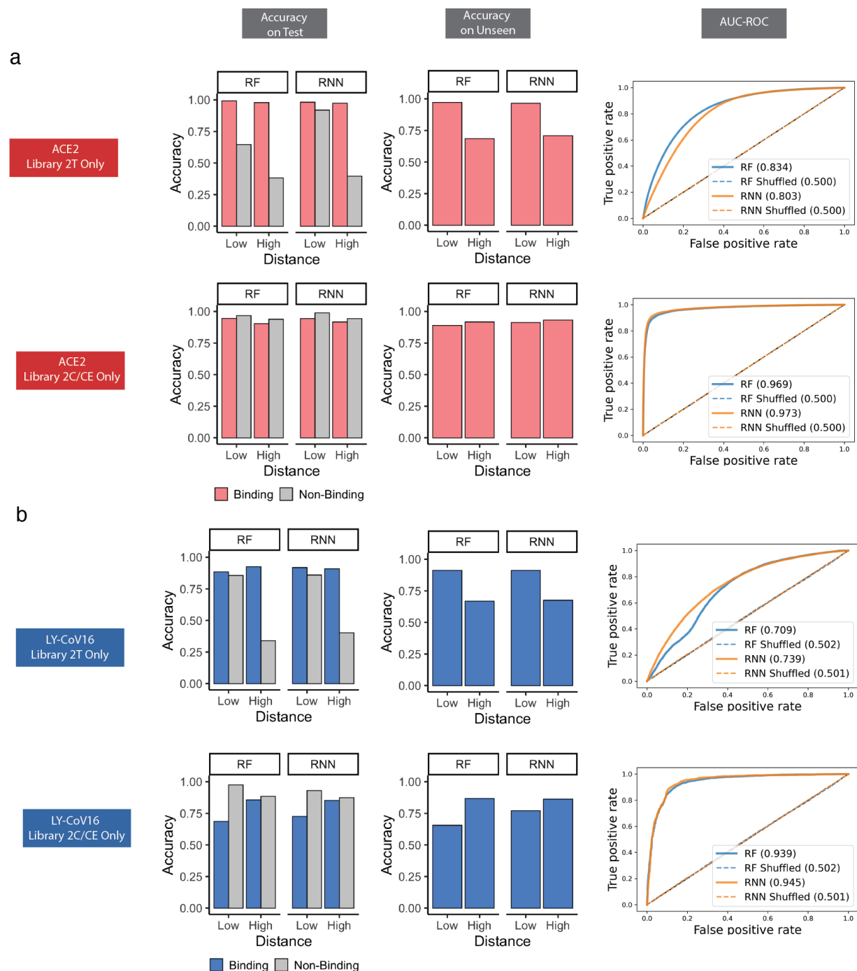
Supplementary Figure 3. Accuracy and ROC curves for models trained on data from low and high distance libraries. a, b, The training data for ACE2 or LY-CoV16 were split into two subsets to train supervised machine learning (Random Forest, RF) and deep learning (recurrent neural network, RNN) models. Library 2T training data contained only sequences that were \leq ED_3 and Library 2C/CE training data contained only sequences that were \geq ED_4 from original Wu-Hu-1 RBD. The models then performed classification on the entirety of the held-out test data, and the unseen data were removed during balancing. Low and high distance sequences are defined as those \leq ED_5 and \geq ED_6 from Wu-Hu-1 RBD, respectively. Model performances are evaluated by accuracy and AUC-ROC.
