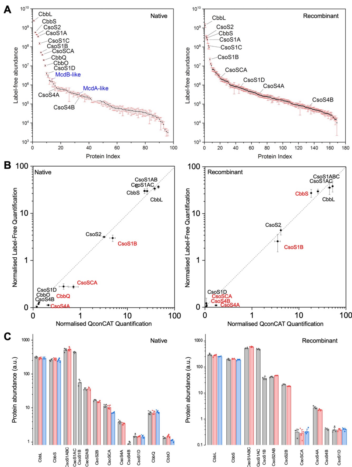
Figure S4. Evaluation of QconCAT and label-free quantification. (A) Protein index of all recognized proteins in label-free quantification. In native carboxysome samples, McdAB-like proteins are both detected. The full protein list provided in Supplemental File; (B) Comparison of QconCAT and label-free quantification. Quantification was normalized to equal total protein quantity. Proteins with the abundance difference greater than 30% from average are labelled in red; (C) Quantification of all QconCAT candidate peptides for H. neapolitanus carboxysomes. Overall good agreements are found within candidate peptides for same protein with the exception of peptide 3 of CsoSCA ( 34 \pm 4 % lower than the other two) and CbbO ( 21 \pm 3 %) in native carboxysome samples.
