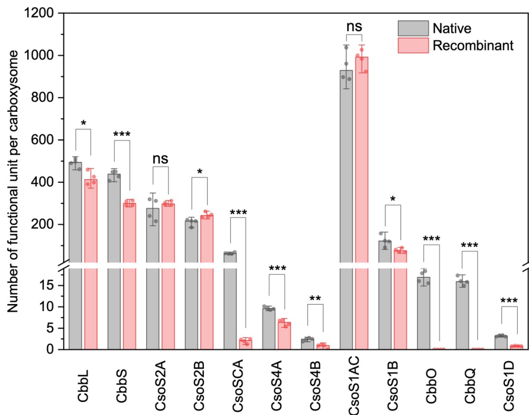
Figure 2. Stoichiometry comparison of native and recombinant carboxysomes. ns, as no statistical significance; *, p < 0.05 ; **, p < 0.01 ; ***, p < 0.001 using two sample t-test, equal variance not assumed (welch correction). Data are shown as mean \pm SD from four biological replicates.
