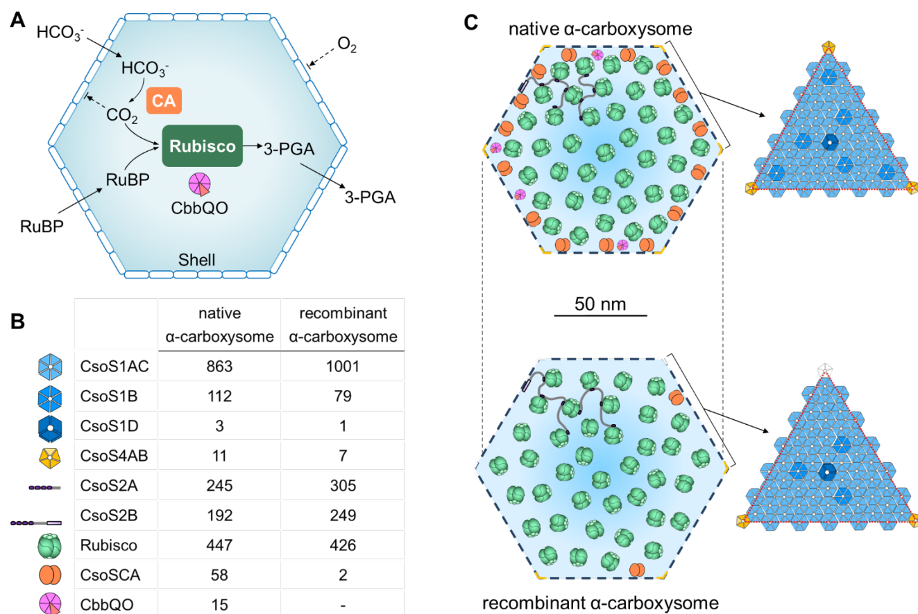
Figure 3. Structural models of H. neapolitanus α-carboxysomes. (A) Schematic of the pathways of carbon fixation in the α-carboxysome, including Rubisco activases CbbQO as the structural components; (B) The stoichiometry of each structural component within native and recombinant α-carboxysome (see Table 1 and 2). (C) Schematic of native and recombinant α-carboxysome structures and shell organizations. The numbers of proteins do not represent actual abundance and is only for illustration purposes.
