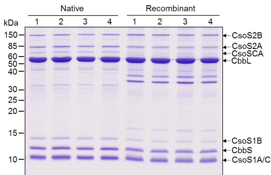
Figure S3. SDS-PAGE of purified carboxysomes from H. neapolitanus and E. coli with four biological replicates prepared for quantification by QconCAT mass spectrometry. 10 µg proteins are loaded per well.
