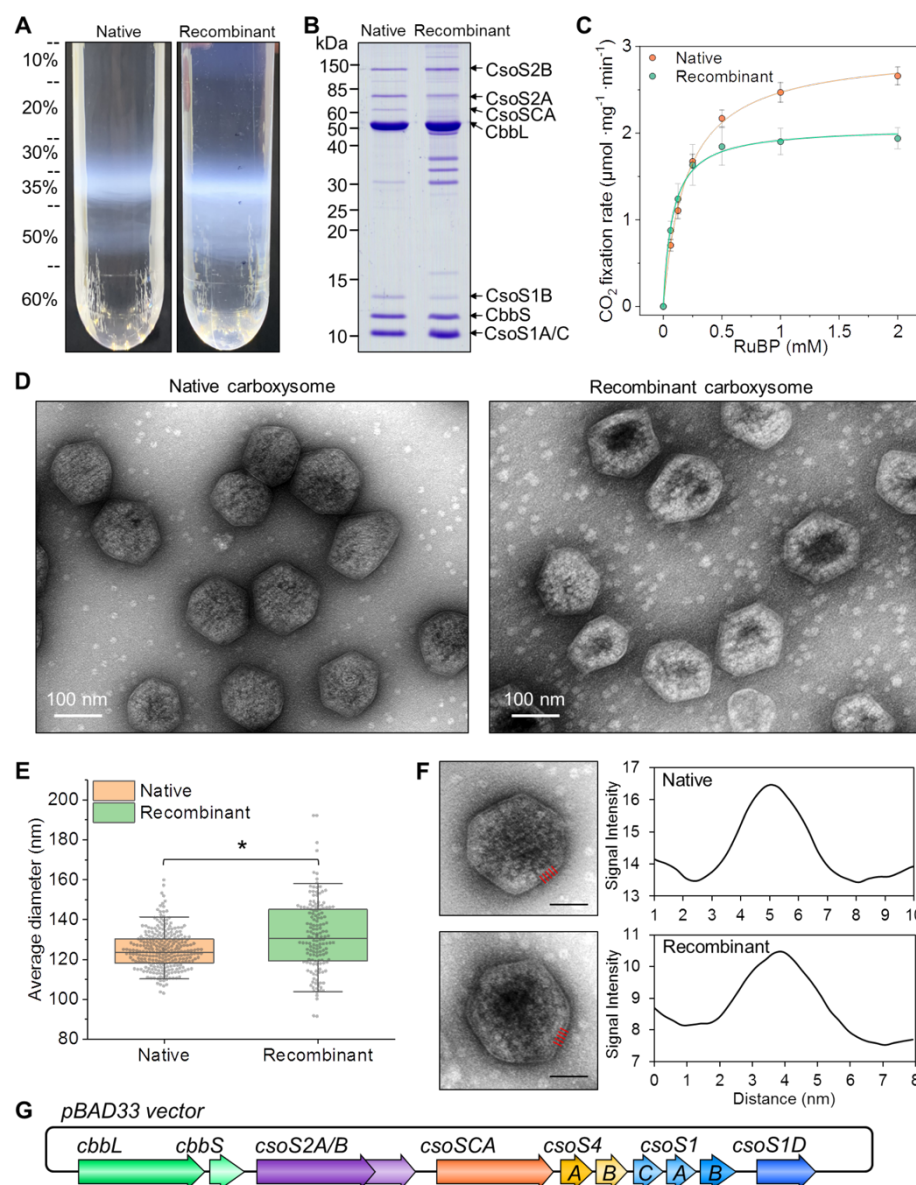
Figure S1. Purification and characterization of native and recombinant α-carboxysomes from H. neapolitanus and E. coli . (A) Sucrose gradient for carboxysome fractions. The milky band between 35%-50% sucrose fraction interface consists of enriched carboxysomes; (B) SDS-PAGE of purified carboxysomes isolated from four replicate batches of culture showing the majority bands of α-carboxysome proteins; (C) Carbon-fixation kinetics as a function of the RuBP concentrations revealed that native and recombinant carboxysomes possess V_{max} at 2.96 \pm 0.09 and 2.07 \pm 0.12 \mu\text{mol} \cdot \text{mg}^{-1} \cdot \text{min}^{-1} and K_{m(\text{RuBP})} at 0.20 \pm 0.02 and 0.08 \pm 0.02 mM, respectively. Data is shown as mean \pm SD from four independent biological replicates; (D) TEM image of purified native and recombinant carboxysomes; (E) Boxplot distribution for diameters of purified native and recombinant carboxysomes, at 124.6 \pm 9.6 nm ( n = 272 ) and 131.8 \pm 18.0 nm ( n = 152 ), respectively. Significant difference of average diameter was confirmed with student t-test ( p < 0.05 ); (F) Analysis on the shell thickness of native and recombinant α-carboxysomes. The shell thickness of native and recombinant α-carboxysomes is 5.3 \pm 0.6 nm and 5.5 \pm 0.8 nm, respectively ( n = 100 ), implicating the single-layer shell architecture. The profile region for measurements were marked by red lines (Scale bar = 50 nm); (G) Recombinant α-carboxysome expression cassette containing cso operon and cbbL/S , plus BMC-T protein encoded gene csoS1D in the pBAD33 vector.
