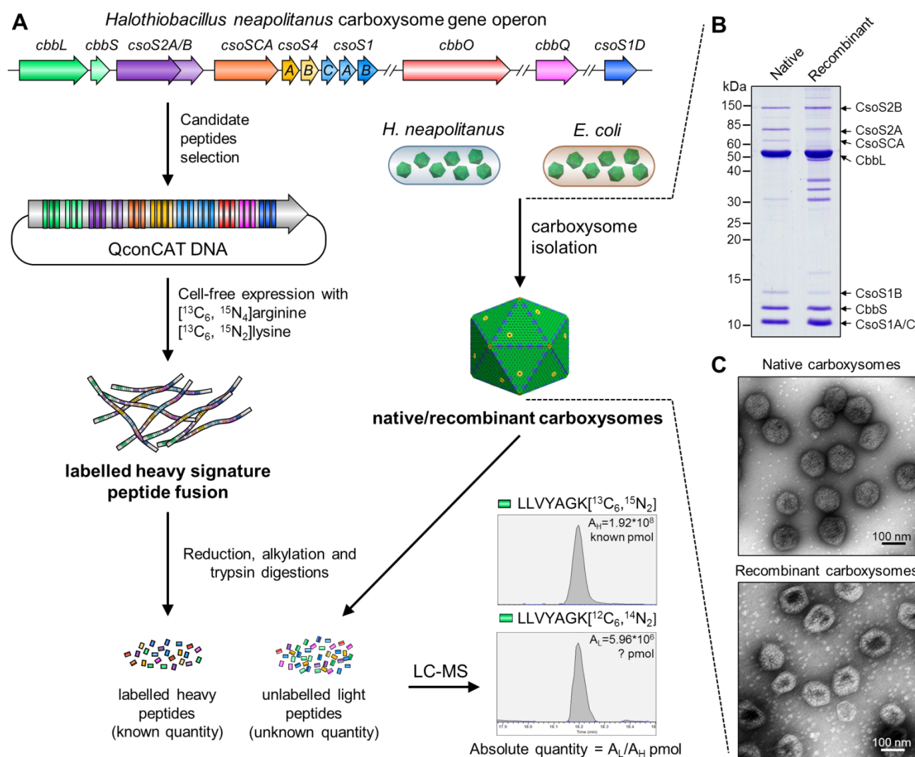
Figure 1. Schematic overview of QconCAT strategy. (A) QconCAT DNA fragment was designed from selected gene sequences from the H. neapolitanus operon that expresses \alpha -carboxysome proteins. The stable isotopes ([ 13 C 6 , 15 N 4 ] arginine and [ 13 C 6 , 15 N 2 ] lysine) labelled QconCAT peptide fusion was expressed via a cell-free system, purified and quantified and added to four replicates samples of isolated native/recombinant \alpha -carboxysomes from H. neapolitanus and E. coli . The absolute quantity and stoichiometry of unlabelled signature peptides for carboxysomal proteins were calculated by LC-MS analysis. One signature peptide for CbbQ, LLVKAGK was shown here as an example. (B) SDS-PAGE of isolated native/recombinant \alpha -carboxysomes showing the majority bands of \alpha -carboxysome proteins. (C) EM images of isolated native/recombinant \alpha -carboxysomes.
