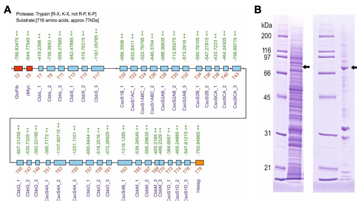
Figure S2. Structure and expression of the H. neapolitanus carboxysome QconCAT. (A) Schematic representation of the quantification concatamer, for quantification of proteins of interest. 35 peptides in QconCAT are represented by blue boxes. Values for the [M+2H^{2+}] m/z peptide ions for the unlabeled QconCAT are aligned above each peptide (green text). The non-target quantification peptides (GluFib and cMyc) and the hexa-histidine tag for QconCAT purification are shaded in red and orange, respectively. (B) SDS-PAGE analysis of QconCAT expression and purification. The coding sequence of QconCAT peptide was sub-cloned into the cell-free expression vector pEU-E01-MCS (left). QconCAT was prepared by wheat germ cell-free synthesis in the presence of [^{13}C_6, ^{15}N_4] arginine and [^{13}C_6, ^{15}N_2] lysine and purified by virtue of the hexa-histidine tag (right). The QconCAT is denoted by the arrow.
