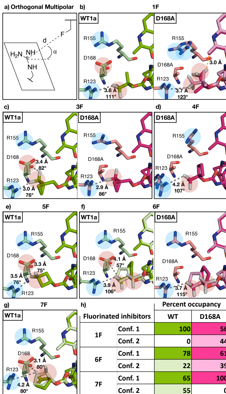
Figure 6. Fluorine specific interactions
