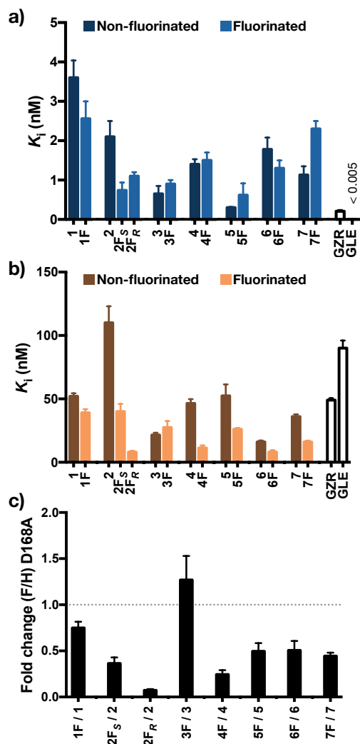
Figure 3. Inhibitor potencies and fold change analyses
