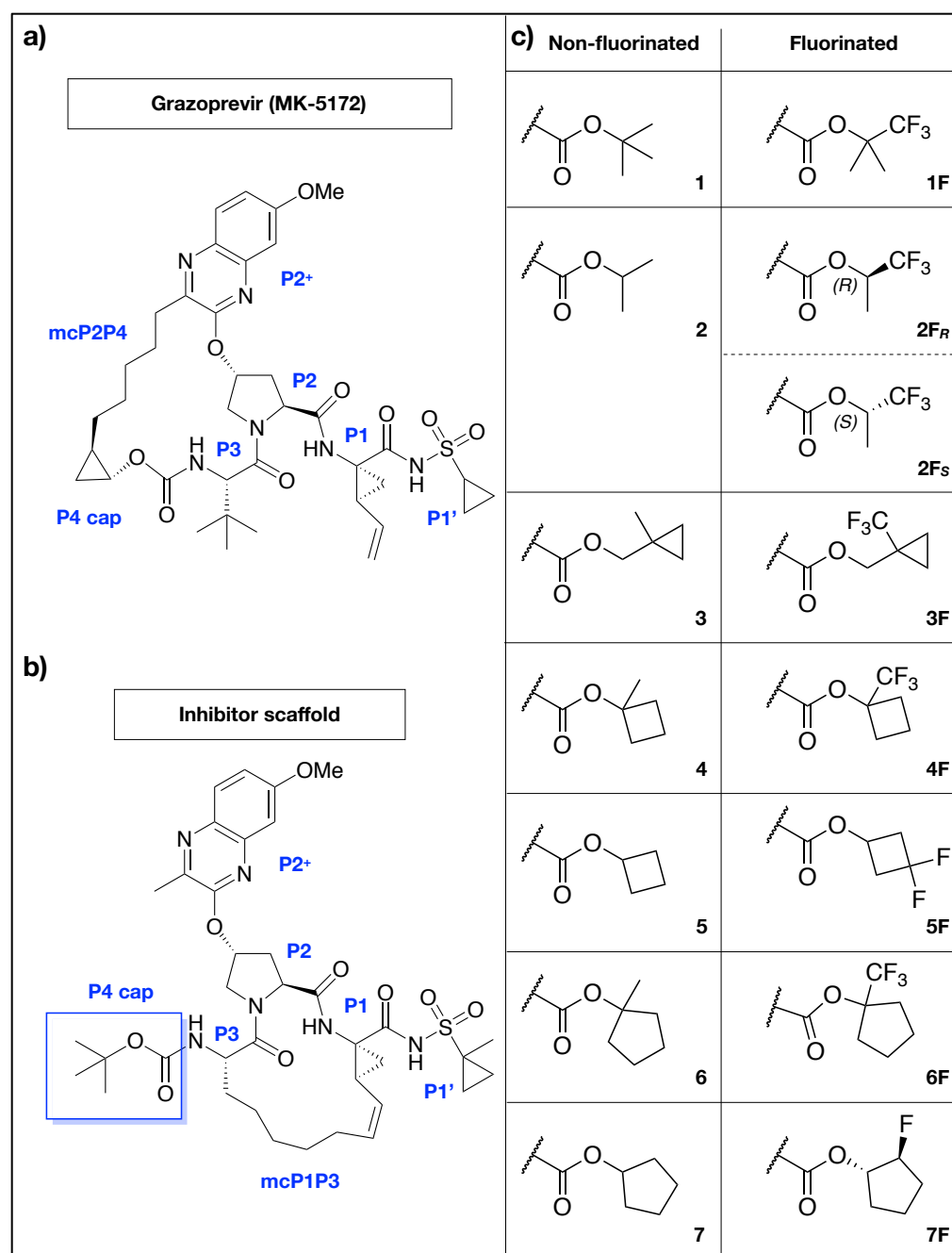
Figure 1. Inhibitor design strategy
