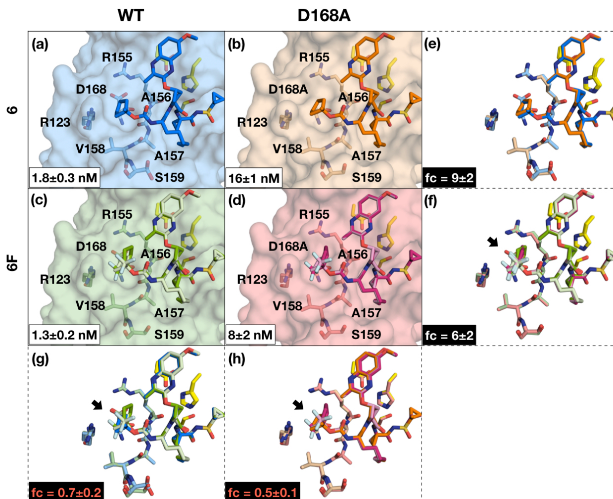
Figure 4. Co-crystal structures of 6 bound to WT1a (a) and D168A (b), and 6F bound to WT (c) and D168A (d). The binding affinity is indicated in the respective panels (a-d). Structural differences in 6 and 6F binding to WT and D168A are shown in (e) and (f) respectively. Structural differences between 6 and 6F binding to WT and D168A is shown in (g) and (h) respectively. The fold change (fc) in binding affinity relative to WT is indicated in the respective panels (e and f). The fold change in binding affinity relative to the parent inhibitor is indicated in (g) and (h) for WT for D168A, respectively. Empty panels indicate no structural differences. The inhibitors and residues of the catalytic triad and S4 pocket (labeled) are shown as sticks. Inhibitors with two conformations are shown in a darker (conformation 1) and lighter (conformation 2) shade, where the darker shade represent the highest occupancy conformation. Arrows in panels e-h indicate structural differences in between the superimposed structures.
