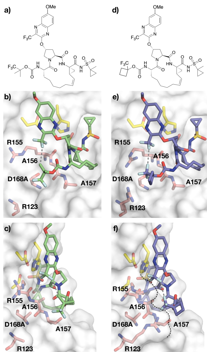
Figure 7. Intermolecular fluorine interaction mediated by R155
