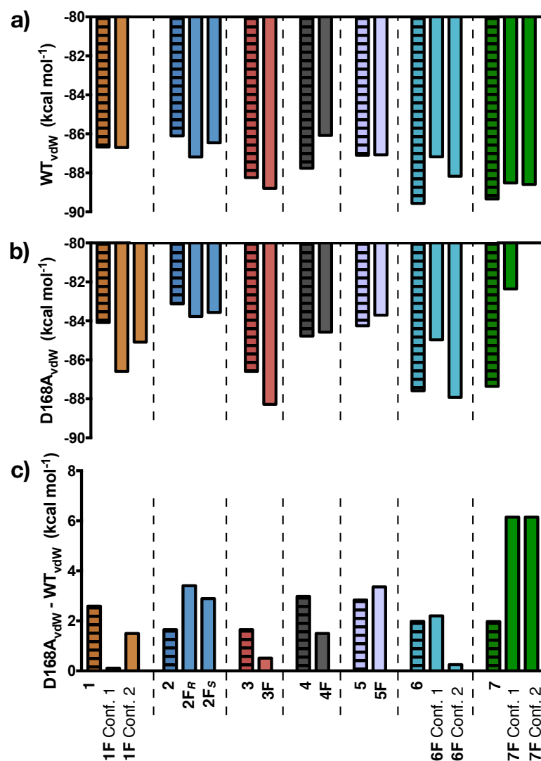
Figure 5. Loss of van de Waals contacts due to the D168A RAS. The total vdW contacts of the inhibitors bound to (a) WT and (b) D168A, and (c) the differences in vdW contacts between WT1a and D168A variant. The striped pattern indicates parent inhibitor data.
