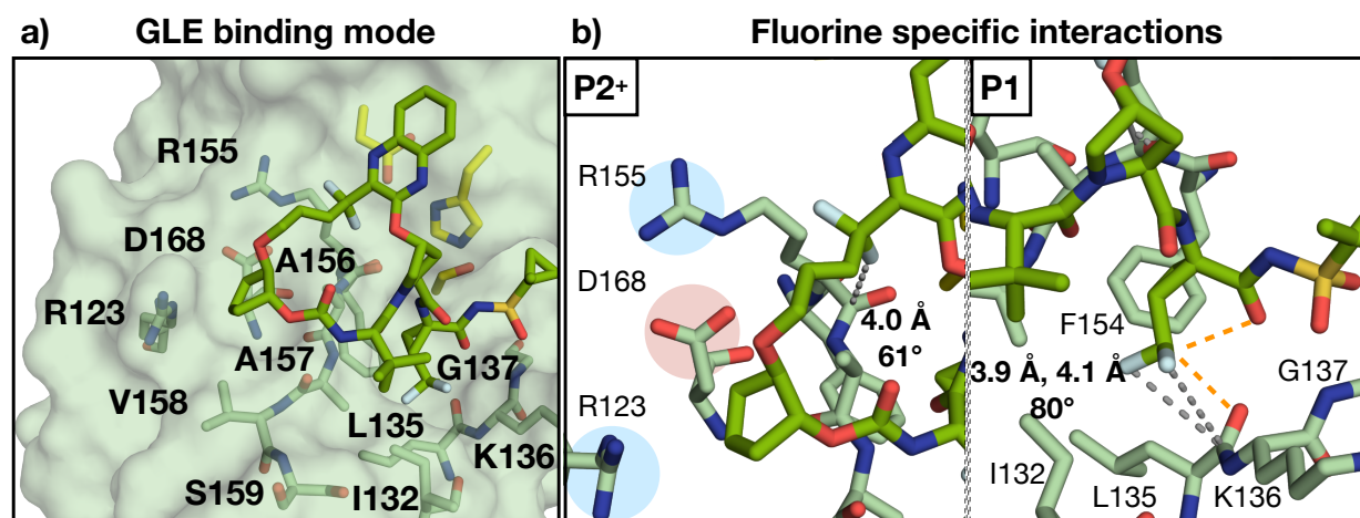
Figure 2. Structural analysis of Glecaprevir
