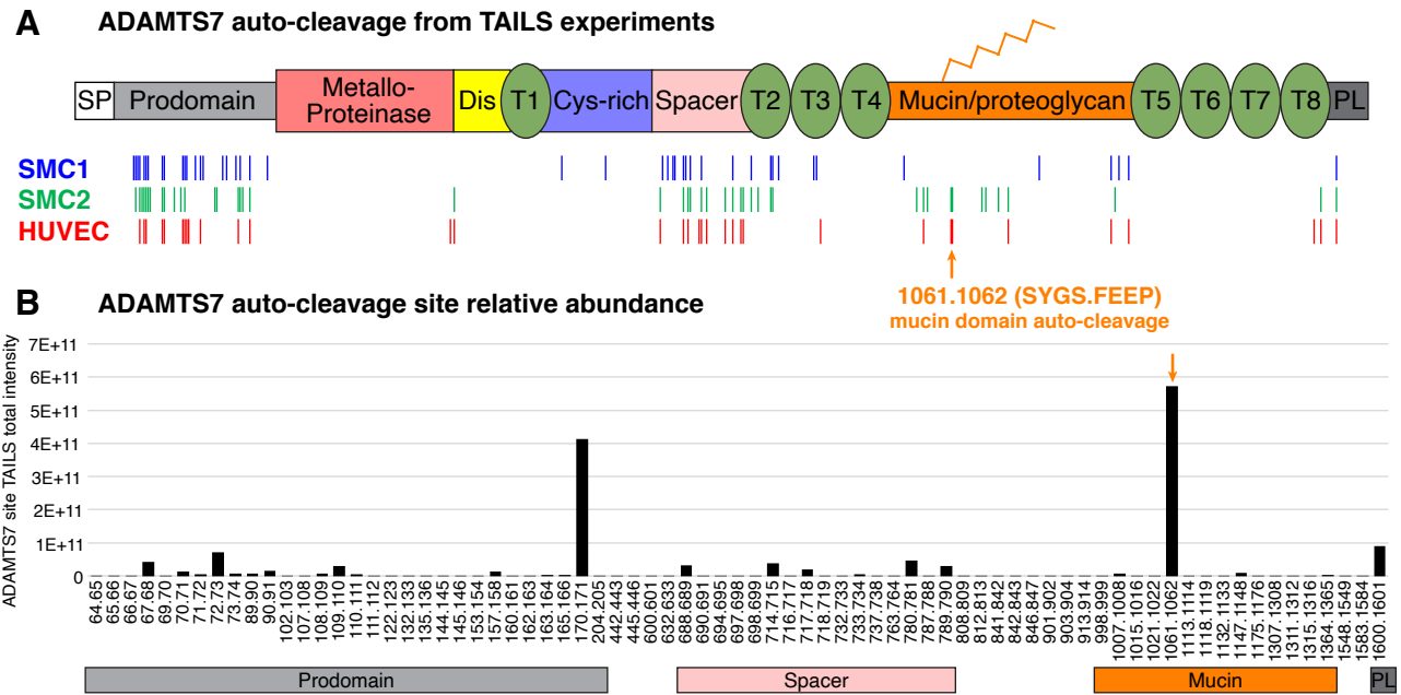
FIG. 1. ADAMTS7 auto-cleavage sites detected in TAILS experiments. A, ADAMTS7 protein domains and locations of the TAILS significantly regulated WT/EQ peptides indicating auto-cleavage events. Abbreviated ADAMTS7 domains: signal peptide (SP), disintegrin (Dis), thrombospondin repeats (T), cysteine-rich (Cys-rich), protease and lacunin (PL). B, ADAMTS7 auto-cleavage peptide total intensities pooled from all TAILS experiments to show relative abundance of each event.
