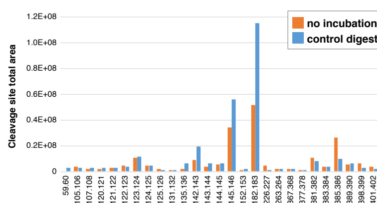
Figure S9 Purified HA-EFEMP1 in vitro cleavage and background cleavage. A, quantitation of semi-tryptic or semi-chymotryptic HA-EFEMP1 peptides from the ADAMTS7 in vitro cleavage assay. A subset of this data at the atypical EGF1 repeat was presented in Figure 7. ADAMTS7 specific cleavage sites at 123.124 and 124.125 are indicated by green arrows. B, background cleavage in purified HA-EFEMP1 within the atypical EGF1 repeat in the absence of enzyme shown by western blot under non-reducing conditions. A region below the full-length HA-EFEMP1 was excised from a parallel Coomassie stained non-reducing gel and sent off for LC-MS/MS identification of EFEMP1 peptides. C, quantitation of semi-tryptic or semi-chymotryptic peptides showing background cleavage from the commercial purified HA-EFEMP1 protein. Background cleavage at positions 123.124 and 124.125 were detected and did not increase in abundance after overnight digestion in control conditions.
