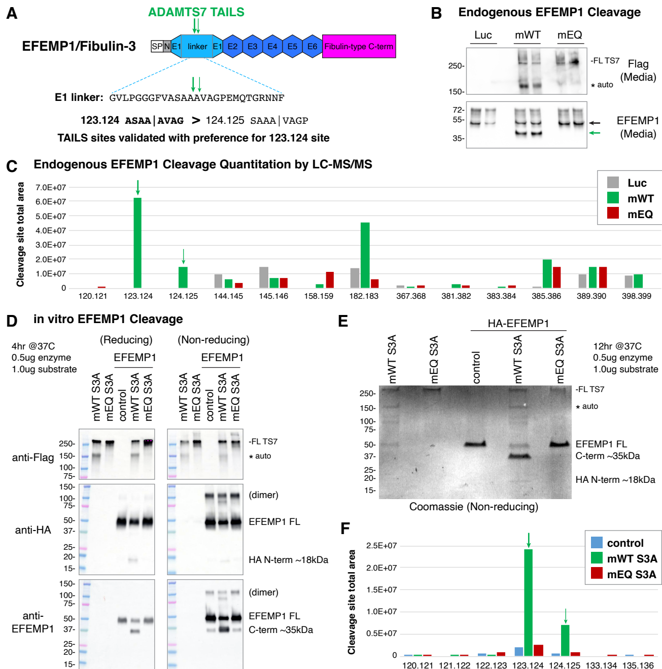
FIG. 5. Validation of TAILS substrate EFEMP1 and cleavage site preference. A, EFEMP1/Fibulin-3 protein domains, amino acid sequence of the atypical EGF repeat linker and location of the ADAMTS7 cleavage sites. Abbreviated EFEMP1 domains: signal peptide (SP), N-terminal region (N), EGF repeats (E). B, concentrated media from HUVEC expressing Ad-Luc, Ad-mWT or Ad-mEQ assessed by western blot under non-reducing conditions. Anti-EFEMP1 antibody recognizes an epitope C-terminal to the ADAMTS7 cleavage sites. C, quantitation of semi-tryptic or semi-chymotryptic peptides from HUVEC media matching novel cleavage sites from the endogenous EFEMP1 protein. The total area was greater for the 123.124 cleavage site compared to the adjacent 124.125 cleavage site. Additional cleavage events observed were also found in the Luc and EQ controls. D, in vitro cleavage of HA-EFEMP1 by purified full-length mouse ADAMTS7 S3A assessed by western blot. The antibodies to the N-terminal HA epitope and C-terminal EFEMP1 epitope recognized the EFEMP1 more strongly under non-reducing conditions. A band at 100kDa under non-reducing conditions is consistent with a purified HA-EFEMP1 dimer, which was also sensitive to ADAMTS7 cleavage. E, overnight digest of HA-EFEMP1 by mouse ADAMTS7 S3A assessed by Coomassie staining. F, quantitation of semi-tryptic or semi-chymotryptic peptides from the atypical EGF1 repeat region from HA-EFEMP1 showing a consistent preference for the 123.124 cleavage site.
