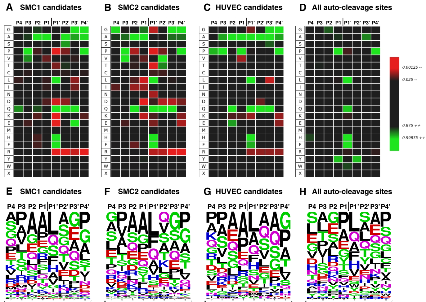
Figure S8 TAILS high confidence substrate site specificity compared with ADAMTS7 auto-cleavage sites. A-D, TAILS candidate substrate cleavage sites and ADAMTS7 auto-cleavage sites analyzed using iceLogo to generate heatmaps adjusted for the abundance of each amino acid in humans. A, SMC1 candidate heatmap ( p < 0.01 , +FC > 1 , n = 179 ), B, SMC2 candidate heatmap ( p < 0.05 , +FC > 1 , n = 200 ), C, HUVEC candidate heatmap ( p < 0.05 , +FC > 1 , n = 118 ). D, the heat map including all unique ADAMTS7 auto-cleavage sites ( n = 75 ) resembles the TAILS high confidence substrates. E-H, Amino acid frequency plots generated by WebLogo showing the similar distribution between experiments, however no amino acid was present more than 30% at any given position at the cleavage site.
