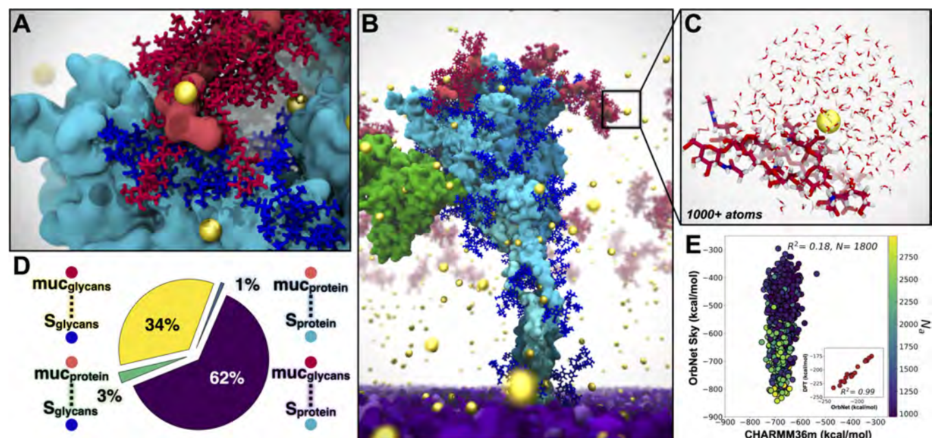
Figure 4: SMA system captured with multiscale modeling from classical MD to AI-enabled quantum mechanics. For all panels: S protein shown in cyan, S glycans in blue, \text{m}_1/\text{m}_2 shown in red, ALB in orange, \text{Ca}^{2+} in yellow spheres, viral membrane in purple. A) Interactions between mucins and S facilitated by glycans and \text{Ca}^{2+} . B) Snapshot from SMA simulations. C) Example \text{Ca}^{2+} binding site from SMA simulations (1800 sites, each 1000+ atoms) used for AI-enabled quantum mechanical estimates from OrbNet Sky. D) Quantification of contacts between S and mucin from SMA simulations. E) OrbNet Sky energies vs CHARMM36m energies for each sub-selected system, colored by total number of atoms. Performance of OrbNet Sky vs. DFT in subplot ( \omega\text{B97x-D3/def-TZVP} , R^2 = 0.99 , for 17 systems of peptides chelating \text{Ca}^{2+} (Hu et al., 2021)). Visualized with VMD.
