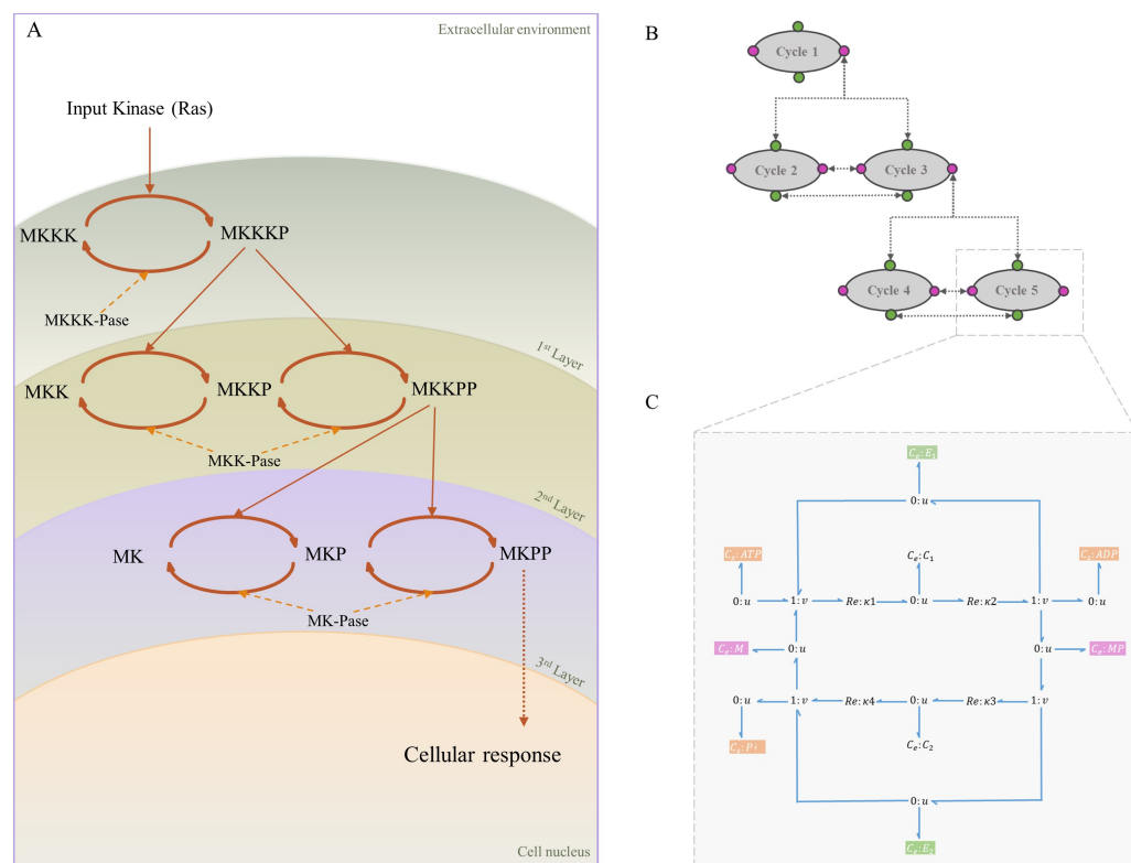
Fig 6. Structure of MAPK cascade. (A) Kinetic representation. The stimulus from the extracellular environment is received (Ras) and transmitted through the MAPK cascade to the cell nucleus. The layers demonstrate the cycles with the same kinase and phosphatase enzymes; (B) MAPK cascade with five modules. Linking species are shown in colours where green corresponds to the linking enzymes and pink corresponds to unphosphorylated/phosphorylated mitogen proteins. Arrows show the links between the modules; (C) The symbolic bond graph model of each cycle. Sources of potential with fixed concentrations ( C_s :ATP, C_s :ADP, and C_s :Pi) are shown in orange. (Same sources of potential within the modules are omitted in (A) and (C) for clarity).
