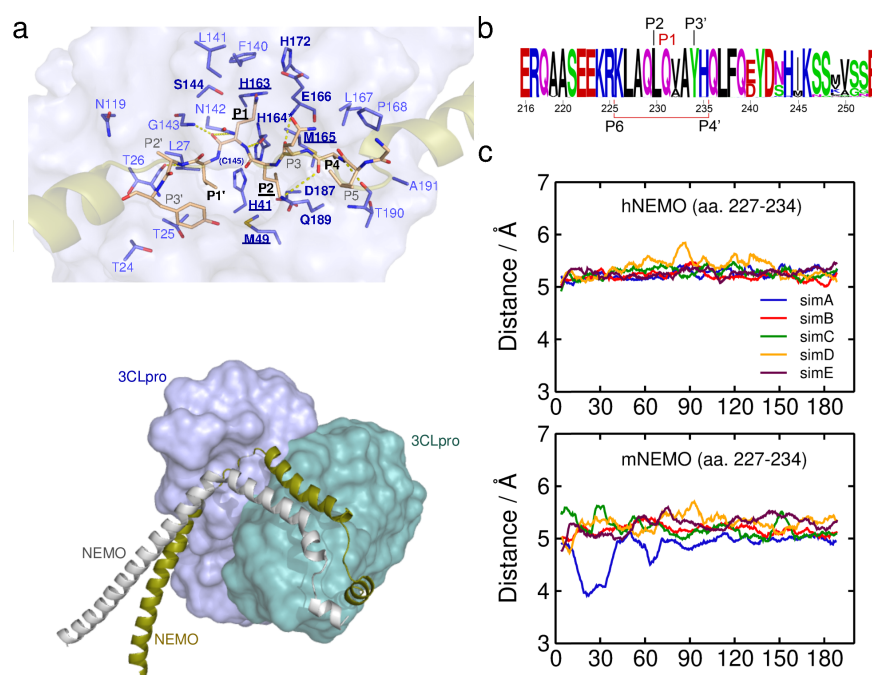
Figure 3. Molecular dynamics simulations of SARS-CoV-2 3CLpro bound to human or mouse
