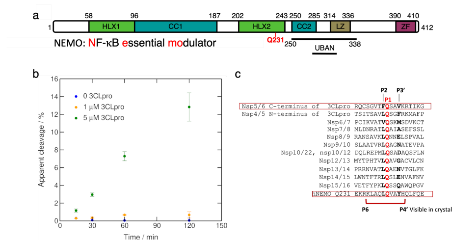
Figure 1. Truncated NF-κB essential modulator (NEMO) is cleaved by 3CLpro in enzymatic assays.
