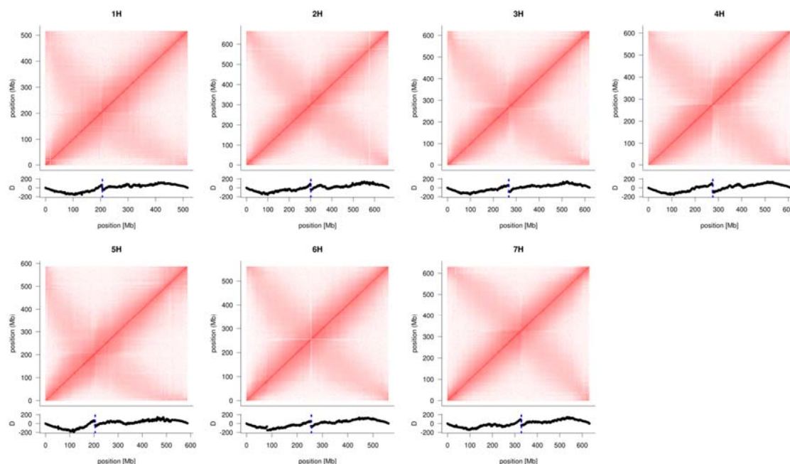
Figure 4: Positioning of centromeres by inspection of Hi-C contact matrices.
