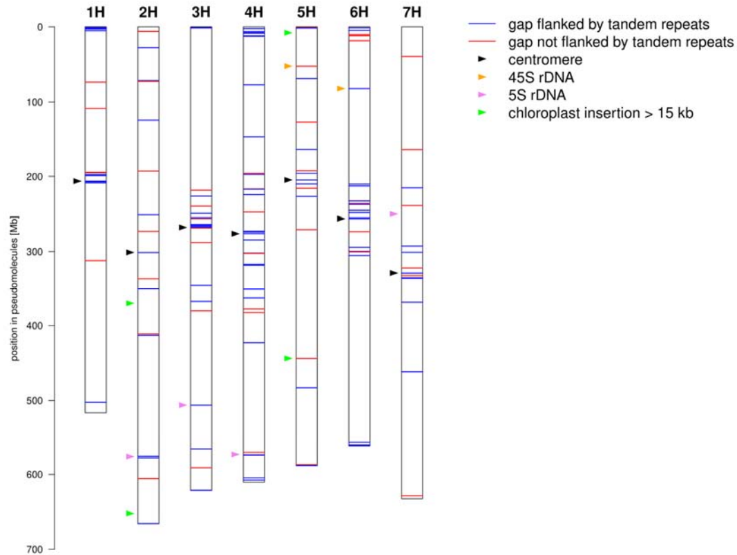
Figure 7: Sequence gaps in the MorexV3 pseudomolecules. The positions of sequence gaps are shown along the pseudomolecules. Gaps are colored according to whether or not at least one of their 1 kb flanking regions contain tandem repeat arrays longer than 500 bp. The positions of centromeres, 5S and 45S ribosomal DNA loci and large (> 15 kb) insertions of plastidal DNA are marked by colored arrowheads.
