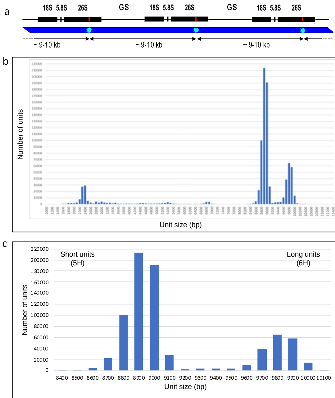
Figure 6: Profiling of 45S rDNA tandem repeats in optical map data. (a) 45S rDNA arrays are composed of clusters of 18S, 5.8S and 26S rRNA genes separated by intergenic spacers (IGS) whose lengths differ between 5H (total unit size ~8.9 kb) and 6H (total unit size ~9.8 kb) rDNA loci. Labelling at DLE-1 site in the 26S rRNA gene (red line) generates a regular pattern in the optical map with a label spacing of ~9-10 kb (bottom). (b) Size distribution of DLE-1-labelled tandem repeats in Morex optical map raw data >150 kb, considering repeat arrays >5 units. The dataset totals 1.09 Tb corresponding to 237-fold coverage of the barley genome. (c) The size category of 8,400-10,100 bp belongs to 45S ribosomal DNA.
