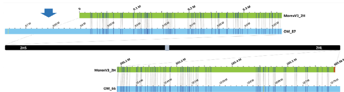
Figure 2. Alignments of the termini of the 2H optical map and sequence assembly reveal missing sequence. The optical map (blue bar) was aligned to the 2H pseudomolecule sequence (green bar). Vertical grey lines connect matching DLE-1 label sites (CTTAAG motif). The optical map extends beyond the 2H sequence at the short arm (2HS) terminus (blue arrow), indicating a minimum of 140 kb missing sequence, while at the long arm (2HL) terminus, the sequence contains 3.6 kb of a regular telomeric motif (TTTAGGG, marked by red stripes) belonging to a functional telomere. Long label-free map segments at both termini suggest the presence of unlabelled subtelomeric satellite repeats.
