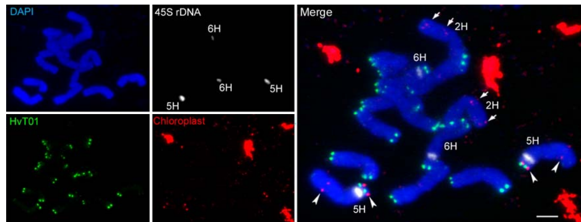
Figure 1: FISH mapping of chloroplast insertions into the nuclear genome of barley cv. Morex. Chloroplast DNA (red), subtelomeric satellite HvT01 (green) and 45S rDNA (white) were mapped on metaphase chromosomes. Chloroplast derived DNA insertions are detected on chromosome 2H (arrows) and 5H (arrowheads). Non-chromosomal chloroplast DNA signals represent plastids. Chromosomes were counterstained by DAPI. Scale bar = 5 \mu m.
