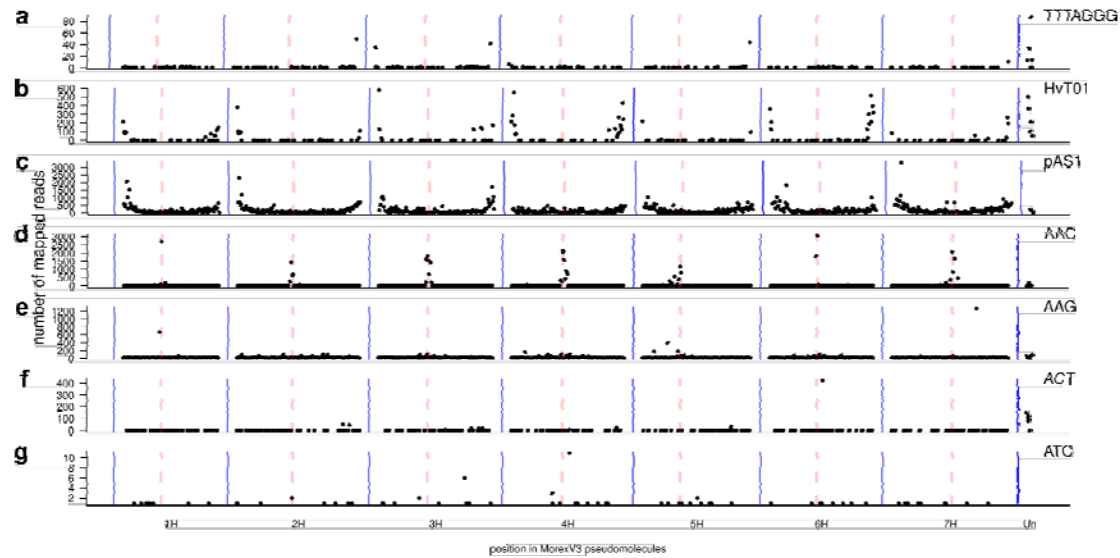
Figure 3: Locations of known satellite arrays in the MorexV3 pseudomolecules. Known repeat sequences were annotated in read sequences. Telomeric repeats (TTTAGGG, (a)) and trinucleotide microsatellites (d-g) were identified with Tandem Repeat Finder in ONT reads; subtelomeric repeats [HvT01 (b) and pAS1 (c)] were found by BLAST against HiFi reads. The counts of reads containing these repeats and mapped uniquely to positions in the MorexV3 pseudomolecules were aggregated in 5 Mb windows and plotted along the genome. Dashed red lines mark centromeres.
