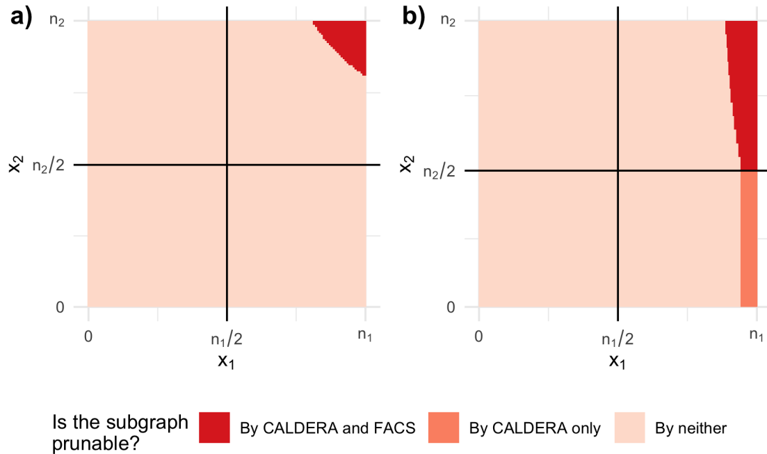
Figure S3: We consider the space of all possible patterns for n = 280 , J = 2 and two cases: a) n_1 = n_2 = 140 and b) n_1 = 260 = 13 \times n_2 . The phenotypes are well balanced in each population and \alpha = 10^{-8} . The extended lower bound increases the number of prunable subgraphs when the populations are imbalanced.
