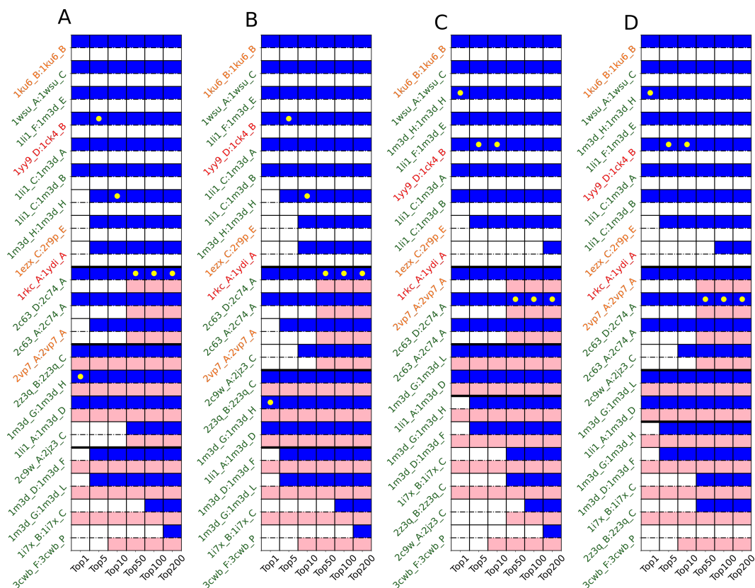
Figure S4: Ranking results per protein pair. A , DLA-Ranker trained and validated on core and rim residues only (DLA-Ranker-CR), B , DLA-Ranker-CR combined with CIPS, C , DLA-Ranker trained and validated on support and core residues only (DLA-Ranker-SC), D , DLA-Ranker-SC combined with CIPS. The color codes are the same as in Fig. 1.
