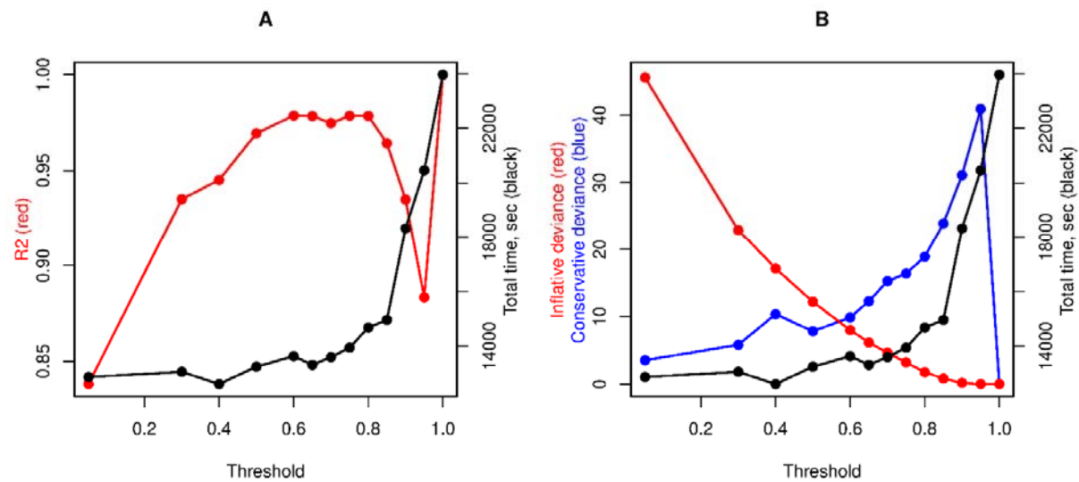
Figure 2. Determination coefficient and deviances of approximated SKAT statistic related to the threshold value. (A) Determination coefficient ( R^2 ) between -\log_{10}(\text{P value}) of original and approximated tests shown in red. (B) Deviances indicating inflation and conservativeness of approximated test statistics compared with original shown in red and blue, respectively.
