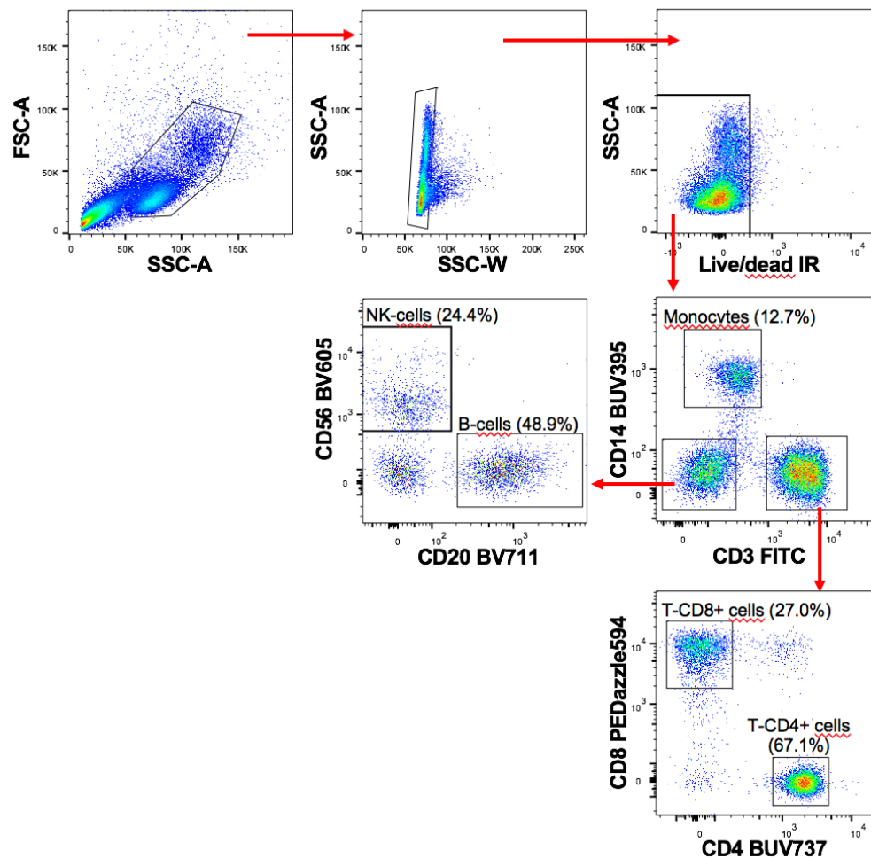
Fig.S5: Gating strategy for immune cell sorting. Gating strategy used to sort monocytes (CD14+), B (CD14-, CD3-, CD56-, CD20+), NK (CD14-, CD3-, CD20-, CD56+), T-CD4+ (CD14-, CD3+, CD8-, CD4+) and T-CD8+ cells (CD14-, CD3+, CD4-, CD8+) from freshly isolated PBMCs from 2 monozygotic twins exhibiting skewed XCI in LCLs.
