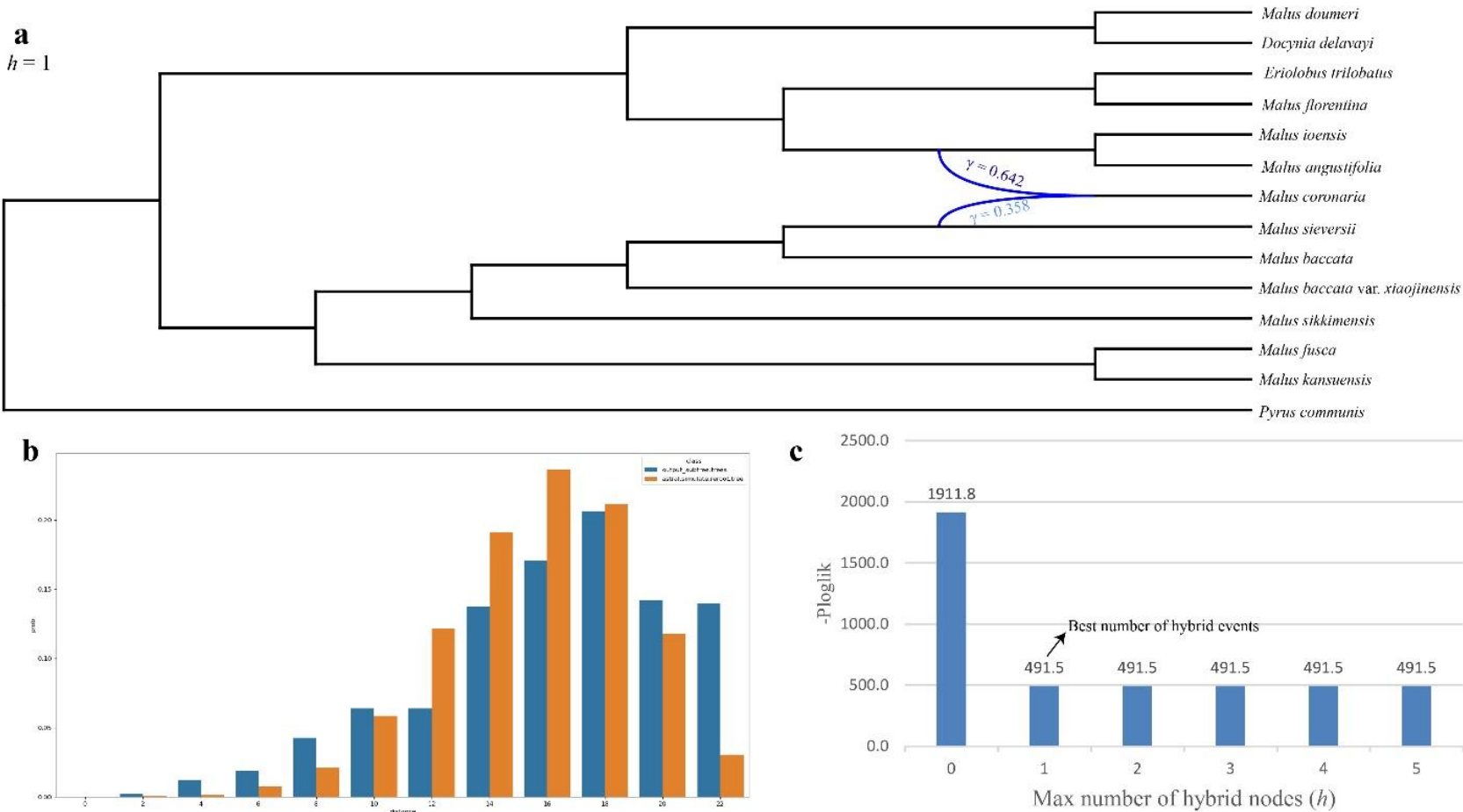
Fig. 5. Coalescent simulation and phylogenetic network analysis from the 14-taxa sampling at the genus level of Malus . a , Species networks inferred from SNaQ network analysis with hmax = 1 as the optimal network. b , Distribution of tree-to-tree distances between empirical gene trees and the ASTRAL species tree, compared to those from the coalescent simulation. c , The pseudo-loglikelihood scores (-ploglik) of one to five maximum number of reticulations. Blue curved branches indicate the possible hybridization event. Dark blue and light blue numbers indicate the major and minor inheritance probabilities of hybrid nodes.
