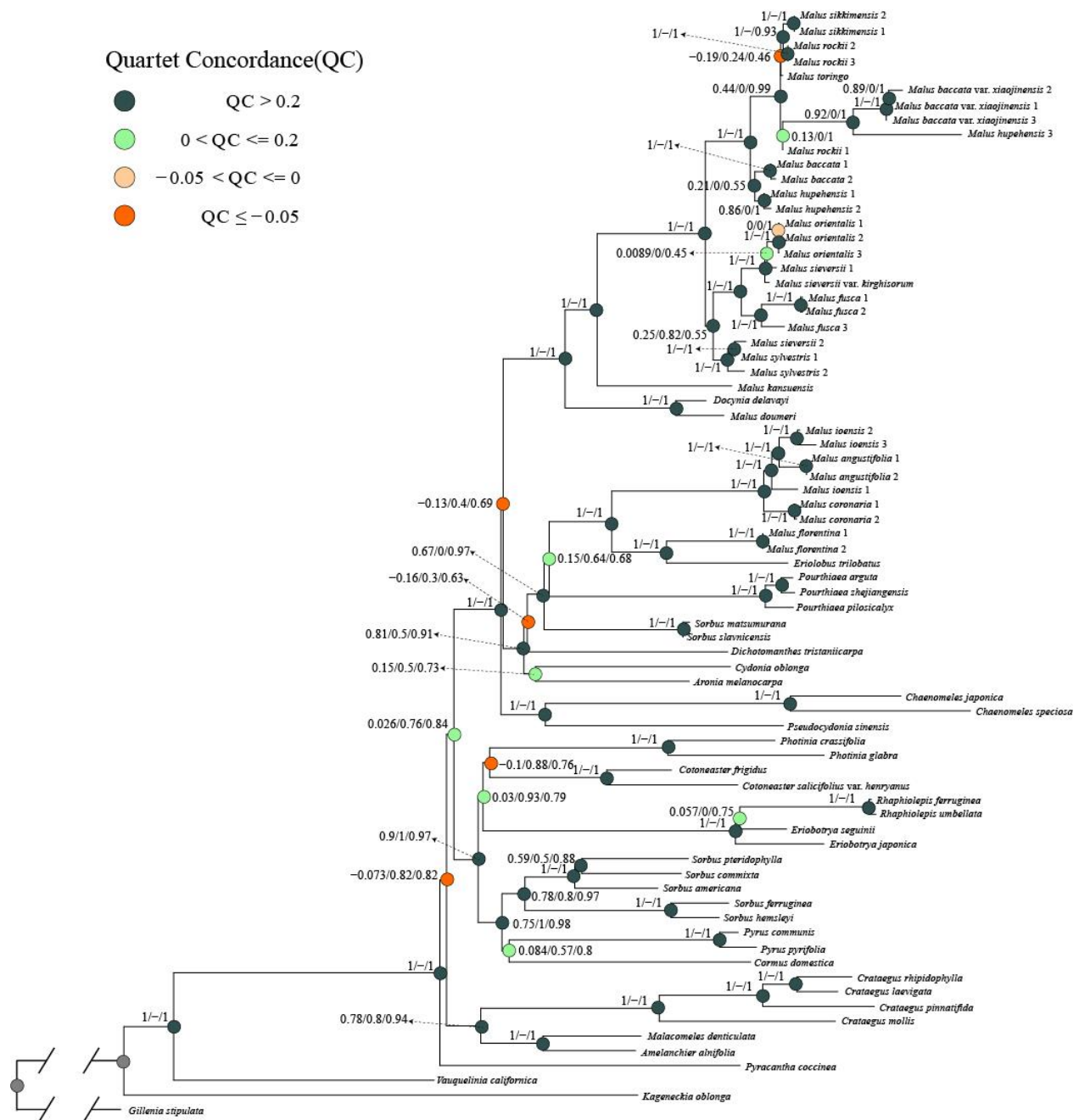
Fig. S15. Maximum likelihood phylogeny of Malus s.l. in the framework of Maleae inferred from RAxML analysis of the concatenated 80 plastid coding genes. Quartet Sampling Scores are shown on branches indicating Quartet Concordance/Quartet Differential/Quartet Informativeness. Quartet Concordance is color-coded according to the legend.
