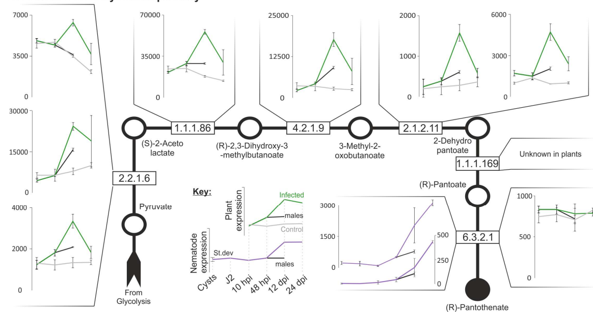
Figure S6. The complete vitamin B5 biosynthesis pathway. Black arrow indicates the linear pathway of vitamin B5 biosynthesis. Products/substrates are indicated with circles, enzymatic reactions (and corresponding EC codes) with squares. For each species, the expression profiles of the gene/s annotated with the EC codes at each step are shown (green for host, purple for parasite), if present. All steps are absent in the parasite H. schachtii , and present and upregulated at 14 dpi in the host A. thaliana , with the exception of the last step (PANC). PANC in the host is not upregulated at any time of infection, whereas PANC present in the parasite is upregulated during infection.
